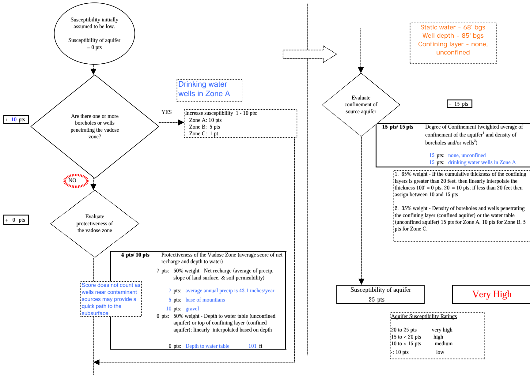
Chart 2. Susceptibility of the aquifer - Bird Creek Campground (211261.001)
