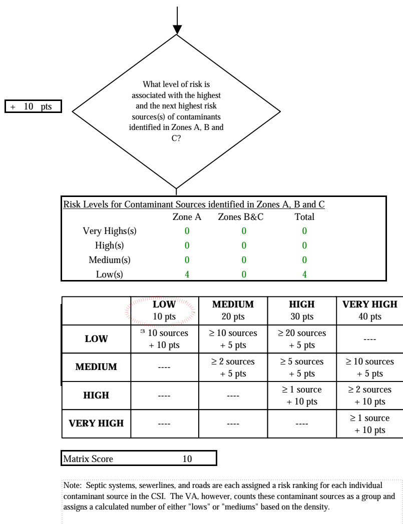
Chart 7. Contaminant risks for Bird Creek Campground (211261.001) - Volatile Organic Chemicals
