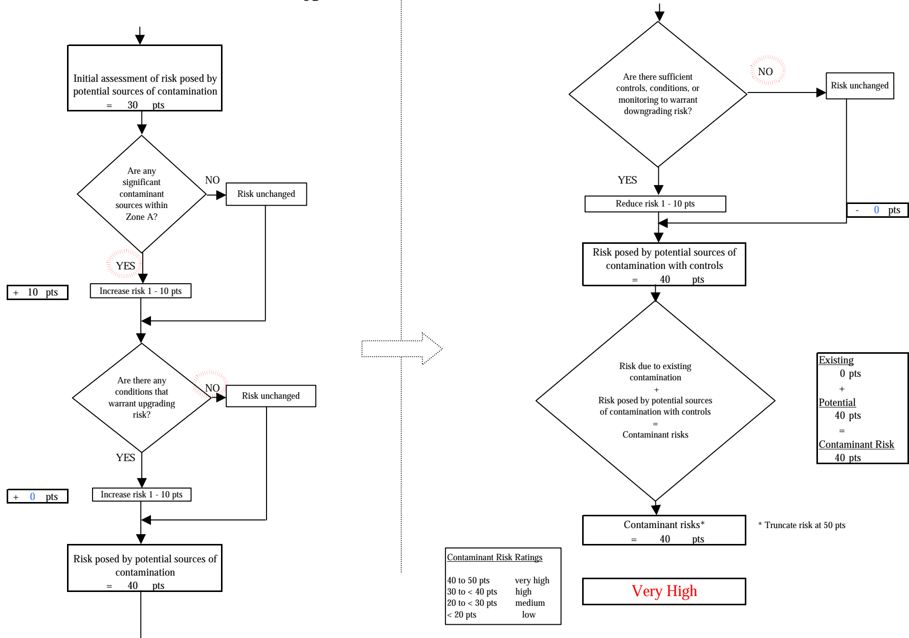
Chart 3. Contaminant risks for Bird Creek Campground (211261.001) - Bacteria & Viruses
