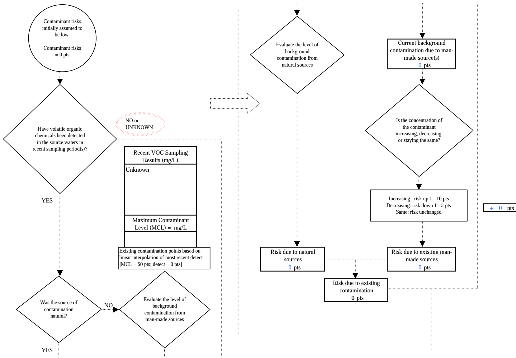
Chart 7. Contaminant risks for Bird Creek Campground (211261.001) - Volatile Organic Chemicals
