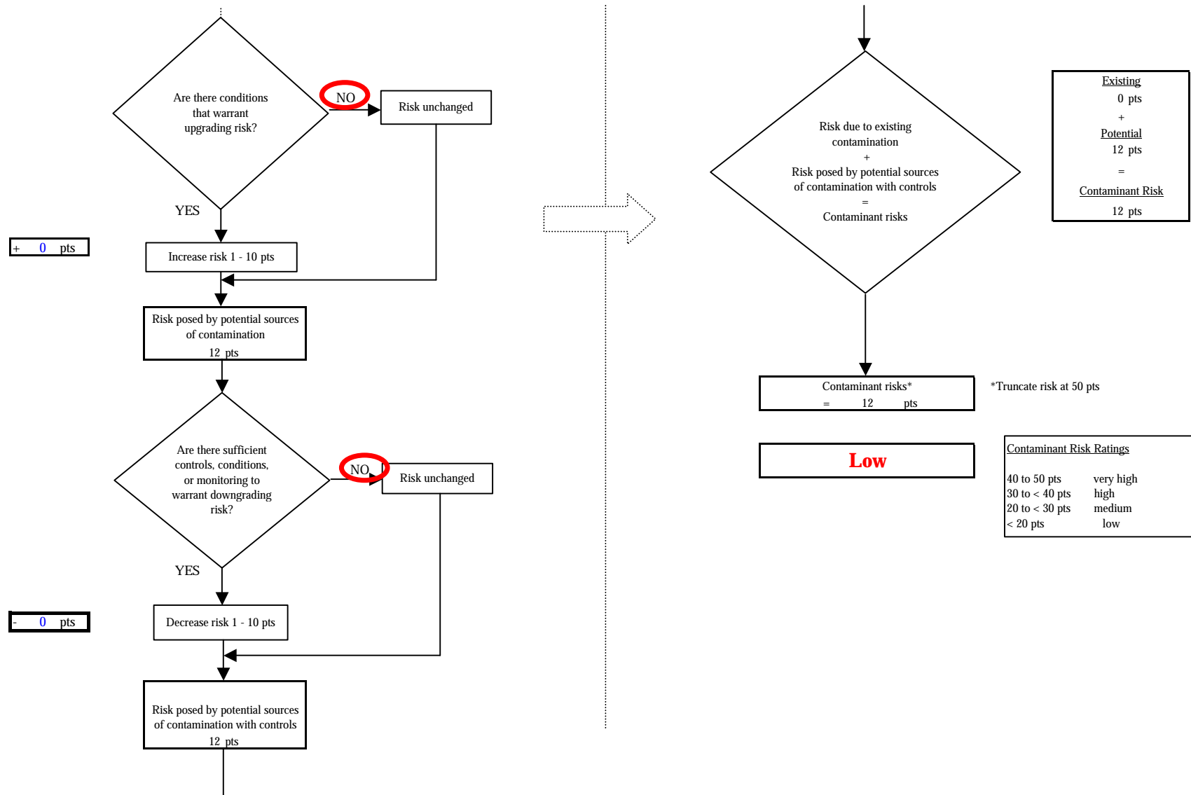
Chart 7. Contaminant risks for Bird Creek Campground (211261.001) - Volatile Organic Chemicals
