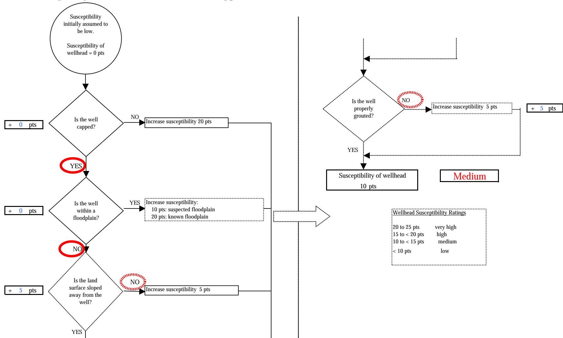
Chart 1. Susceptibility of the wellhead - Bird Creek Campground (211261.001)
