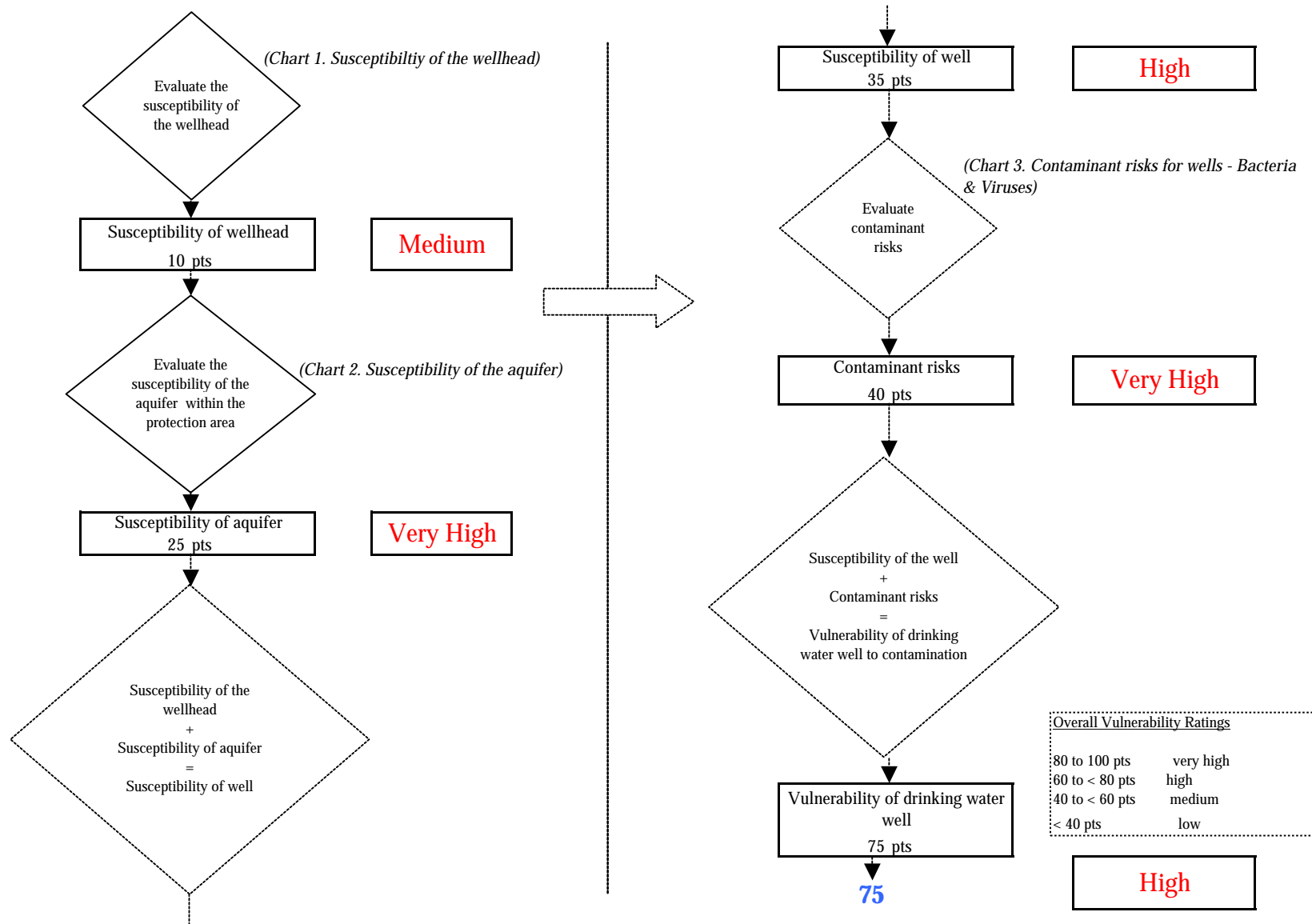
Chart 4. Vulnerability analysis for Bird Creek Campground (211261.001) - Bacteria & Viruses
