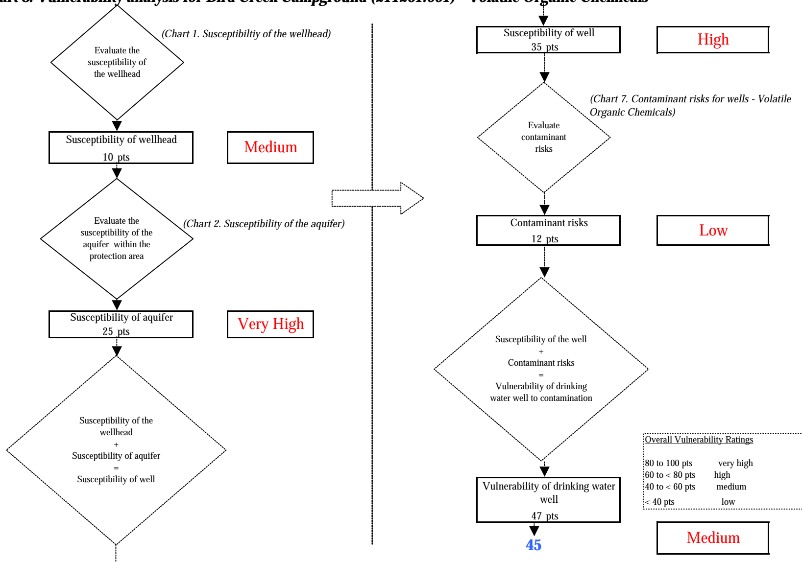
Chart 8. Vulnerability analysis for Bird Creek Campground (211261.001) - Volatile Organic Chemicals
