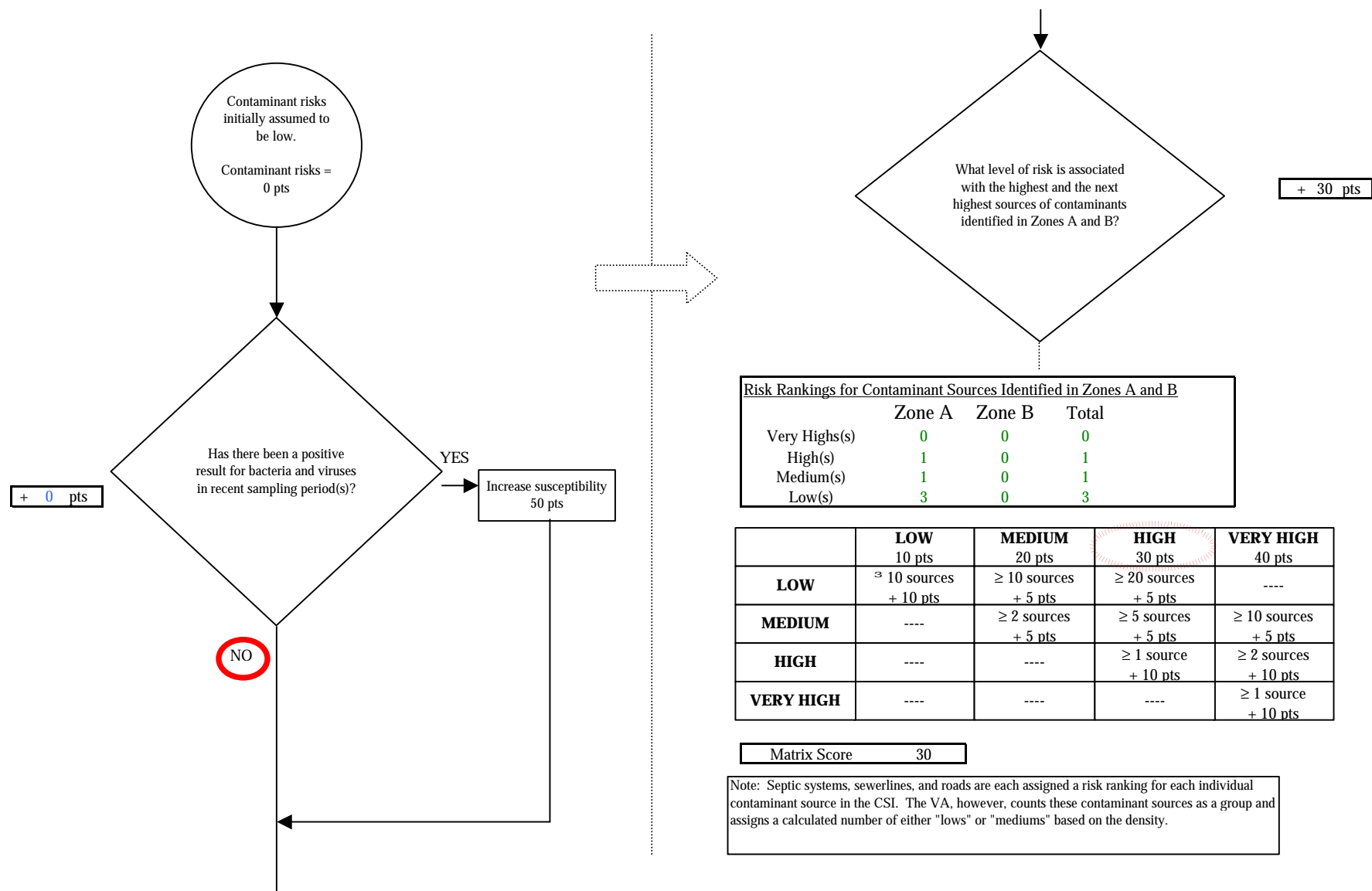
Chart 3. Contaminant risks for Bird Creek Campground (211261.001) - Bacteria & Viruses
