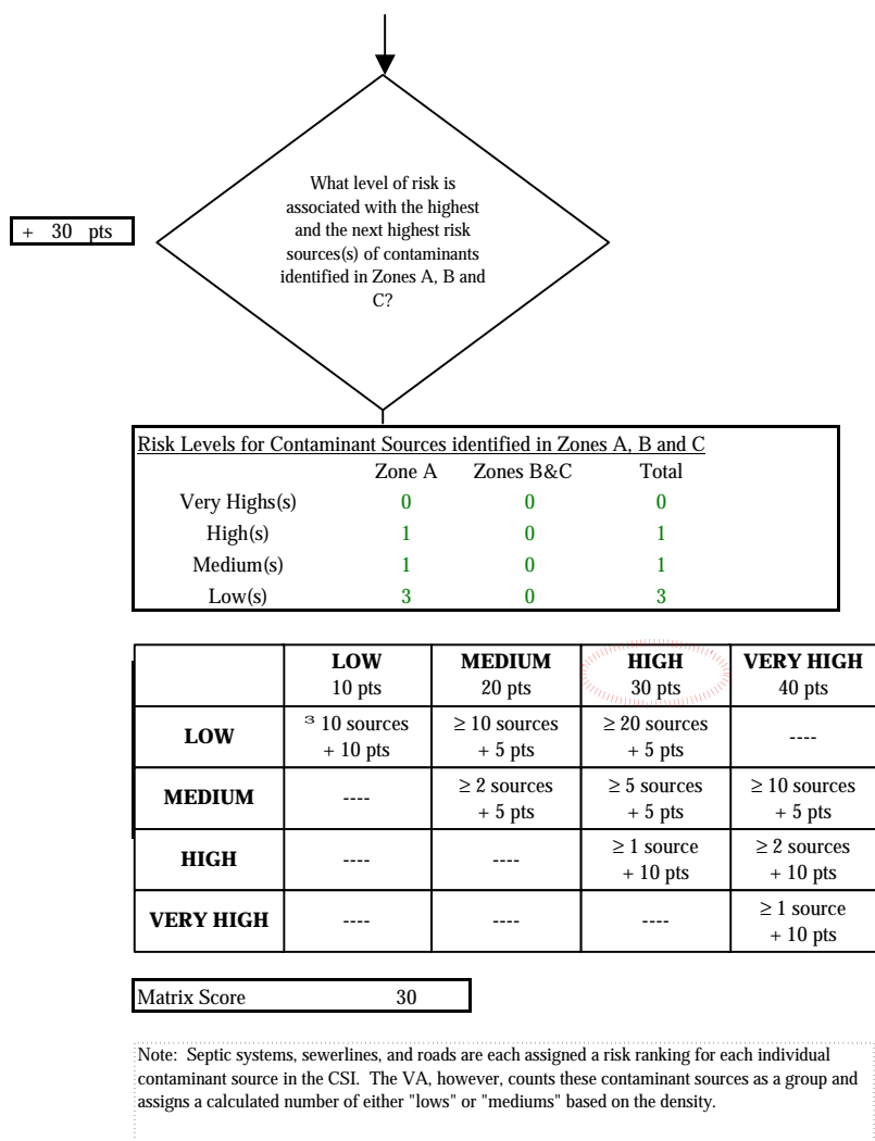
Chart 5. Contaminant risks for Bird Creek Campground (211261.001) - Nitrates and Nitrites
