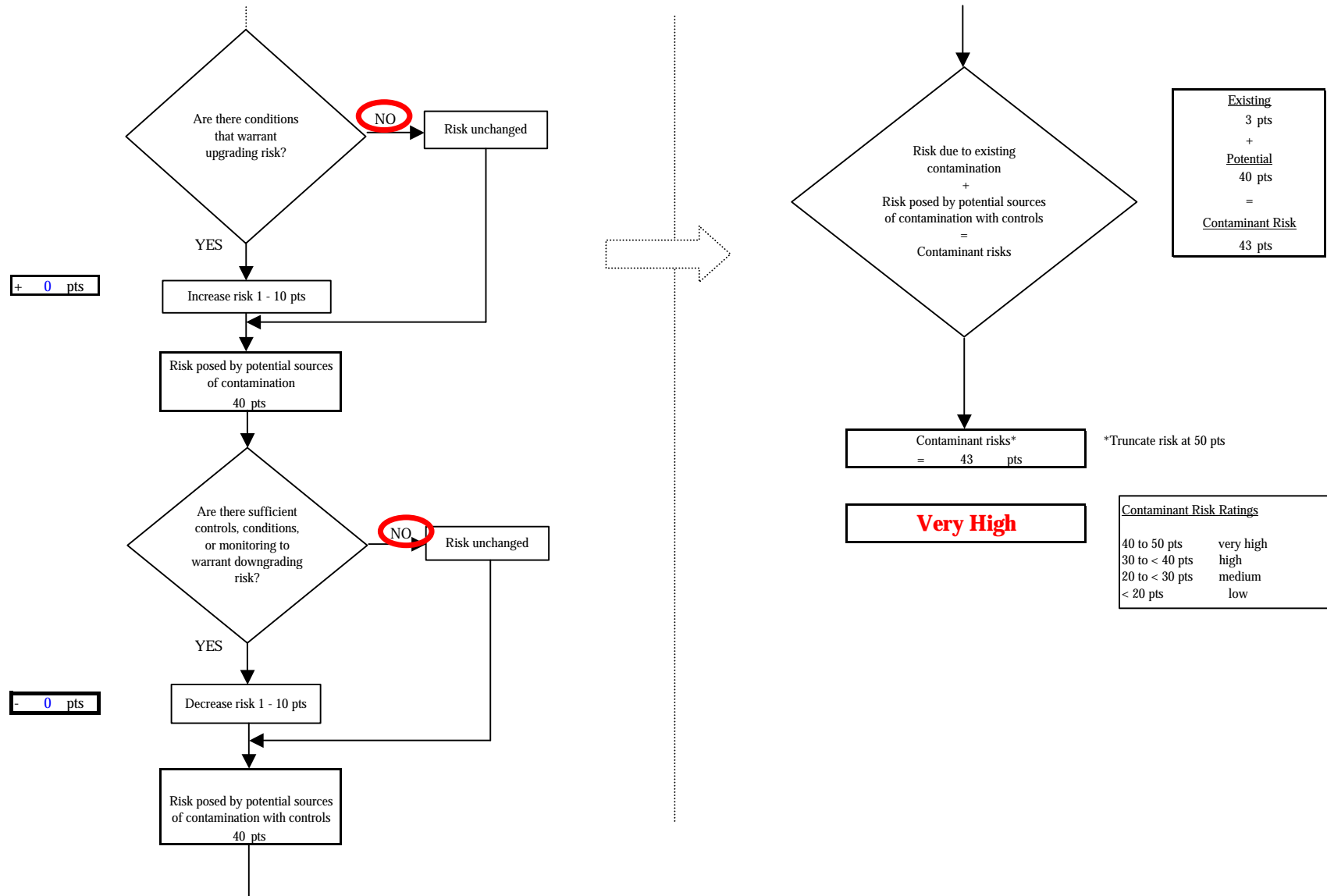
Chart 5. Contaminant risks for Bird Creek Campground (211261.001) - Nitrates and Nitrites
