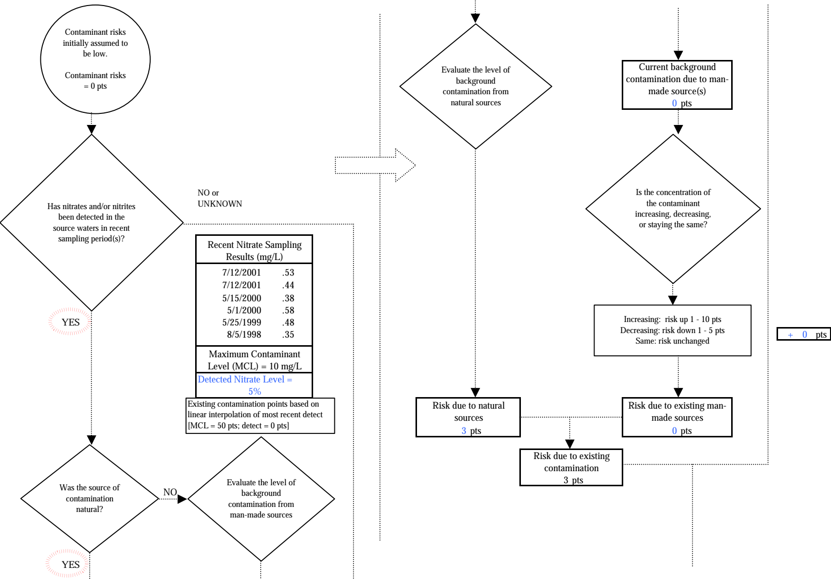
Chart 5. Contaminant risks for Bird Creek Campground (211261.001) - Nitrates and Nitrites
