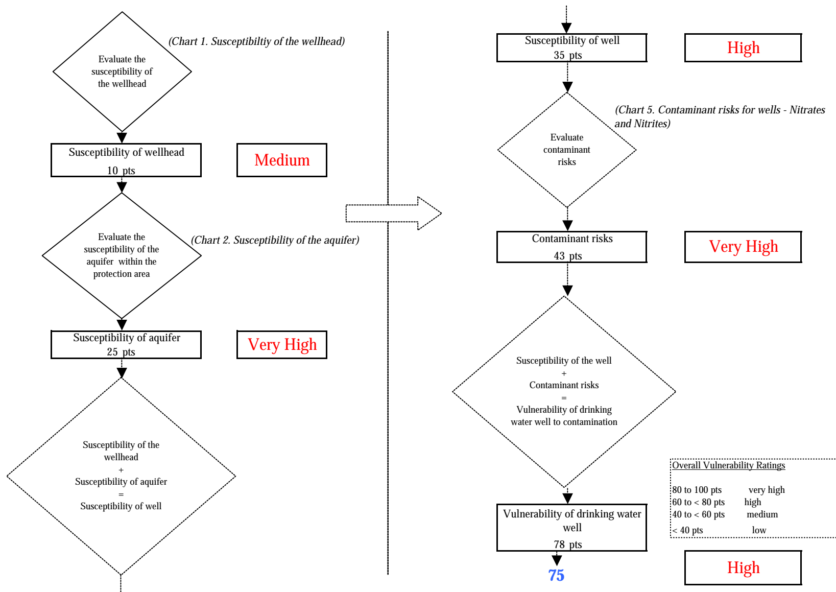
Chart 6. Vulnerability analysis for Bird Creek Campground (211261.001) - Nitrates and Nitrites
