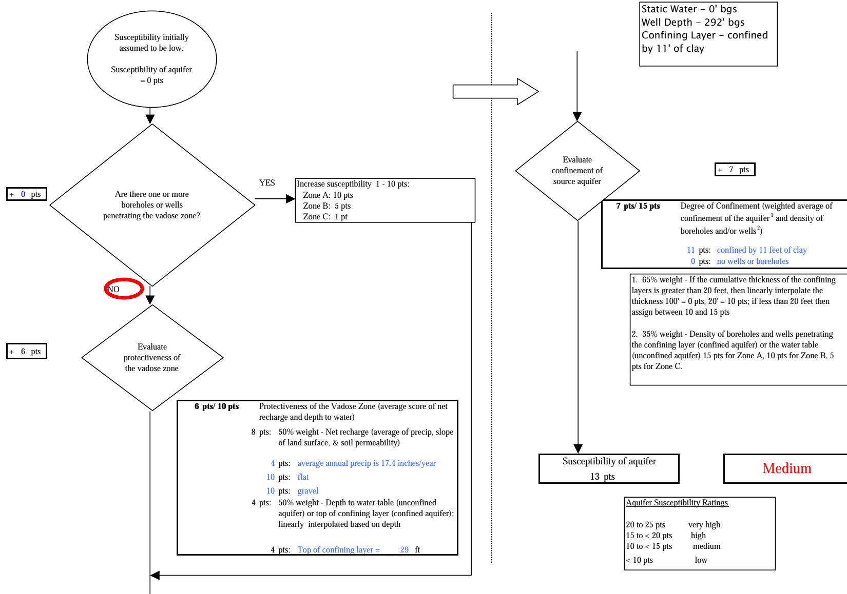
Chart 2. Susceptibility of the aquifer - City of Soldotna Airport (240935.001)
