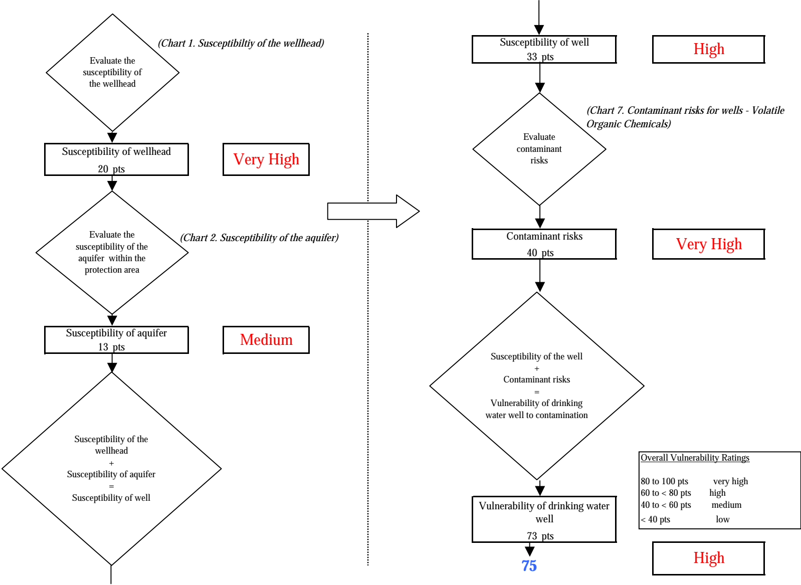
Chart 8. Vulnerability analysis for City of Soldotna Airport (240935.001) - Volatile Organic Chemicals
