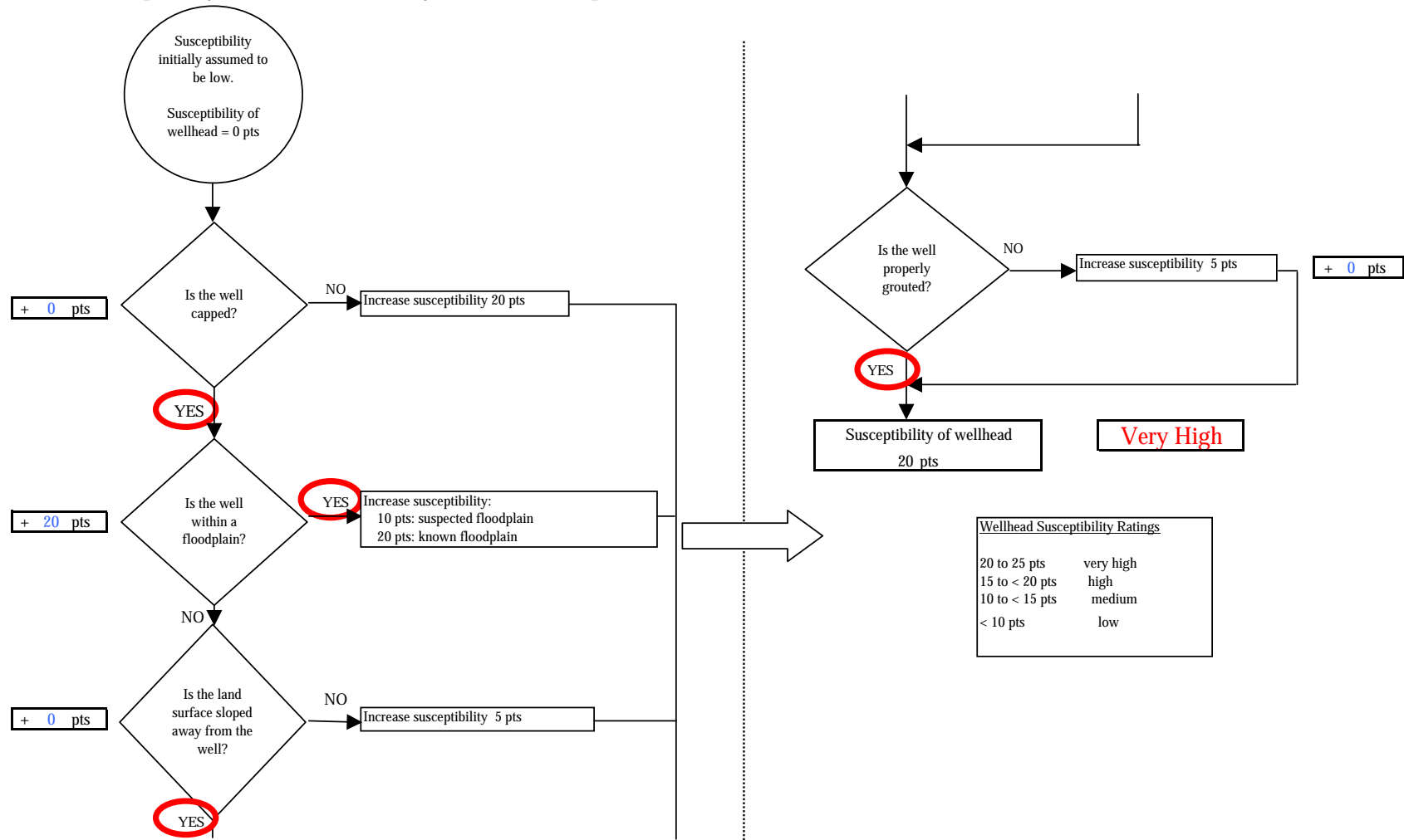
Chart 1. Susceptibility of the wellhead - City of Soldotna Airport (240935.001)
