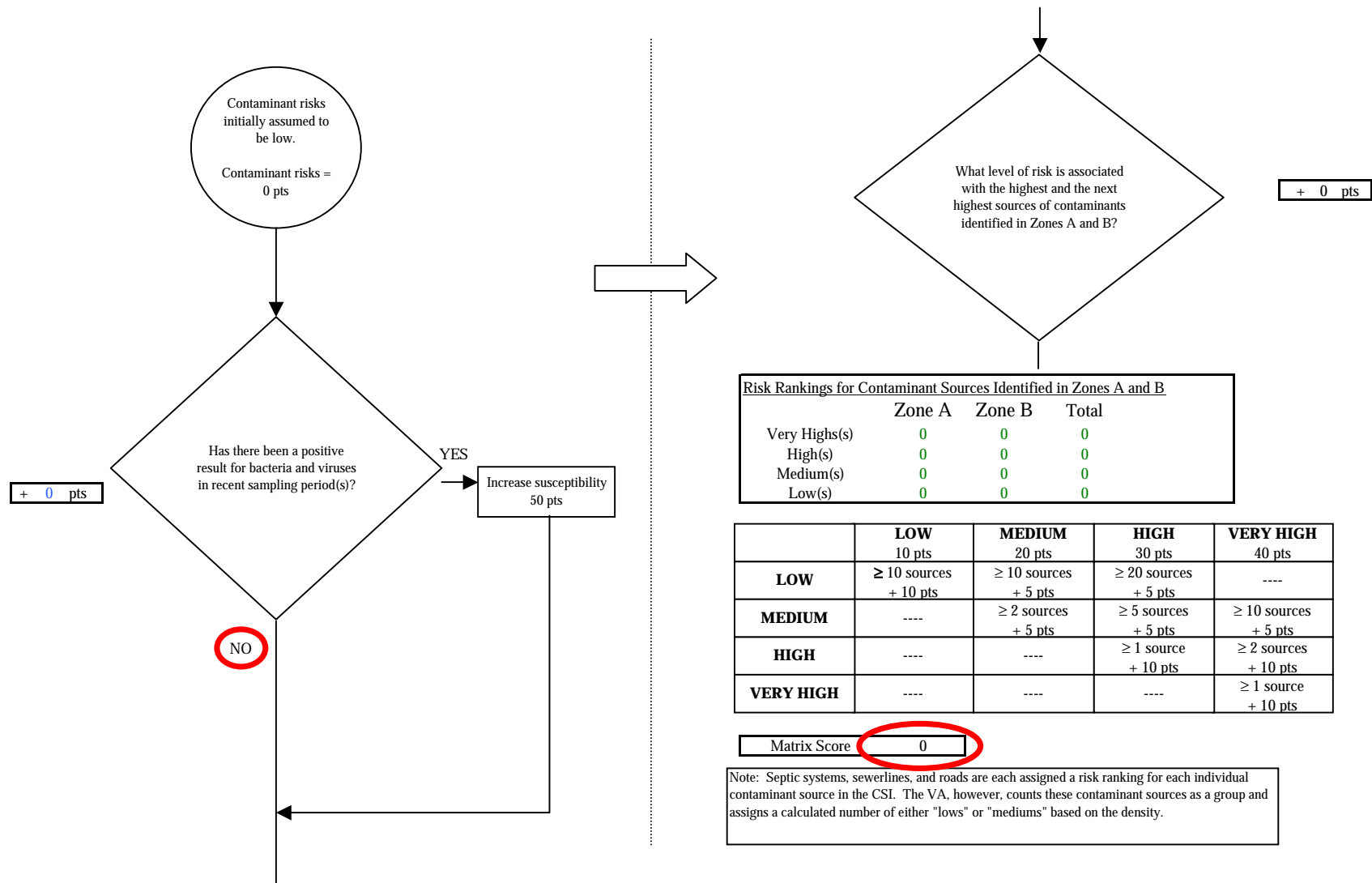
Chart 3. Contaminant risks for City of Soldotna Airport (240935.001) - Bacteria & Viruses
