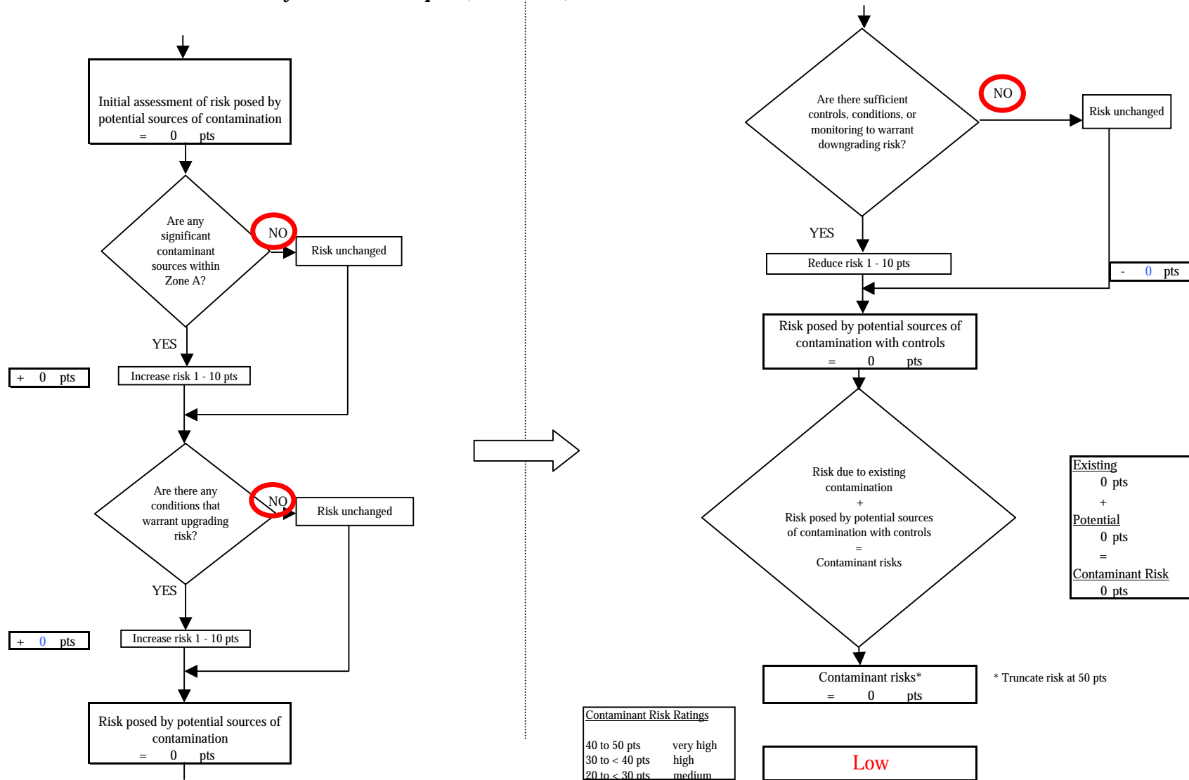
Chart 3. Contaminant risks for City of Soldotna Airport (240935.001) - Bacteria & Viruses
