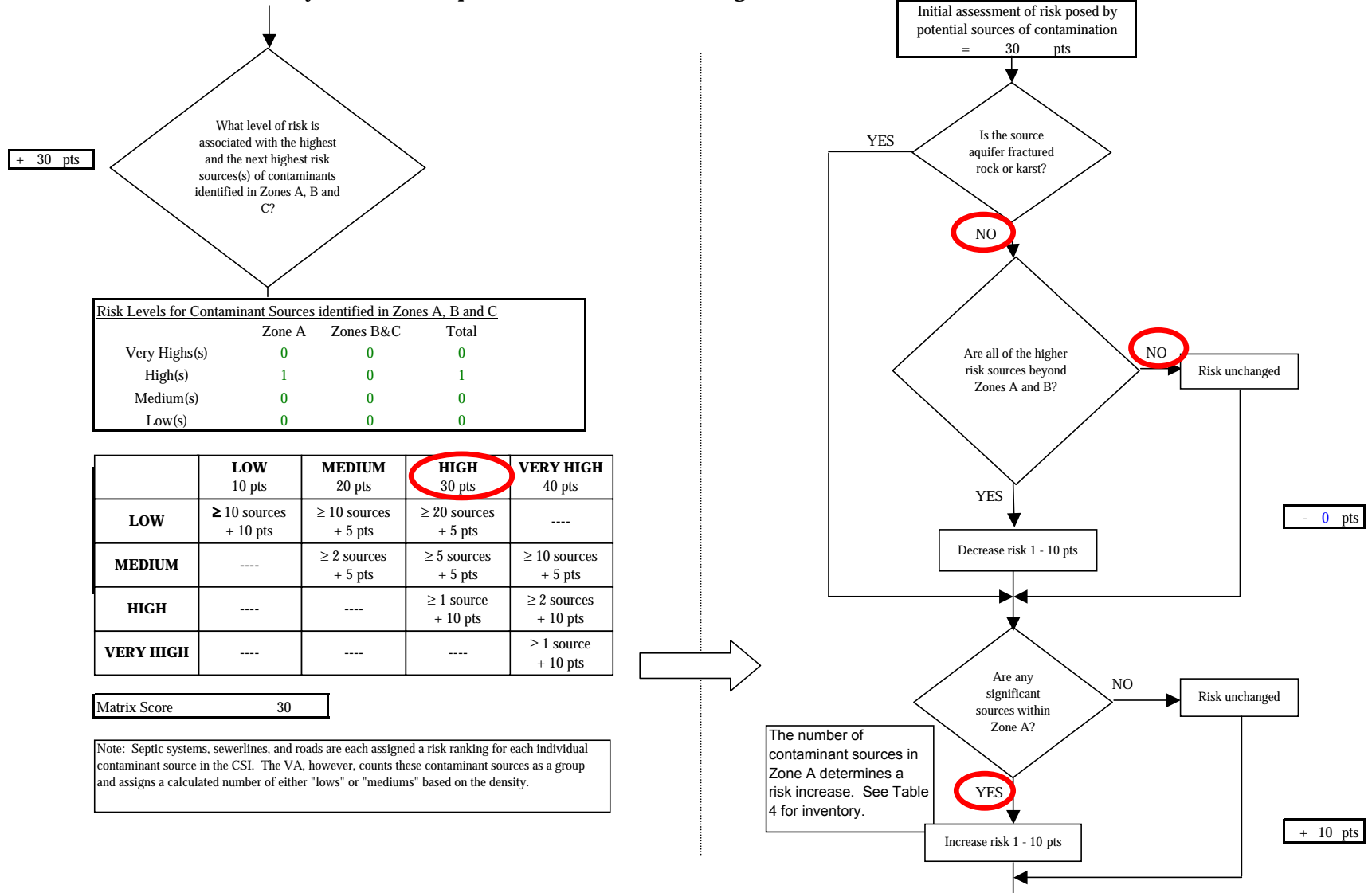
Chart 7. Contaminant risks for City of Soldotna Airport (240935.001) - Volatile Organic Chemicals
