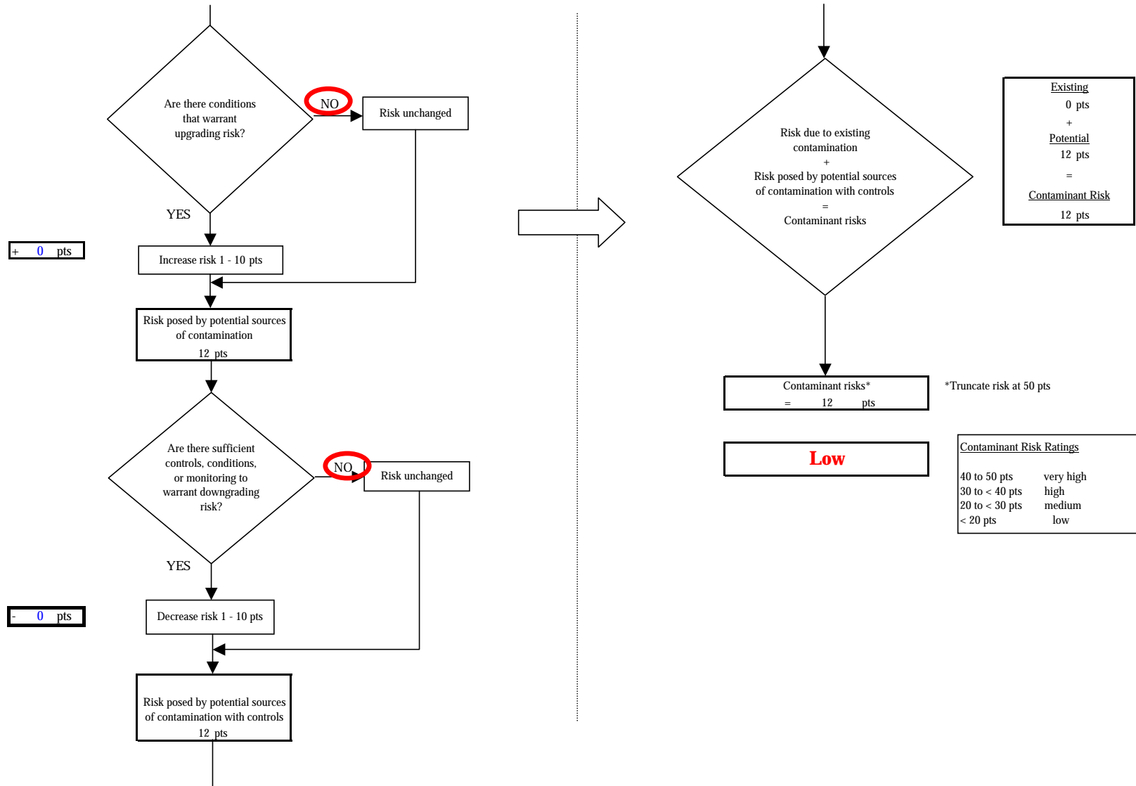
Chart 5. Contaminant risks for City of Soldotna Airport (240935.001) - Nitrates and Nitrites
