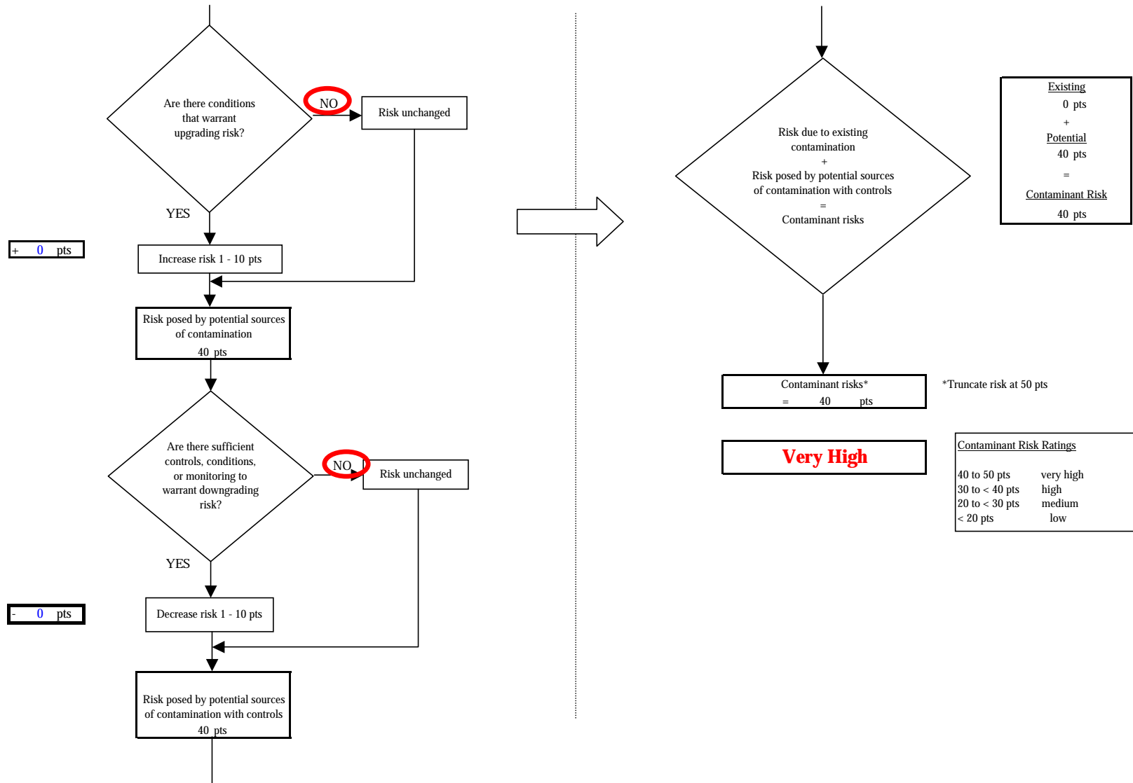
Chart 7. Contaminant risks for City of Soldotna Airport (240935.001) - Volatile Organic Chemicals
