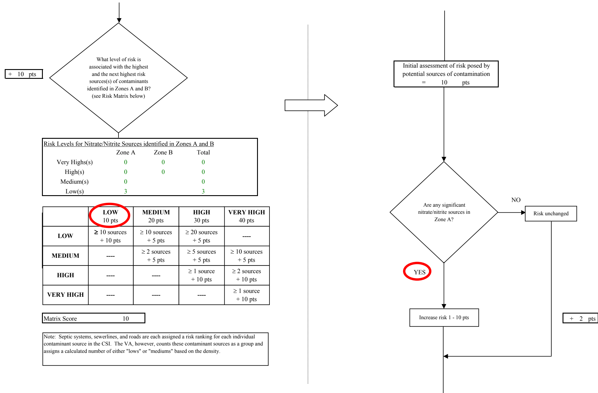
Chart 4. Contaminant risks for Port Graham - Nitrates and Nitrites
