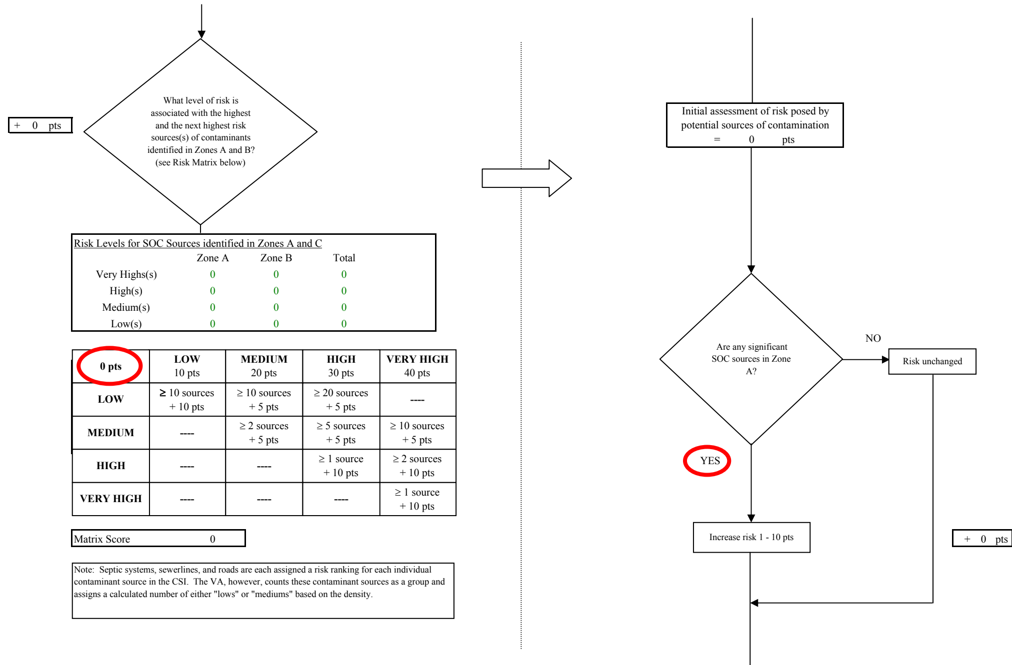
Chart 10. Contaminant risks for Port Graham - Synthetic Organic Chemicals
