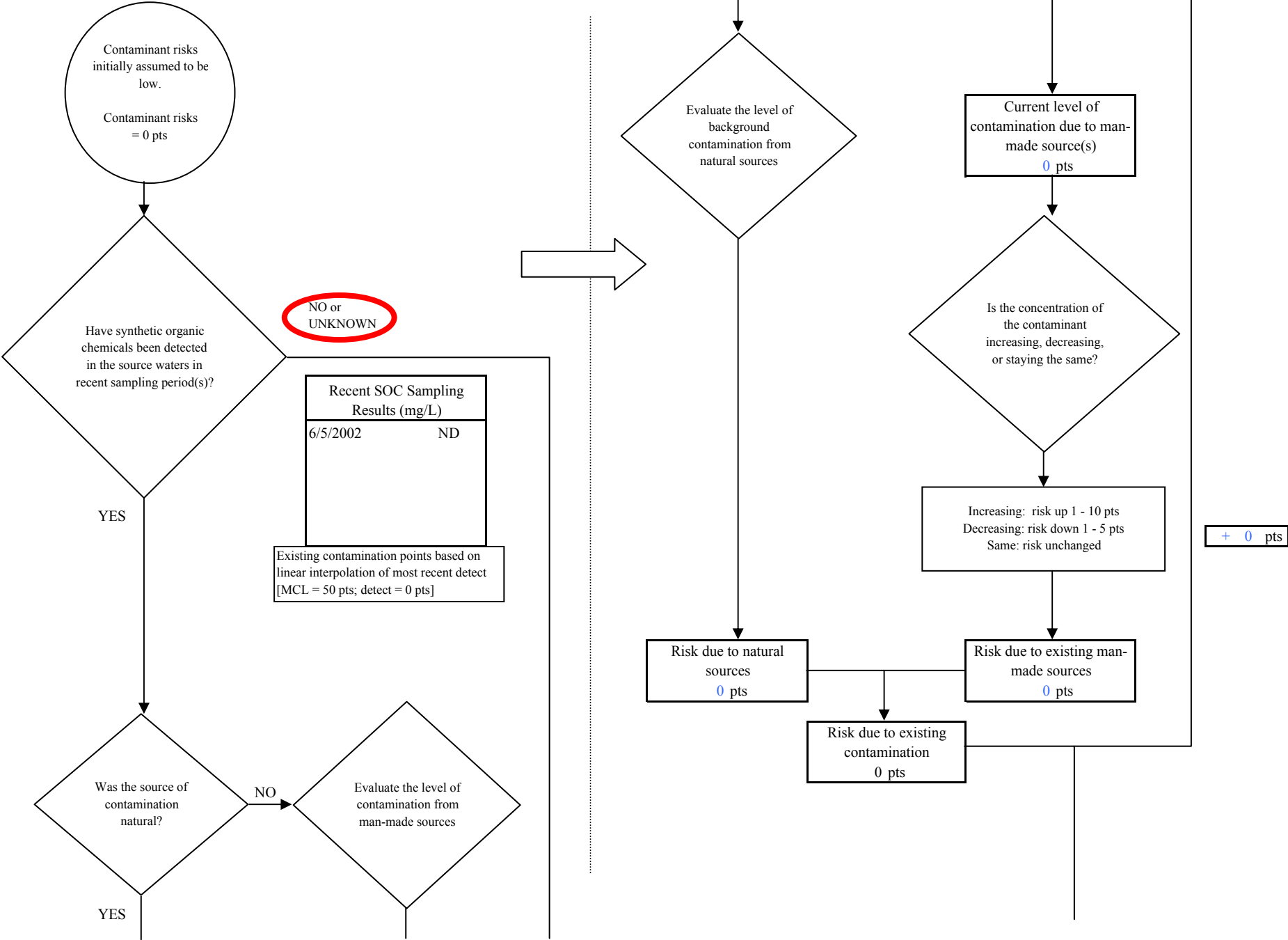
Chart 10. Contaminant risks for Port Graham - Synthetic Organic Chemicals
