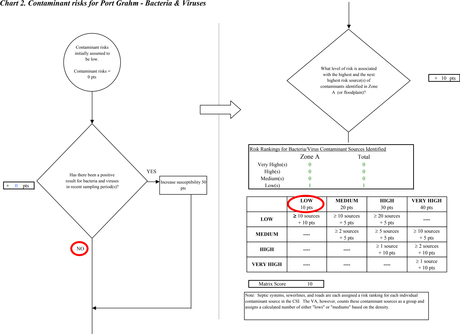
Chart 2. Contaminant risks for Port Graham - Bacteria & Viruses
