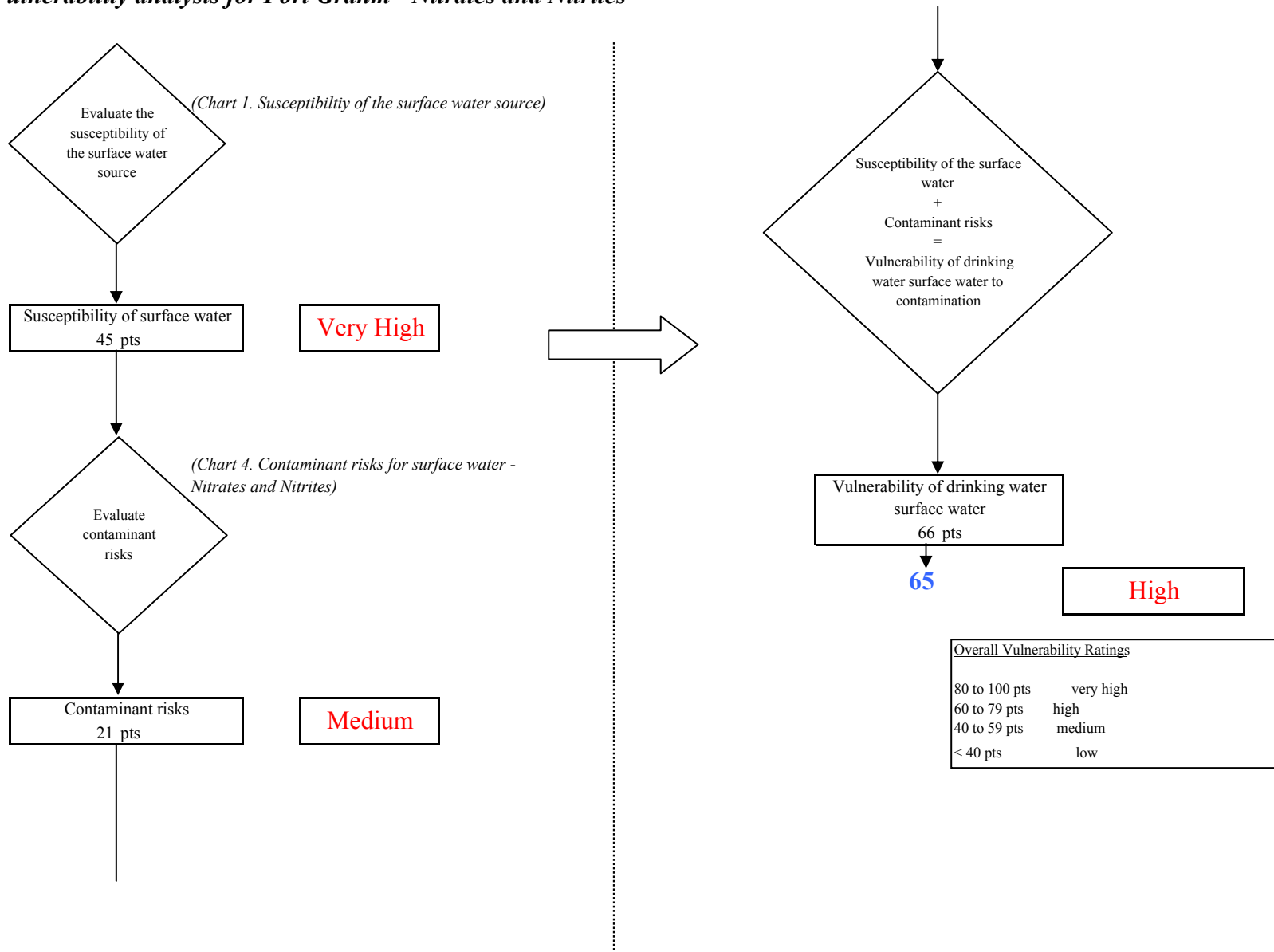
Chart 5. Vulnerability analysis for Port Graham - Nitrates and Nitrites
