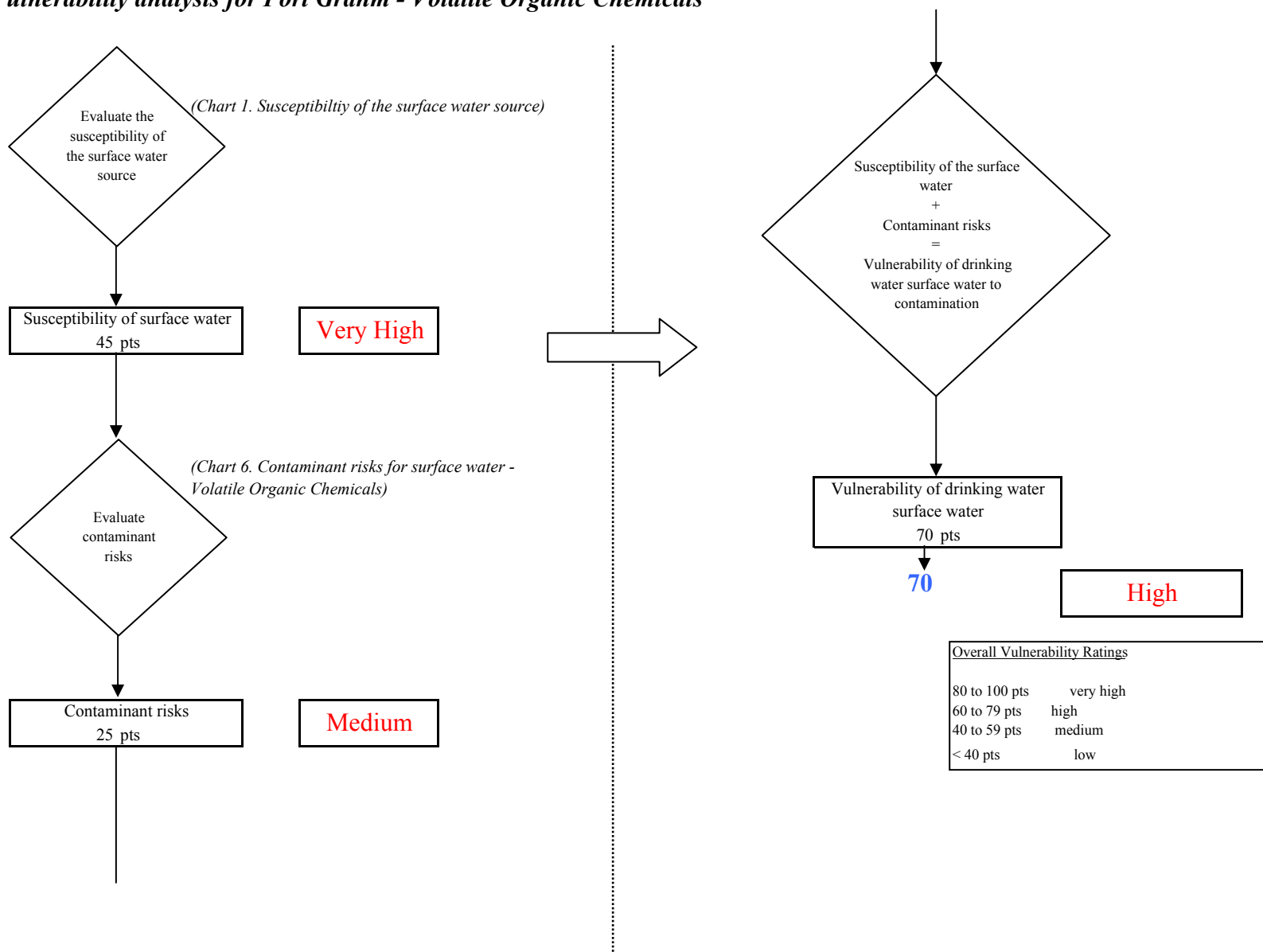
Chart 7. Vulnerability analysis for Port Graham - Volatile Organic Chemicals
