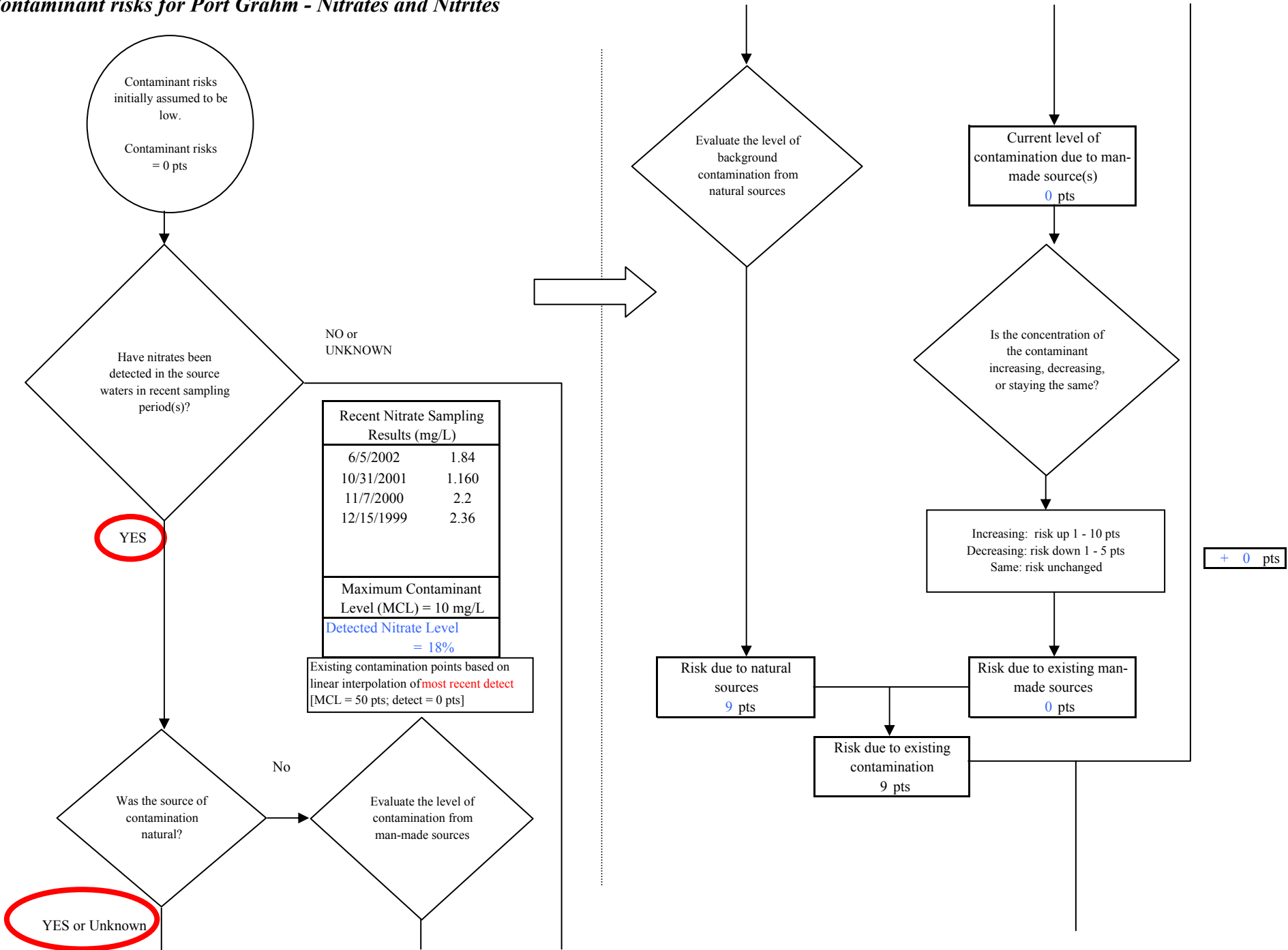
Chart 4. Contaminant risks for Port Graham - Nitrates and Nitrites
