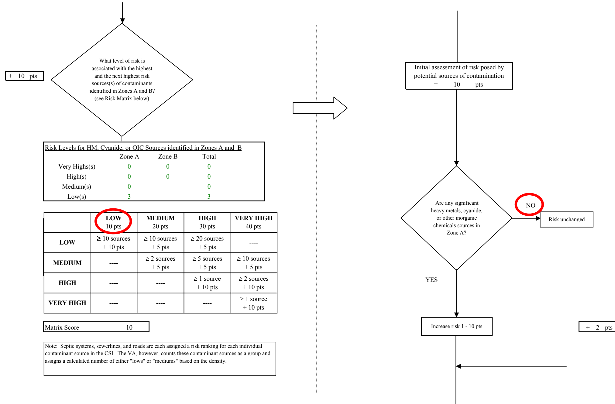
Chart 8. Contaminant risks for Port Graham - Heavy Metals, Cyanide and Other Inorganic Chemicals
