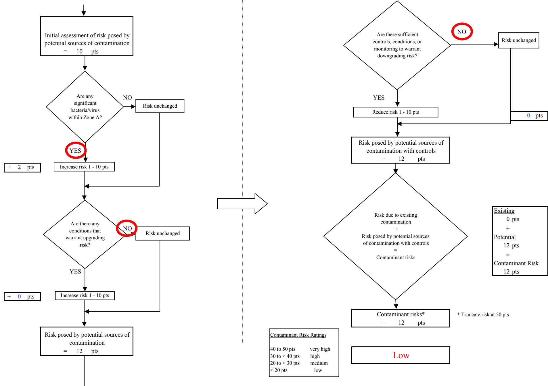
Chart 2. Contaminant risks for Port Graham - Bacteria & Viruses
