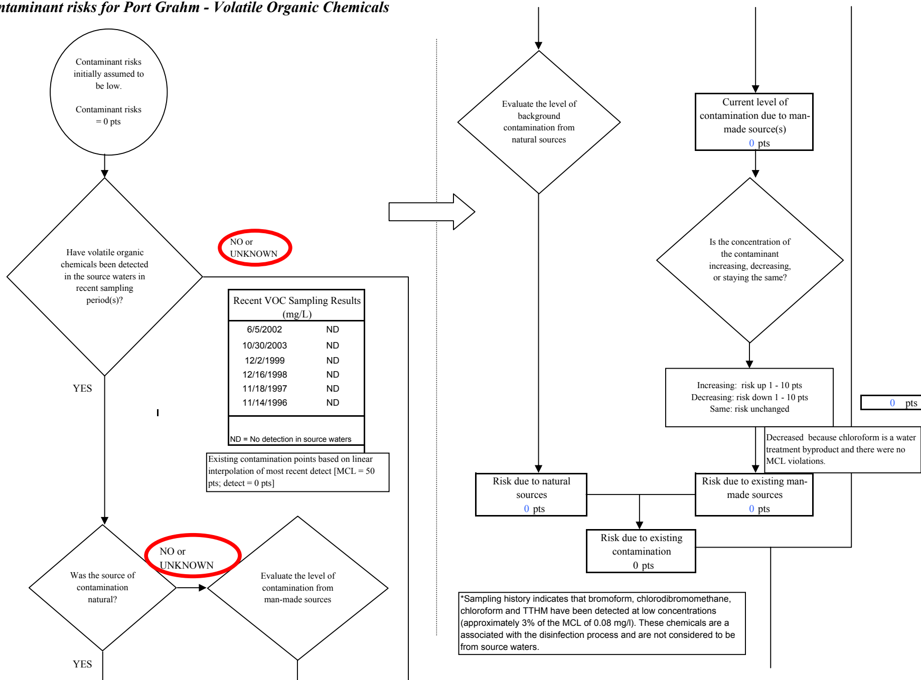
Chart 6. Contaminant risks for Port Graham - Volatile Organic Chemicals
