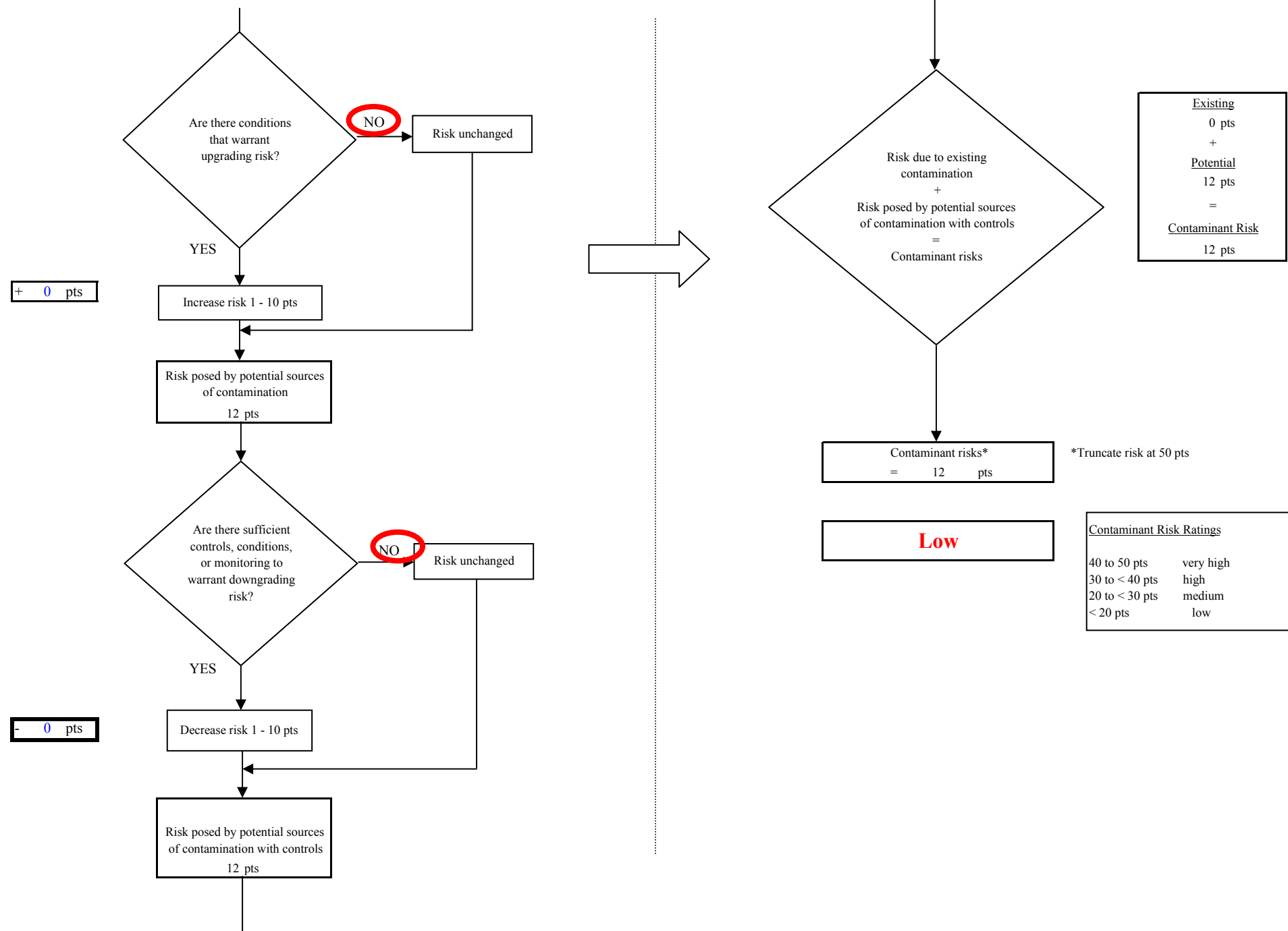
Chart 8. Contaminant risks for Port Graham - Heavy Metals, Cyanide and Other Inorganic Chemicals
