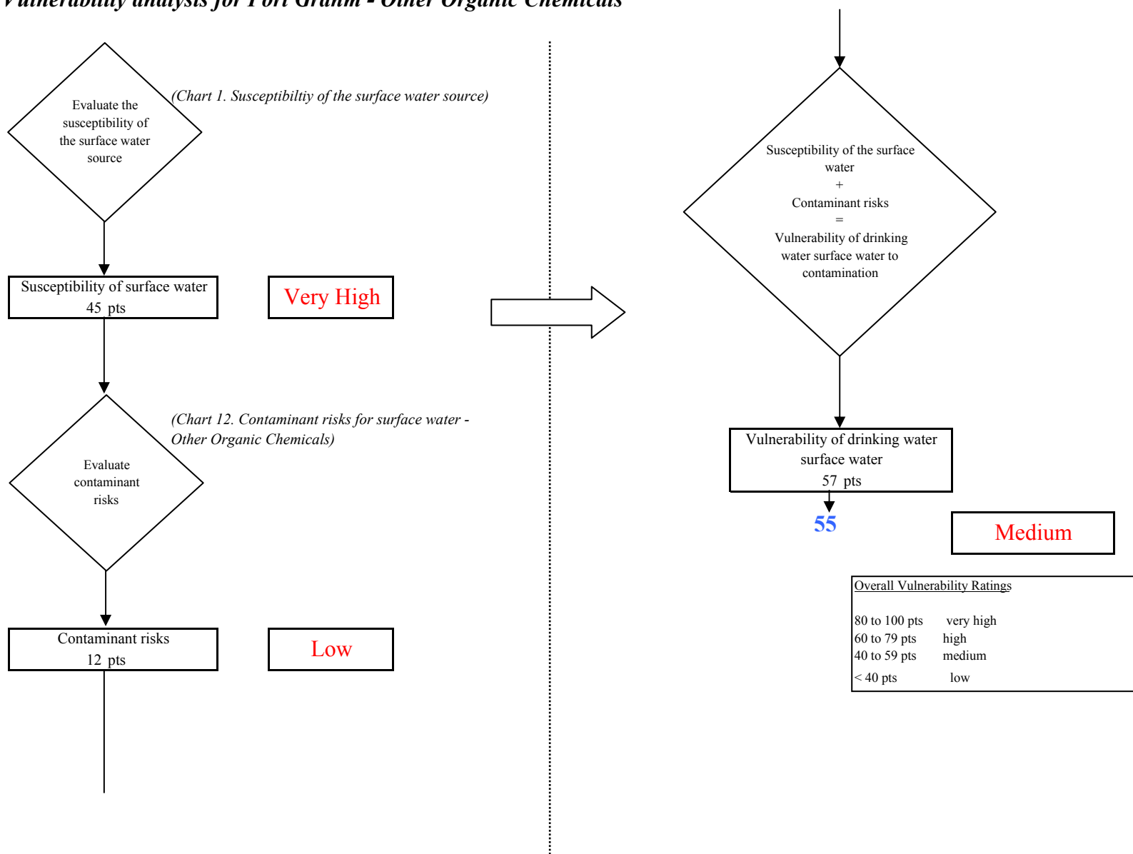
Chart 13. Vulnerability analysis for Port Graham - Other Organic Chemicals
