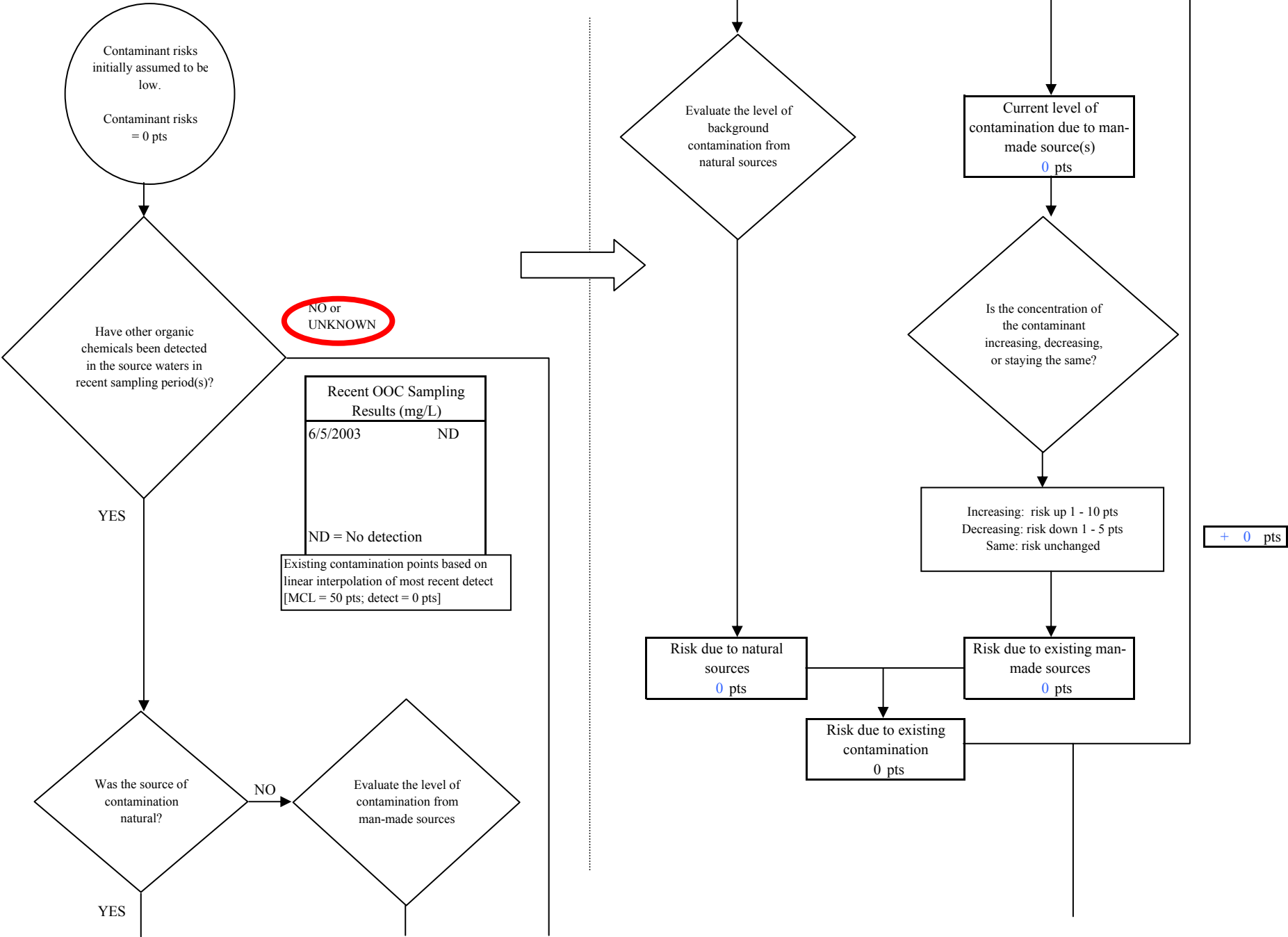
Chart 12. Contaminant risks for Port Graham - Other Organic Chemicals
