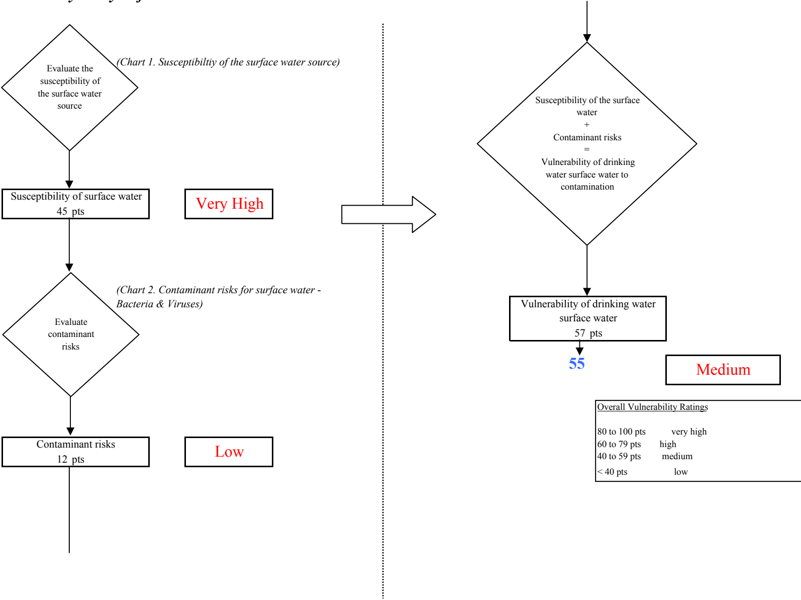
Chart 3. Vulnerability analysis for Port Graham - Bacteria & Viruses
