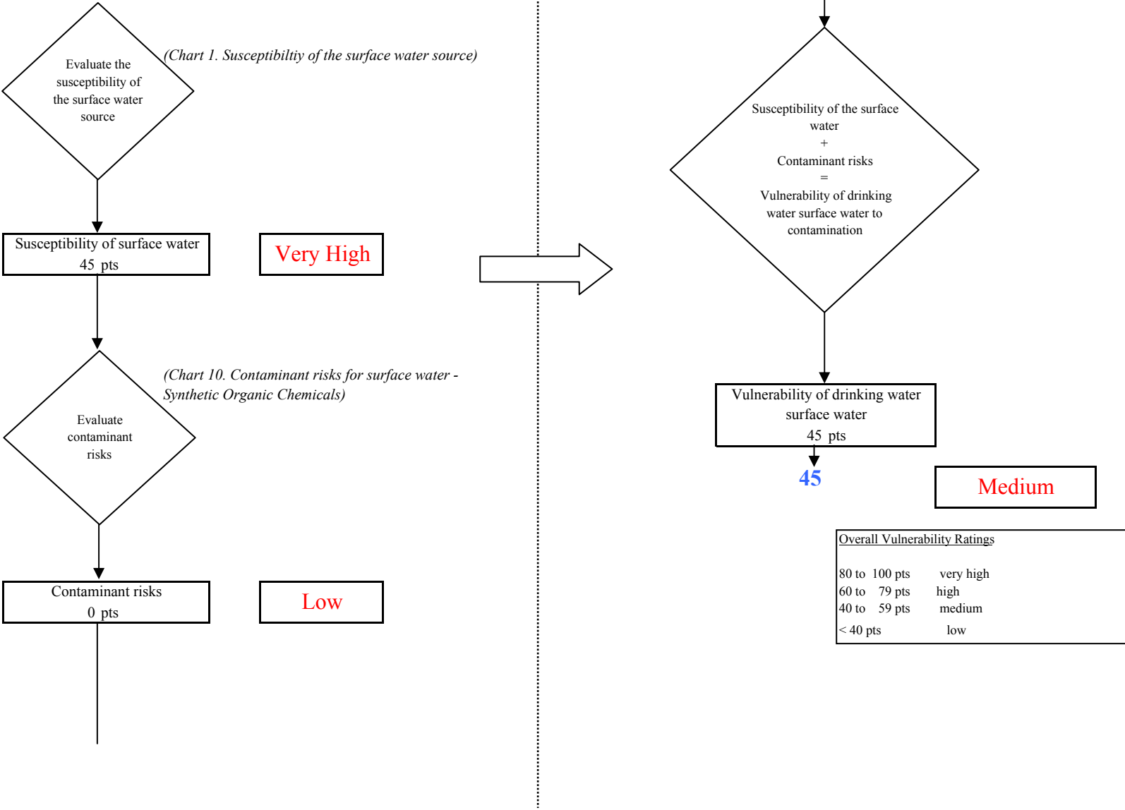
Chart 11. Vulnerability analysis for Port Graham - Synthetic Organic Chemicals
