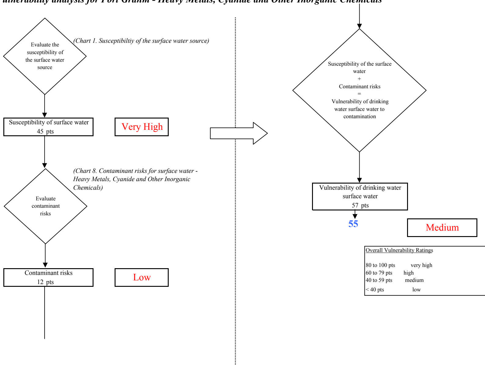
Chart 9. Vulnerability analysis for Port Graham - Heavy Metals, Cyanide and Other Inorganic Chemicals
