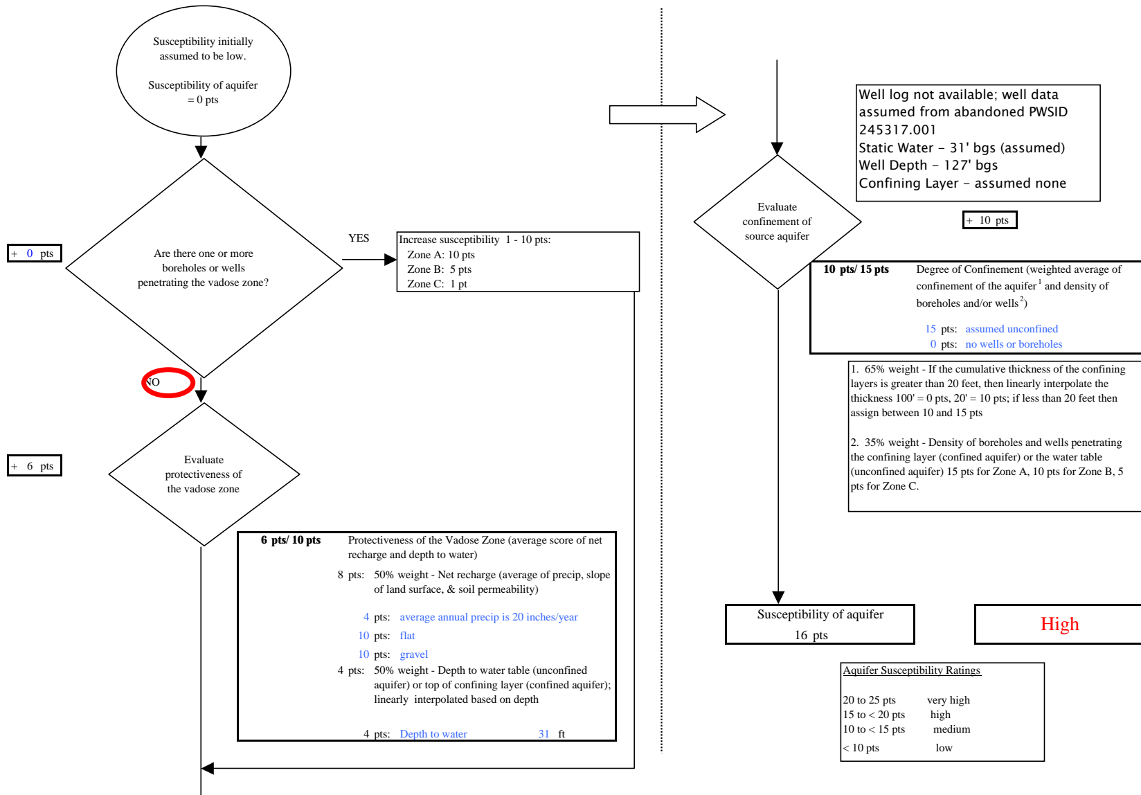
Chart 2. Susceptibility of the aquifer - Blue Grouse Inn (242220.001)
