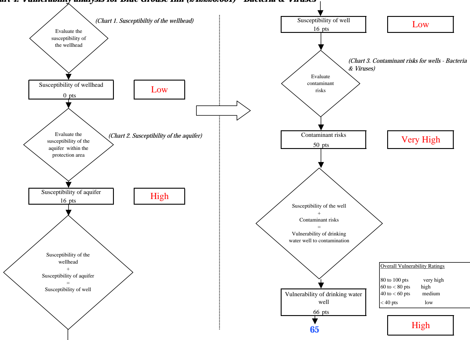
Chart 4. Vulnerability analysis for Blue Grouse Inn (242220.001) - Bacteria & Viruses
