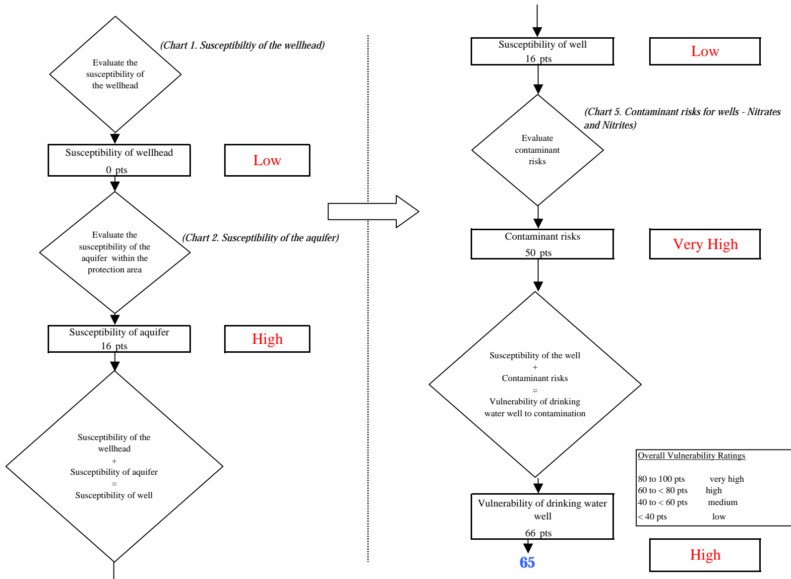
Chart 6. Vulnerability analysis for Blue Grouse Inn (242220.001) - Nitrates and Nitrites
