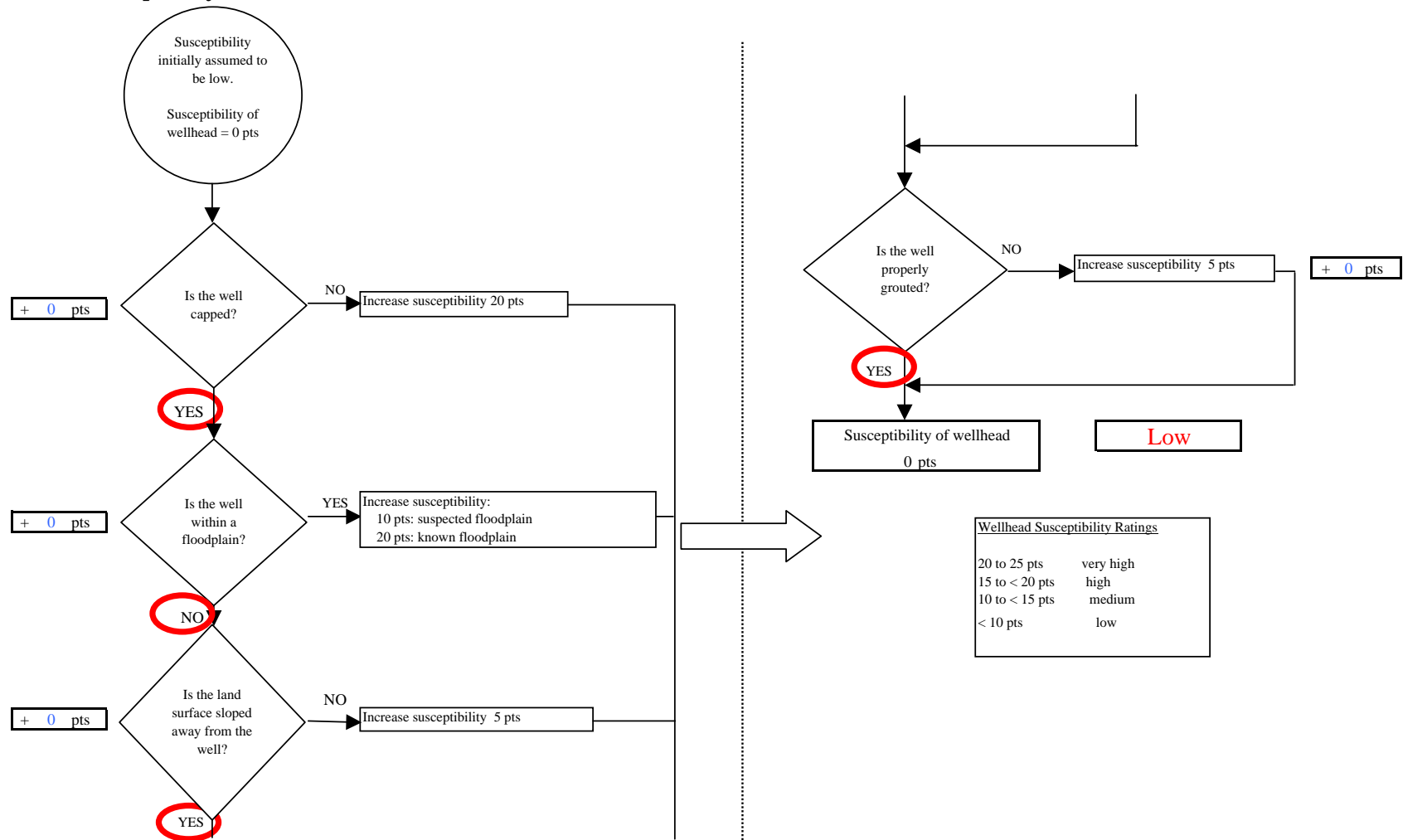
Chart 1. Susceptibility of the wellhead - Blue Grouse Inn (242220.001)
