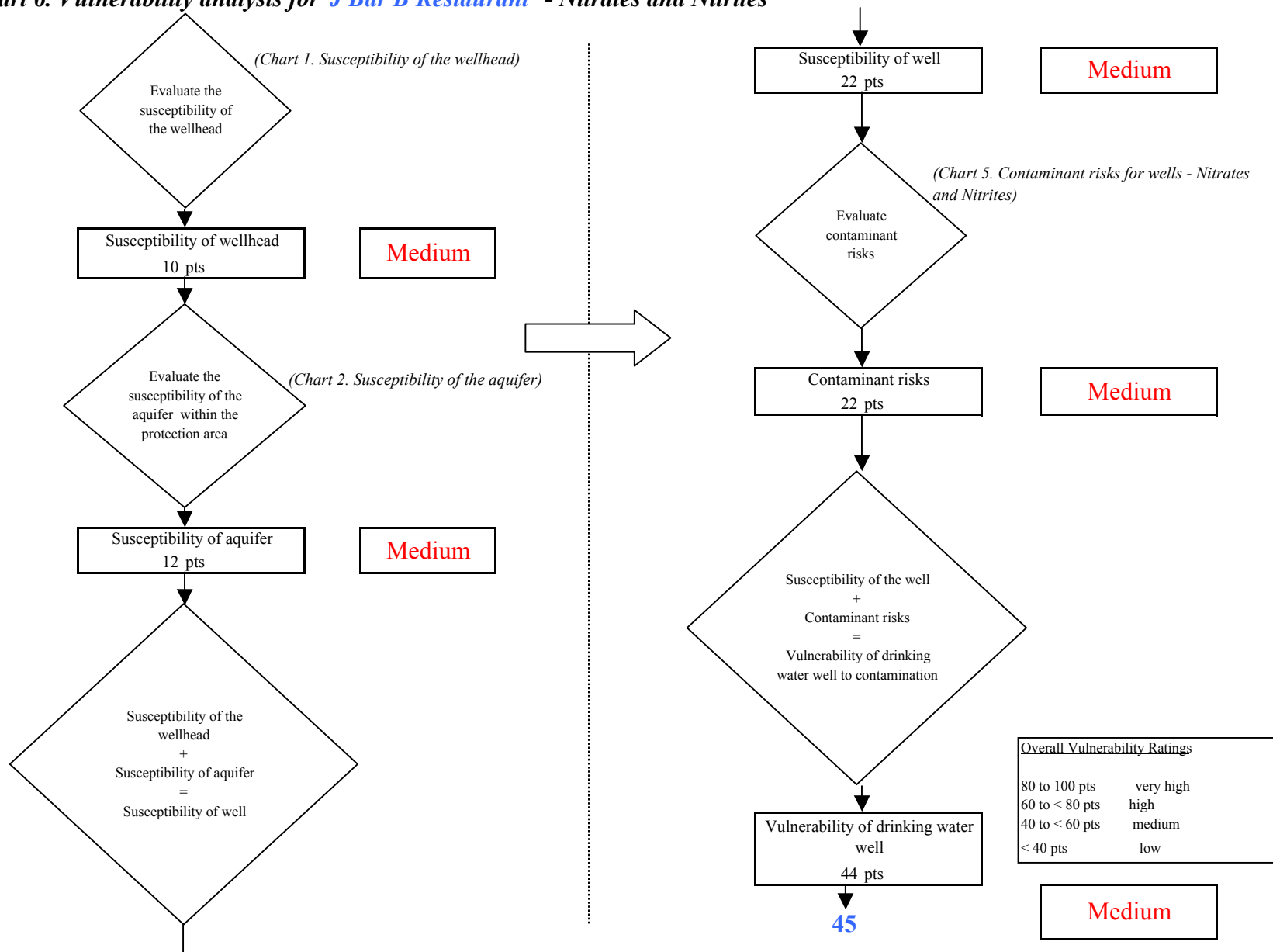
Chart 6. Vulnerability analysis for J Bar B Restaurant - Nitrates and Nitrites
