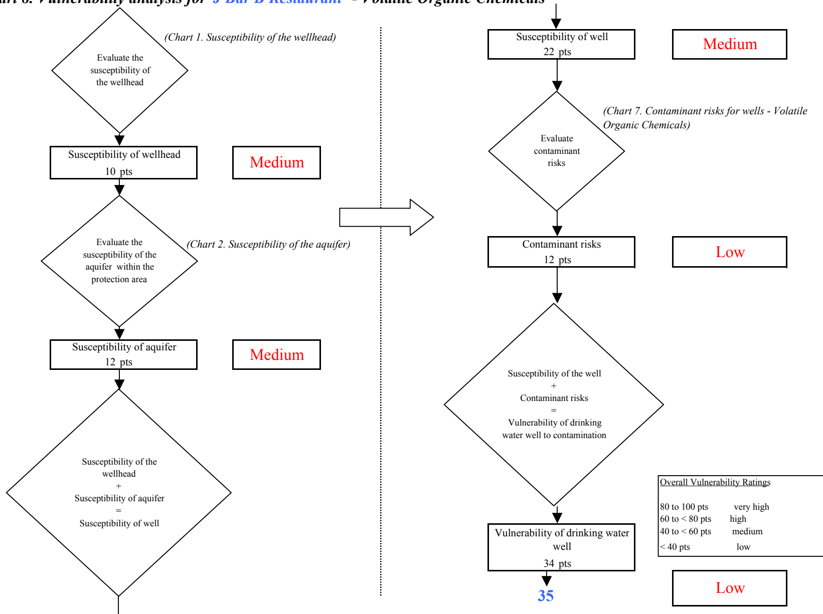
Chart 8. Vulnerability analysis for J Bar B Restaurant - Volatile Organic Chemicals
