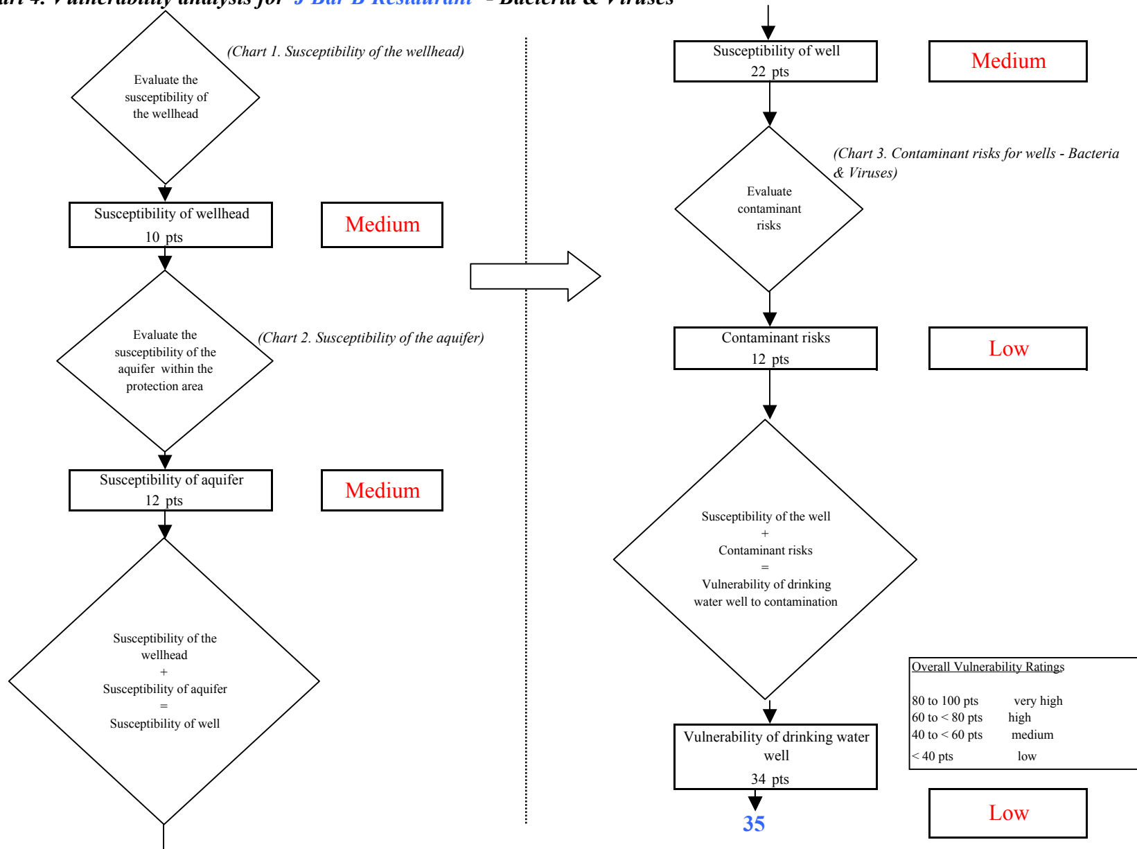
Chart 4. Vulnerability analysis for J Bar B Restaurant - Bacteria & Viruses
