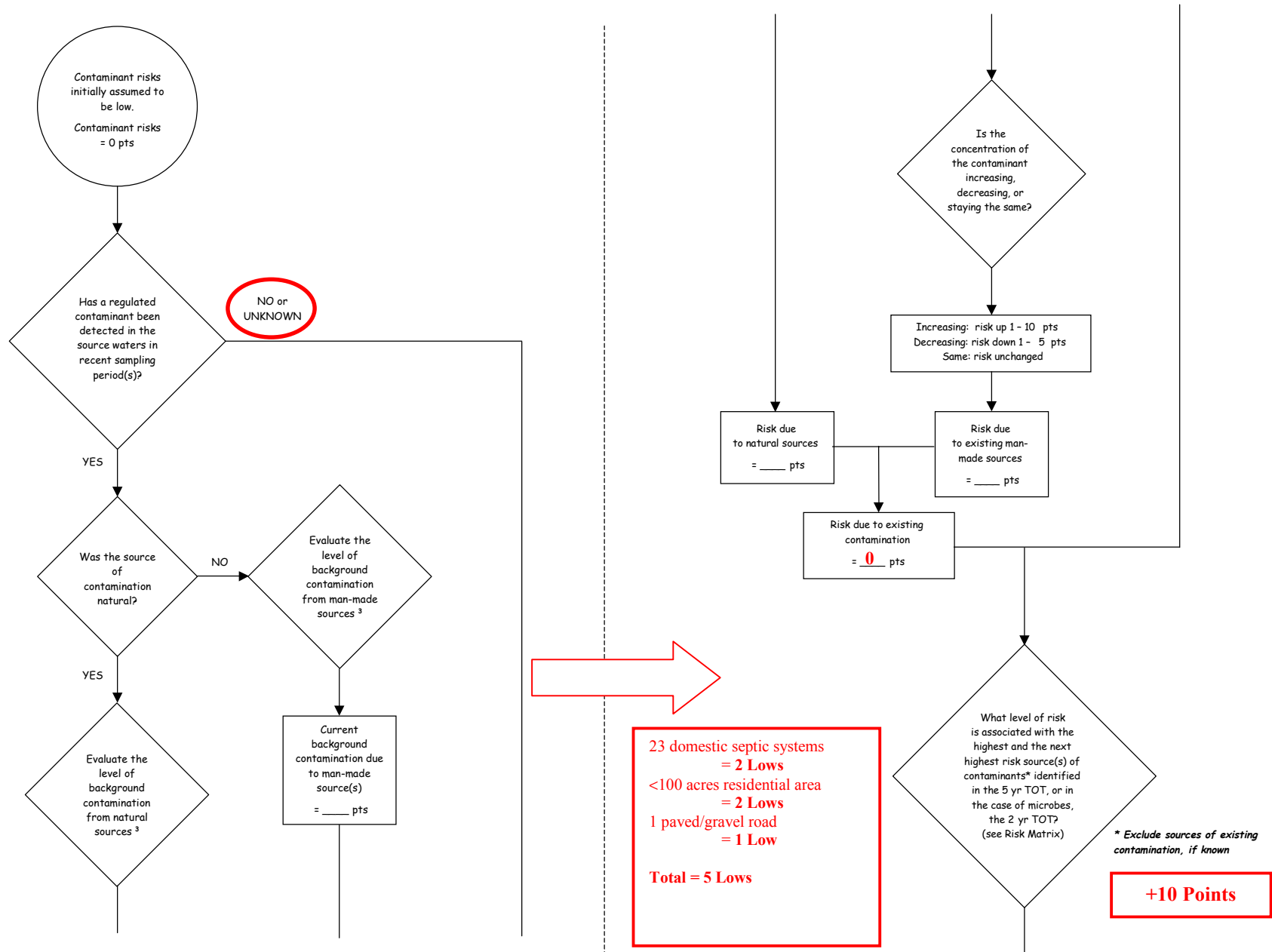
Chart 7. Contaminant risks for Big Lake Condos – Volatile Organic Chemicals
