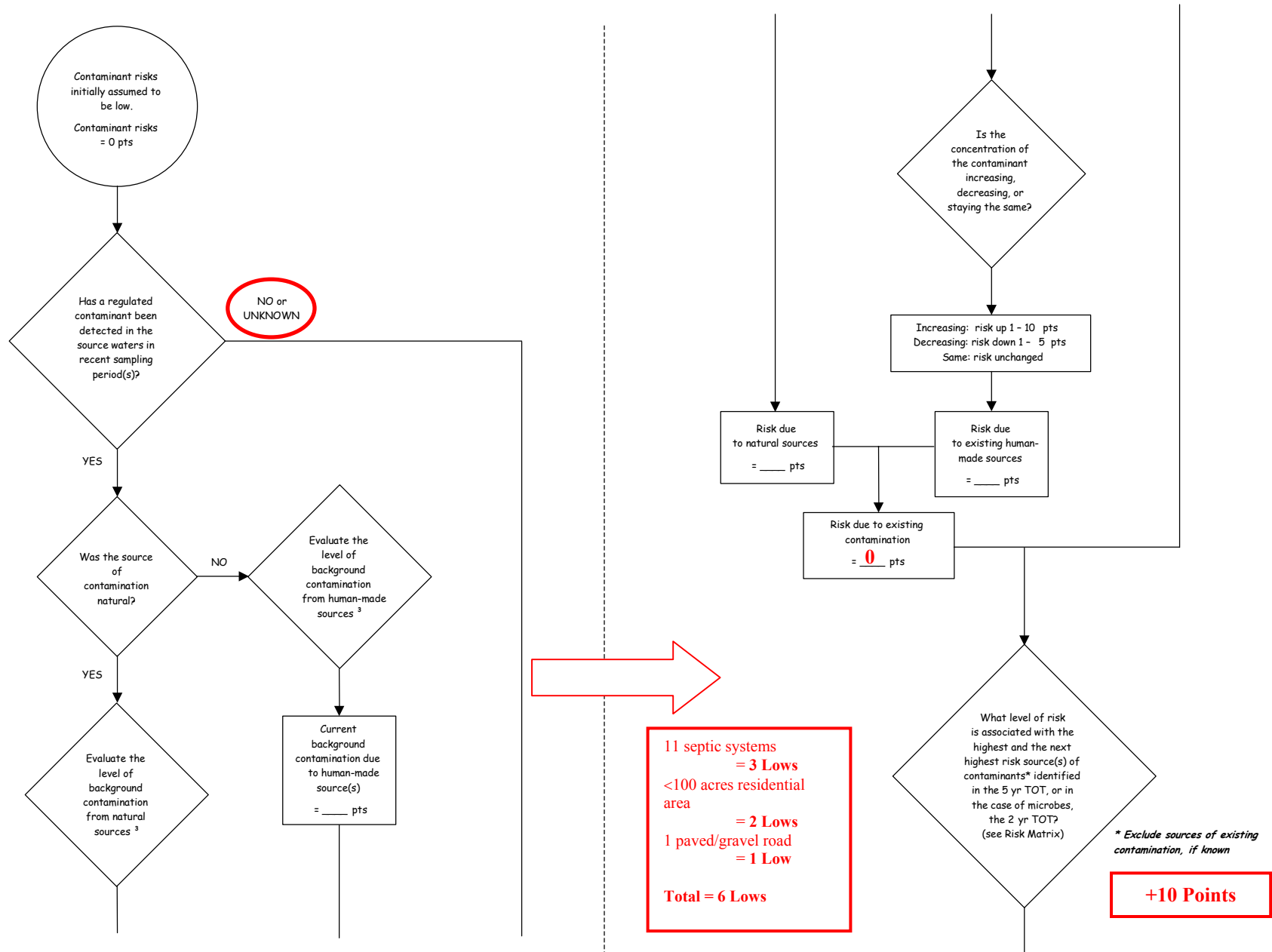
Chart 3. Contaminant risks for Big Lake Condos– Bacteria & Viruses
