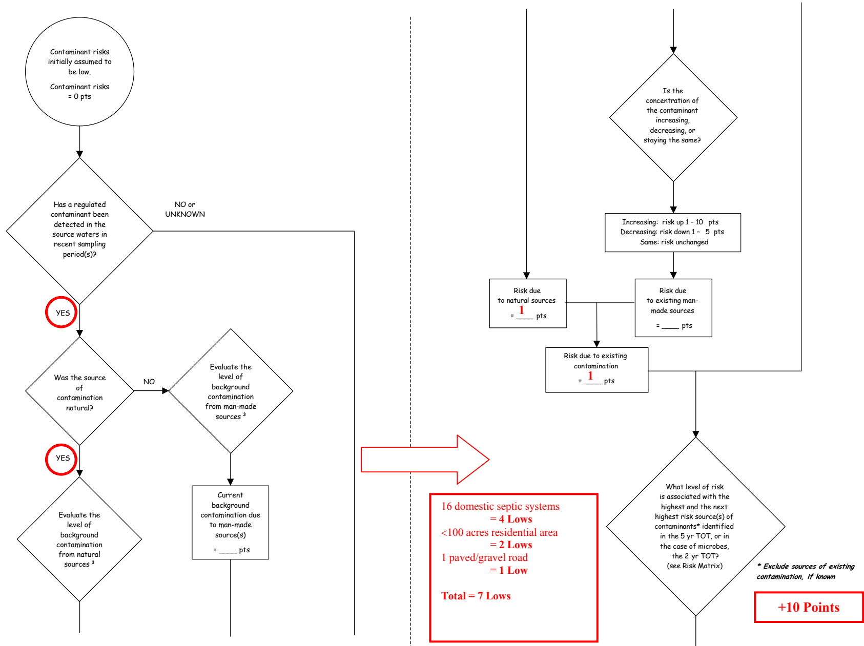
Chart 5. Contaminant risks for Big Lake Condos – Nitrates and Nitrites
