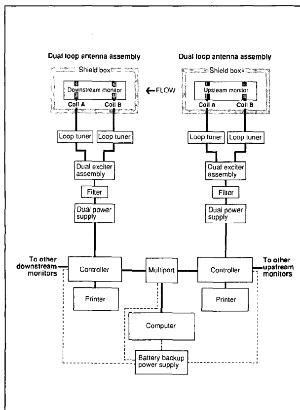
Figure 3 Typical PIT-tag monitoring system for dams.
