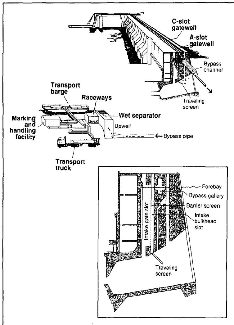
Figure 7 Typical hydroelectric dam with juvenile salmon collection facilities.
