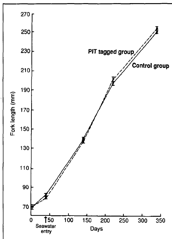
Figure 4 Comparison of length change between PIT-tagged (broken line) and control (solid line) fall chinook salmon (1984 brood) over time.
