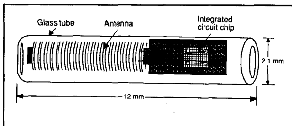
Figure 1 PIT tag.
