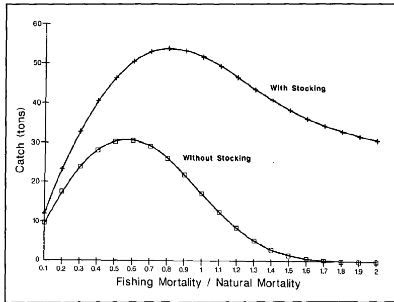
Figure 4 Equilibrium Ricker surplus production model with and without stocking. Curve without stocking based on biomass model B = S \exp(0.7 - 0.007S) ; curve with stocking based on B = S \exp(0.7 - 0.007S) + 25 .
