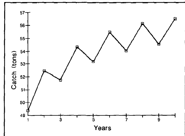
Figure 5 Simulation of yield with F = 1.0 when stocking occurs on even numbered years. Parameters of the Ricker surplus production model with stocking are: A = 1.2 , B = 0.007 , a(H_1)^b = 20t .
