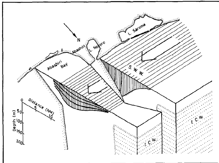
Figure 6 Schema of hydrographic structure generally observed in summer along the Okhotsk Sea coast. S.W.W. = Soya Warm Water; I.C.W. = Intermediate Cold Water; bold lines = temperature gradients.
