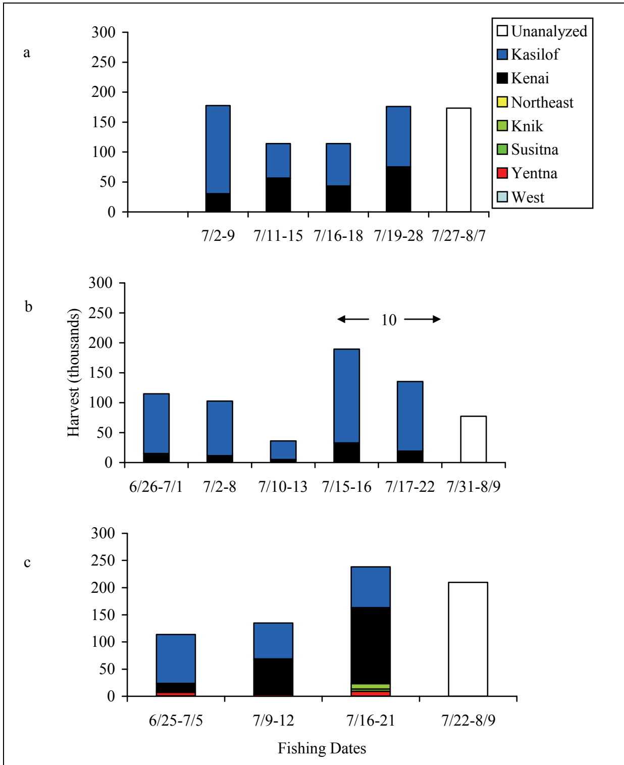
Figure 18. —Harvest by stock estimates for the Kasilof Section set gillnet fishery (Central District, East Side Subdistrict) from a) 2005, b) 2006, and c) 2007. 7/19-28, 2005 and 2007 REVISED - SEE ADDENDUM
