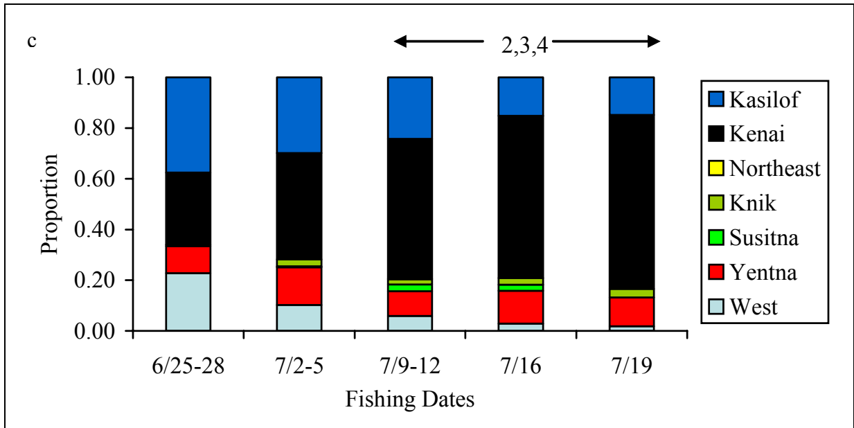
Figure 13. —Revised stock composition estimates for the Central District drift gillnet fishery from 2007.
