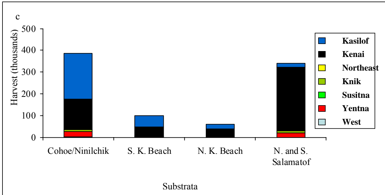
Figure 22. —Harvest by revised stock estimates for the Kasilof and Kenai Section set gillnet fisheries (Central District, East Side Subdistrict) divided into substrata from 2007.
