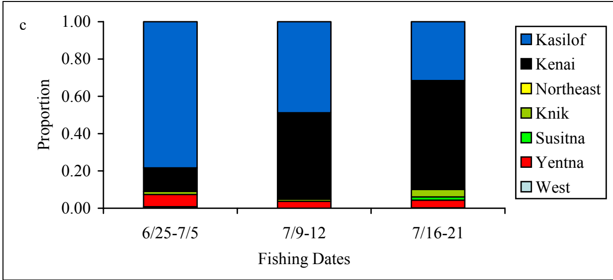
Figure 17. —Revised stock composition estimates for the Kasilof Section set gillnet fishery (Central District, East Side Subdistrict) from 2007.
