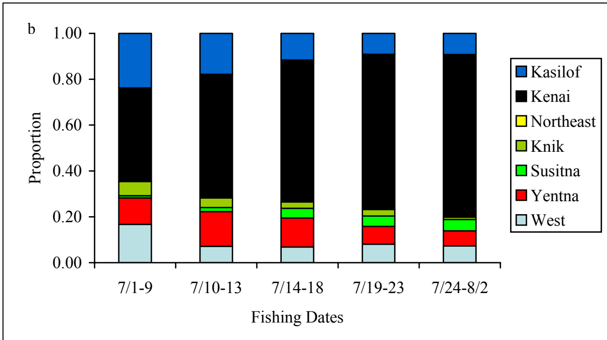
Figure 12. —Revised stock composition estimates for the Cook Inlet Offshore Test Fishery taken in 2007.
