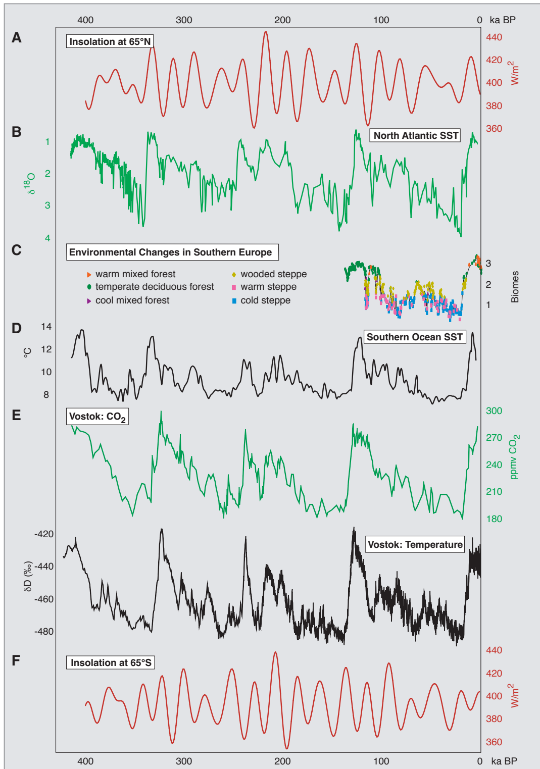
Fig. 3.2. Climatic proxies from both hemispheres over four glacial cycles. The last four glacial cycles as recorded in a variety of paleo-climate records. A. Summer insolation (21 June) at 65°N (Berger 1977). B. North Atlantic Sea Surface Temperature (SST) record of ODP site 980 (McManus et al. 1999). C. Allen et al. (1999) biomes record from lake Monticchio, southern Italy, over the last 100 ka. Biomes are statistical representations of vegetation derived from continental pollen records. D. South Indian ocean SST record from core MD 94-101 (Salvagnac 1998). Temperatures are obtained by foraminiferal transfer functions after Imbrie and Kipp (1971). E. Vostok CO 2 and \delta D (expressed as temperature) records (Petit et al. 1999). F. Summer insolation (21 dec.) at 65°S (Berger 1977).
