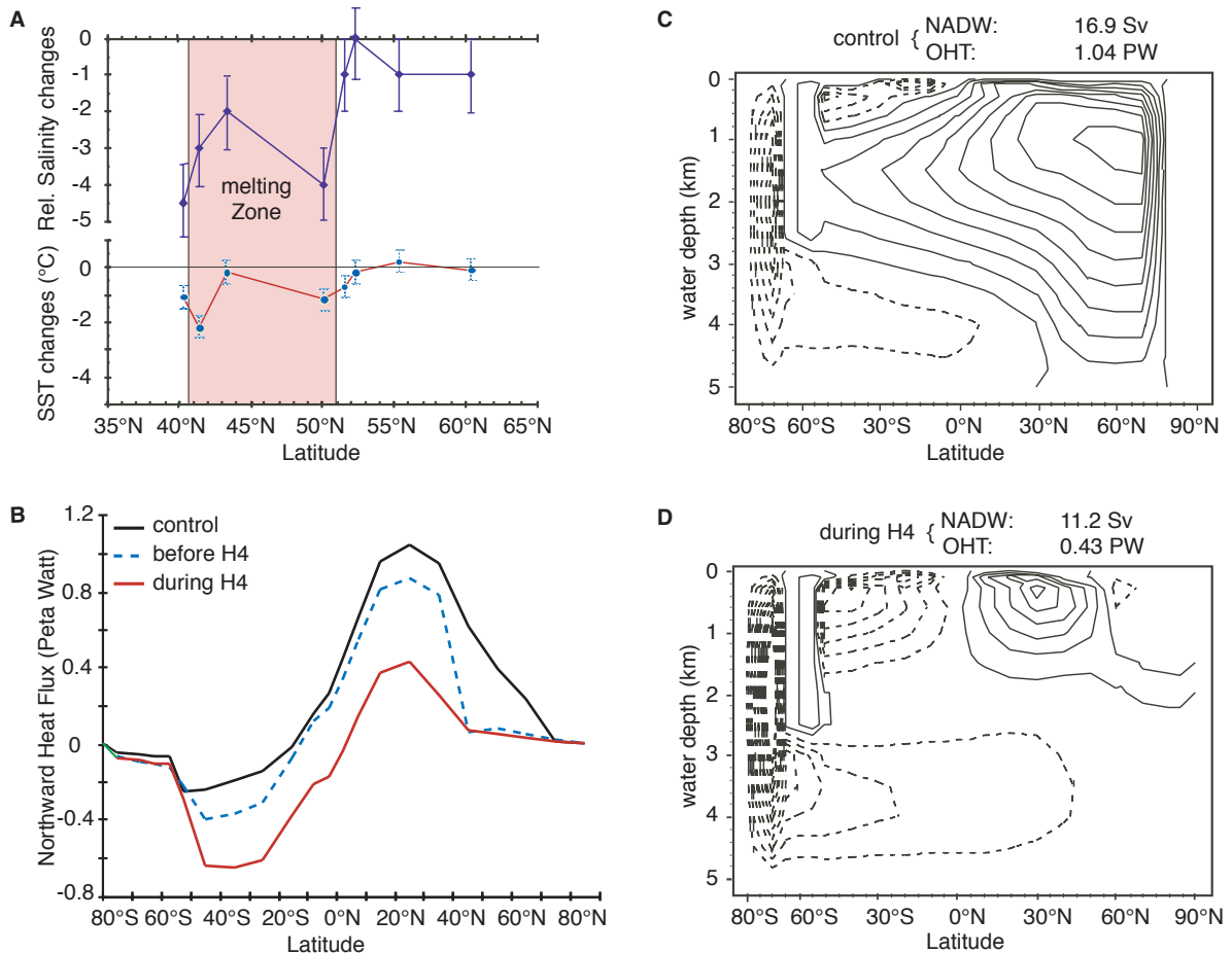
Fig. 3.5. 2-D zonal model simulation of the effect of Heinrich event H4 on thermohaline circulation adapted from (Paillard and Cortijo 1999). A. Zonal mean of the anomaly (H4 - before H4) for Sea Surface Salinity and Sea Surface Temperature, versus latitude. These data are used as input for the model. B. Changes in modeled northward oceanic heat transport for the control run, before H4 and during H4. C. Vertical distribution of the ocean heat fluxes for the control run, versus latitude. Flux of North Atlantic deep water (NADW) at its maximum is 16.9 Sv and oceanic heat transport (OHT) 1.04 PW. D. During H4: The model predicts a lower northern heat flux (by more than 50%) with a smaller NADW flux (11.2 Sv) and much shallower thermohaline circulation. Low latitude heat is preferentially transported to the Southern Hemisphere.
