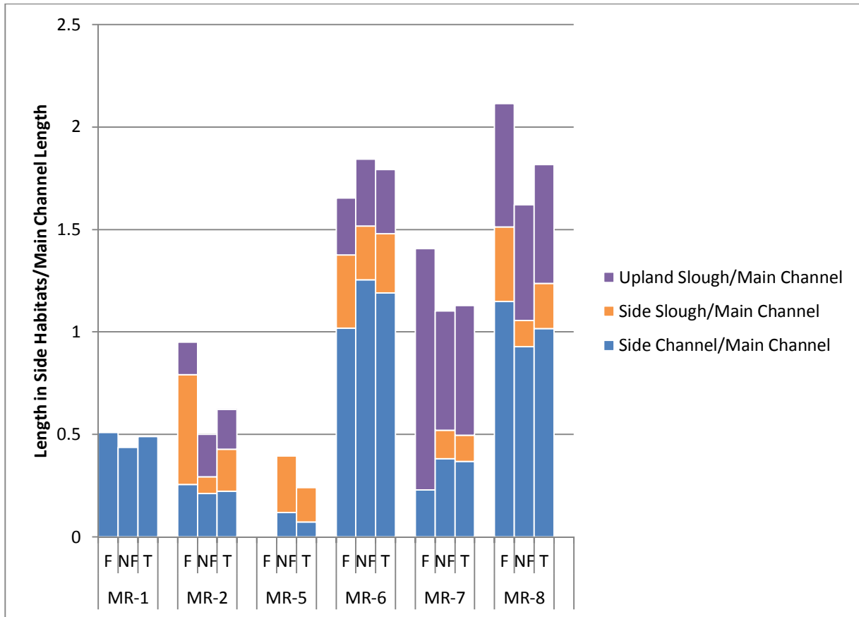
Figure 14. Side channel, side slough, and upland slough lengths per mile of main channel by geomorphic reach and focus area (F), non-focus area (NF), and total (T).
