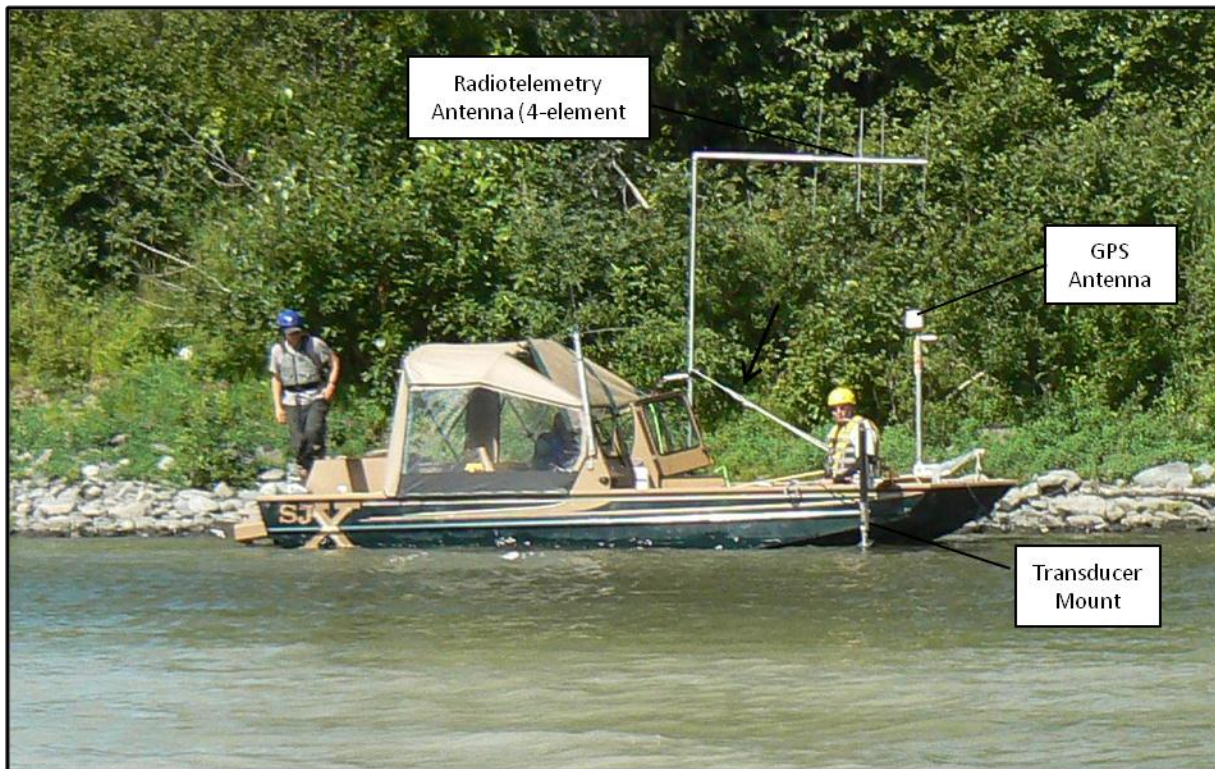
Photo 6. Setup for boat surveys using sonar to assess spawning activity in turbid water, July 28, 2012.
