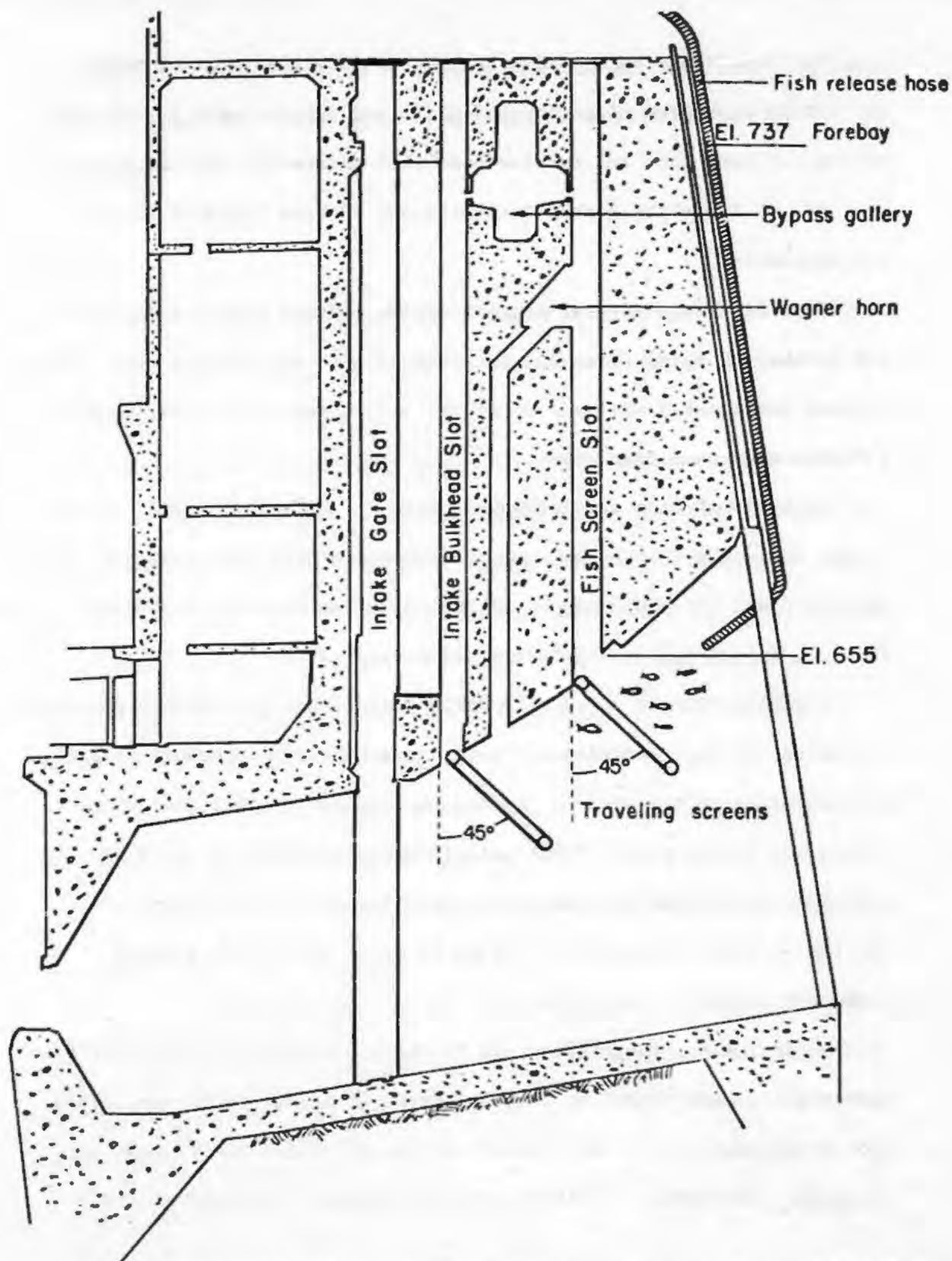
Figure 1.—Schematic drawing of traveling screen placement in the turbine intake at Lower Granite Dam. Traveling screens were tested in either the intake bulkhead slot or the fish screen slot at various angles from vertical (a screen angle of 45° is illustrated).
