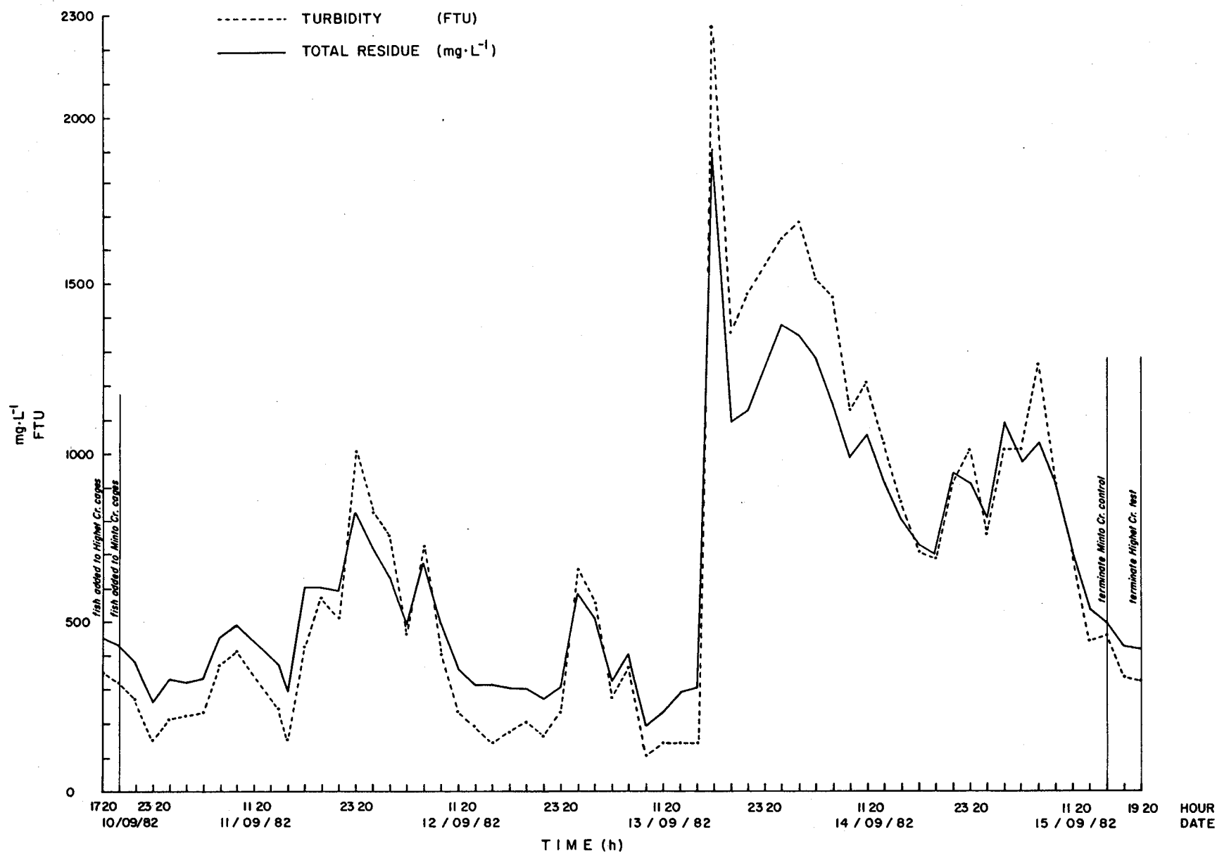
FIG. 25. Illustration of concentration of suspended sediment (total residue) and turbidity within cages held in Hight Creek during September 1982.
