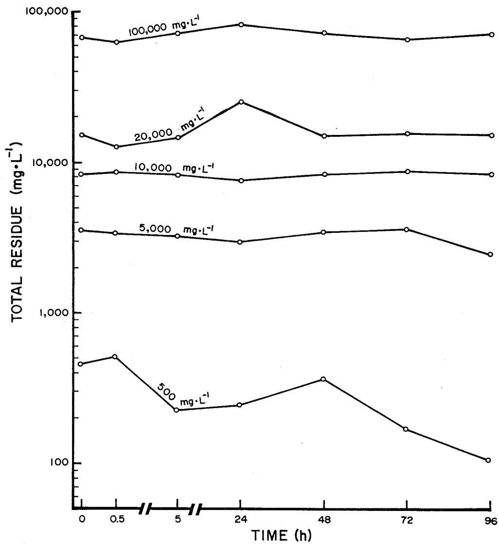
FIG. 9. Illustration of the stability of differing concentrations of suspended paydirt fines within recycle test tanks during a 96-h bioassay.
