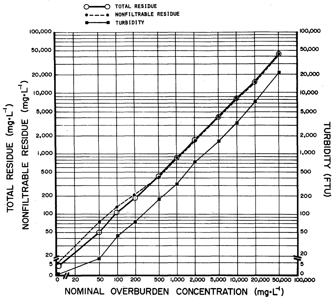
FIG. 8. Relationship of total residue, nonfiltrable residue and turbidity for suspensions of overburden sediment in freshwater.
