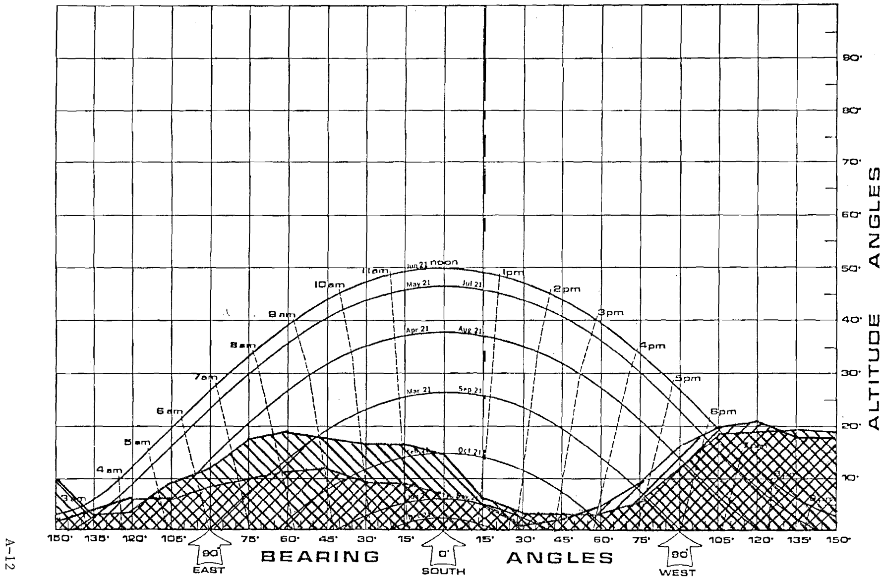
Sun path diagram for 64°N latitude.
