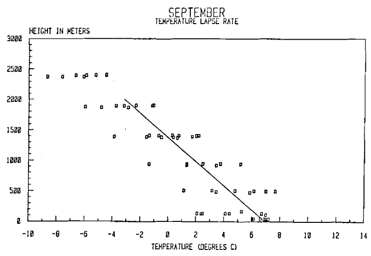
Figure 7. Vertical air temperature distribution. Anchorage and Fairbanks 1968, 1969, 1970, 1980, 1981, 1982.
