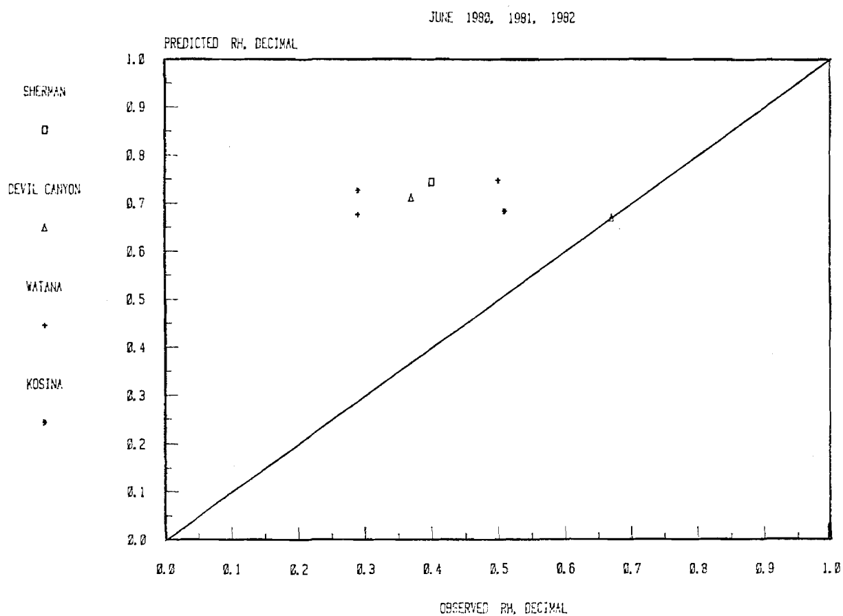
Figure 19. Susitna observed humidities vs. humidities predicted from Talkeetna data.
