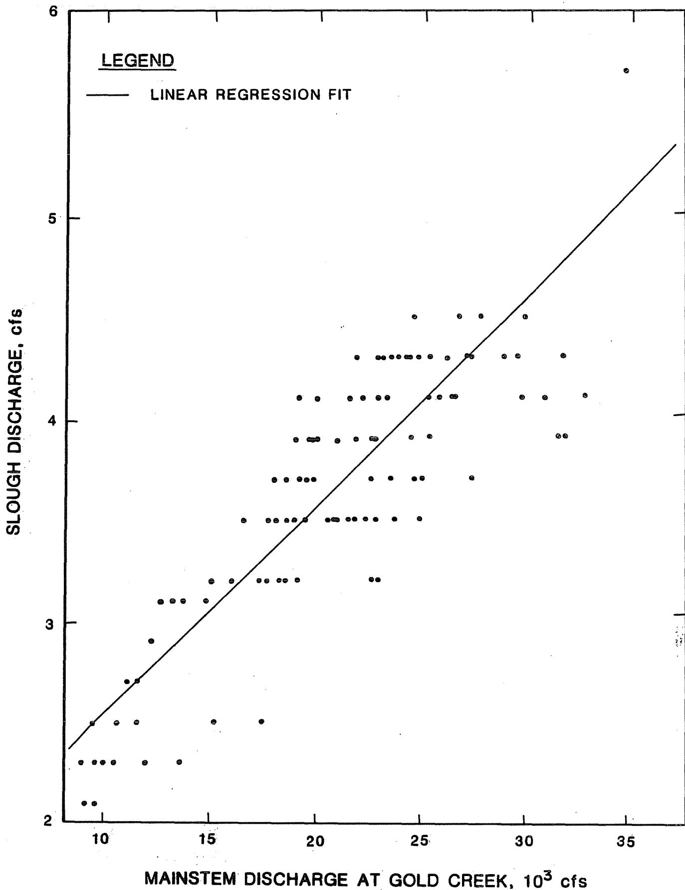
SLOUGH 11 DISCHARGE VS. MAINSTEM DISCHARGE AT GOLD CREEK, SUMMER 1983
