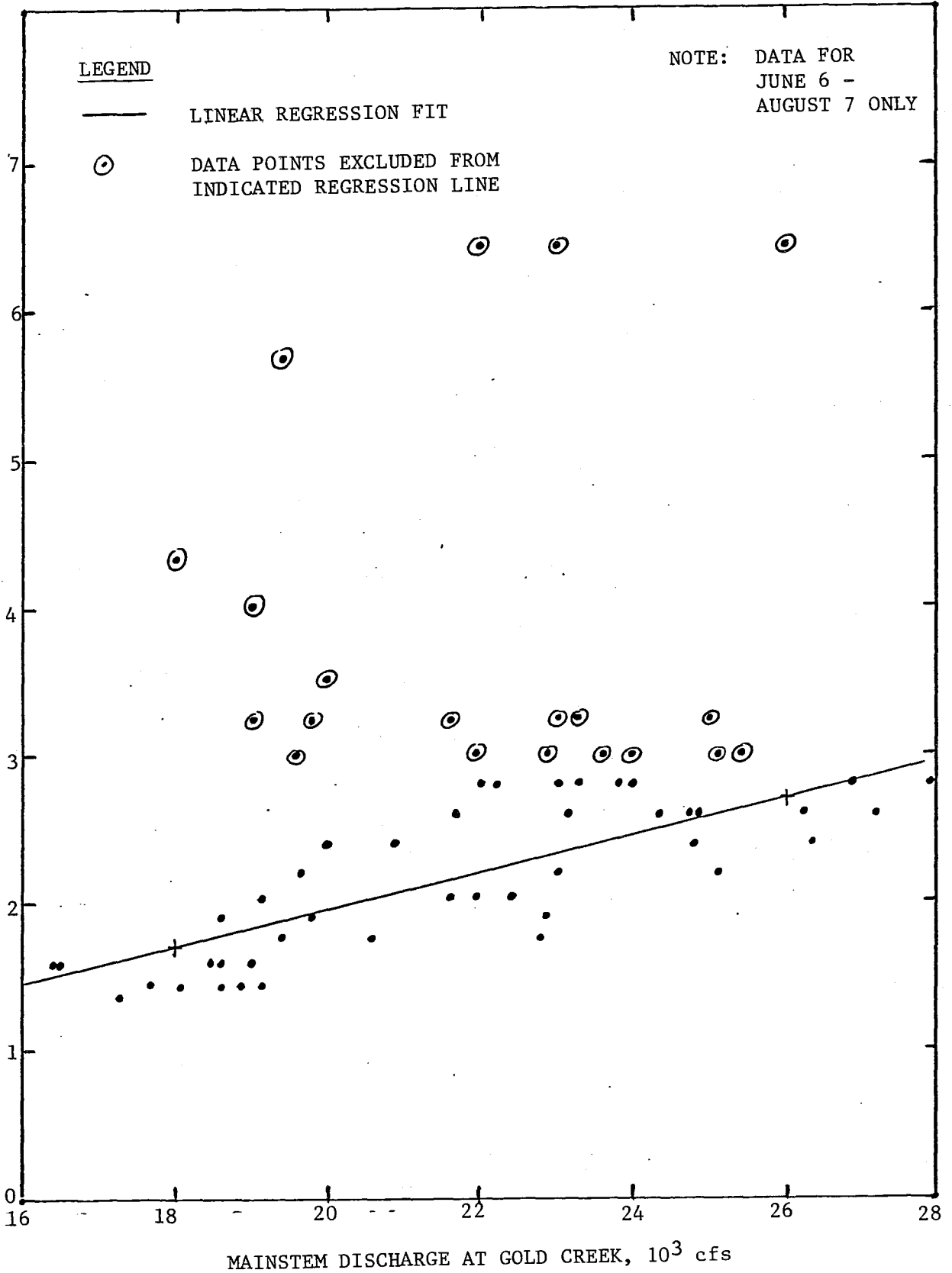
EXHIBIT 18b. SLOUGH 8A DISCHARGE VS. MAINSTEM DISCHARGE AT GOLD CREEK, SUMMER 1983
