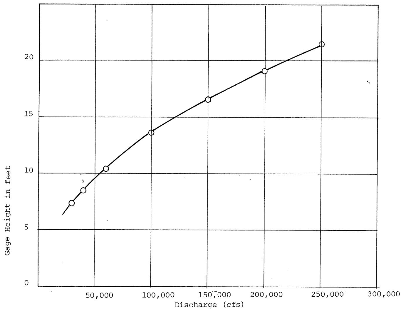
STAGE-DISCHARGE RELATIONSHIP SUSITNA RIVER AT SUSITNA STATION FIGURE 5.4
