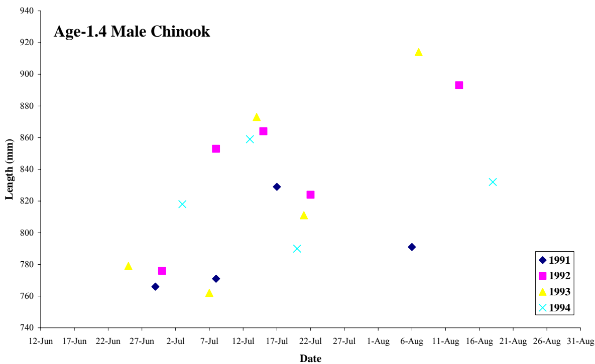
Figure 7.- Inseason changes in average length for age-1.4 Chinook observed at Tuluksak River weir.
