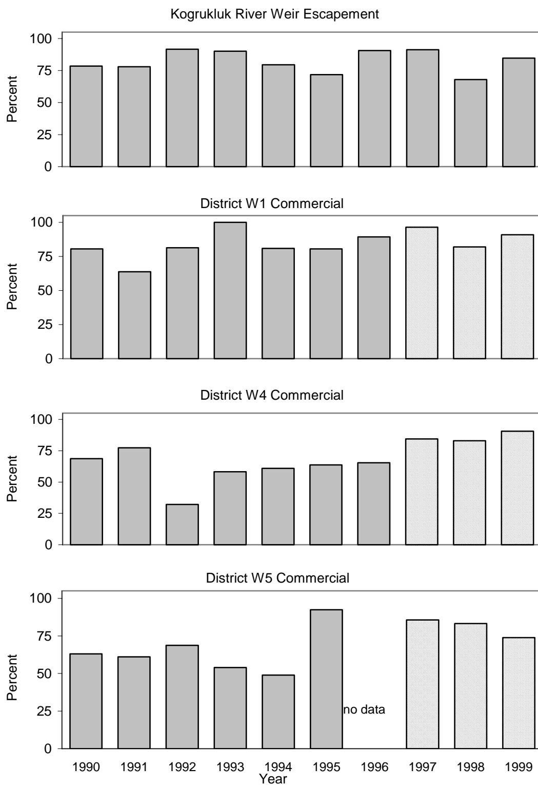
Figure 10.- Historical percentage of age-1.3 Chinook salmon reported as males from Kogruklu River weir and Districts 1, 4 and 5, 1990-1999. Hatch-marked bars only include data for fish with confirmed sex identification.
