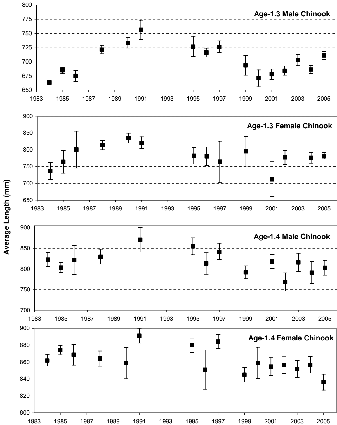
Figure 15.- Historical average annual length with 95% confidence intervals for Chinook salmon at Kogrukluk River weir (Jasper and Molyneaux In prep ).
