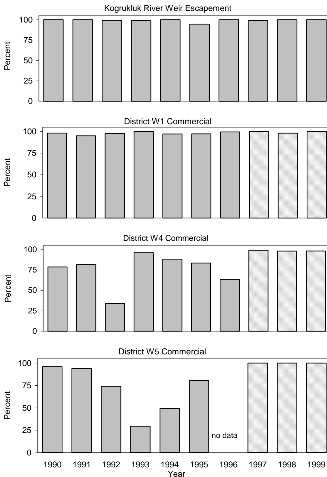
Figure 3.- Historical percentage of age-1.2 Chinook salmon reported as males from Kogrukluk River weir and Districts 1, 4 and 5, 1990–1999. Hatch-marked bars only include data for fish with confirmed sex identification.
