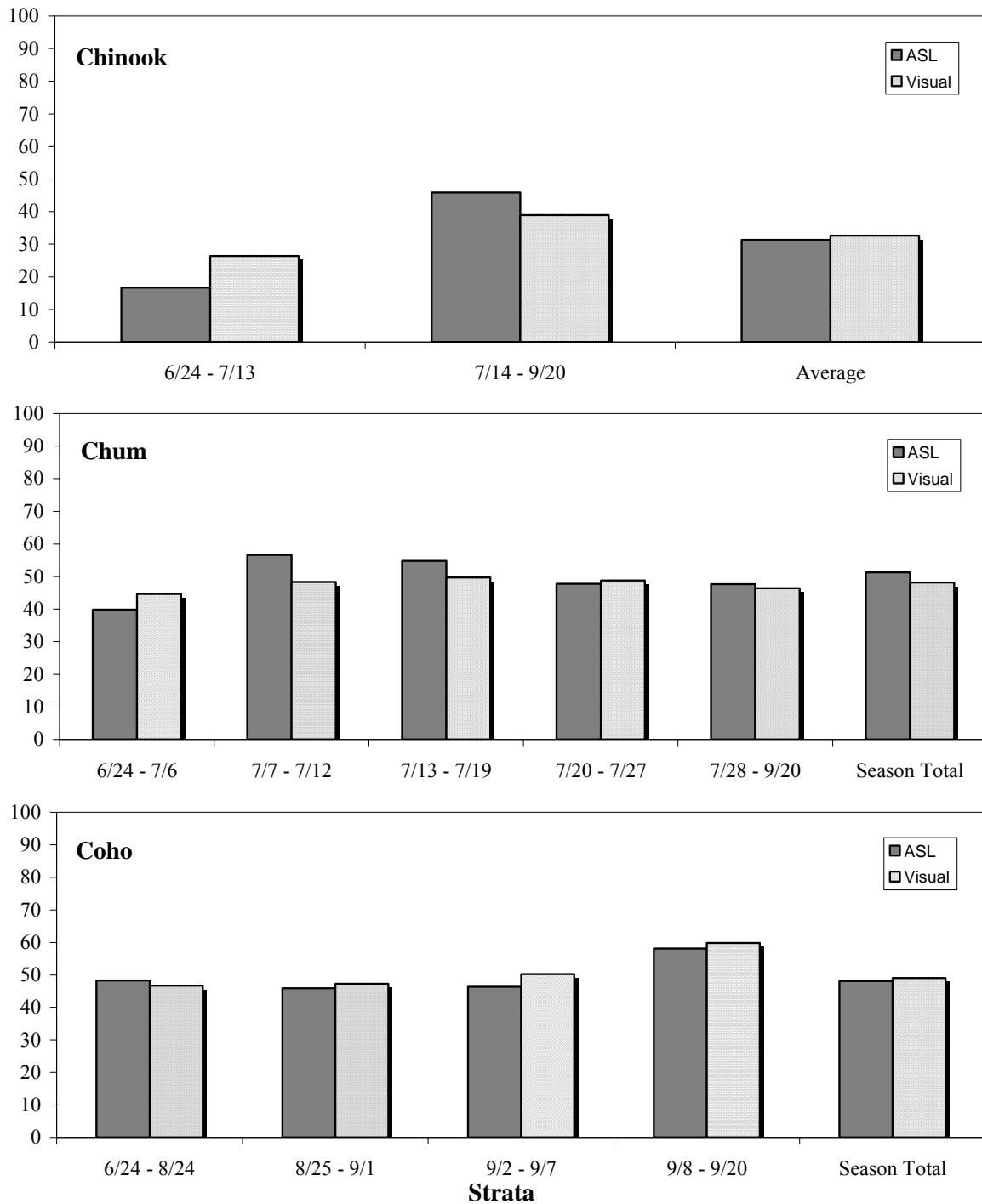
Figure 8.- Percentage of females per strata as determined by ASL sampling compared to visual identification at Takotna River weir, 2005 (Costello et al. 2006a).
