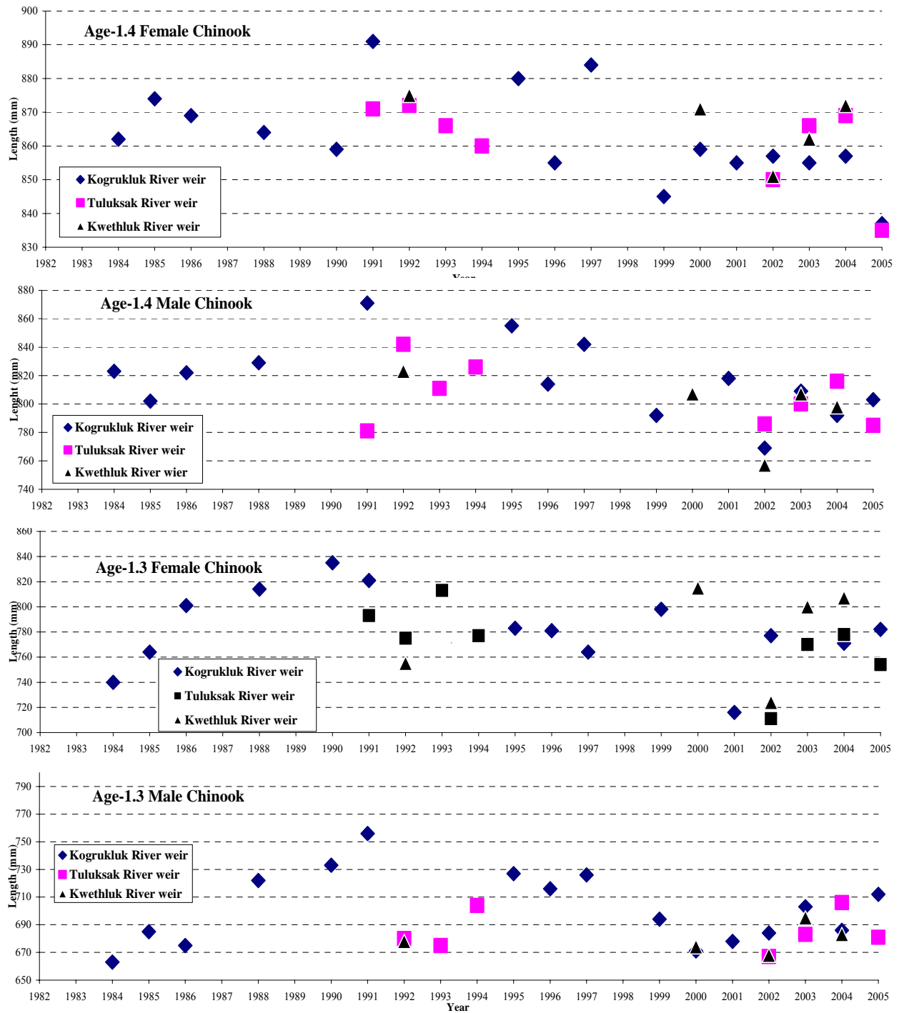
Figure 14.- Length-at-age for Chinook salmon at three Kuskokwim River tributary escapement projects.
