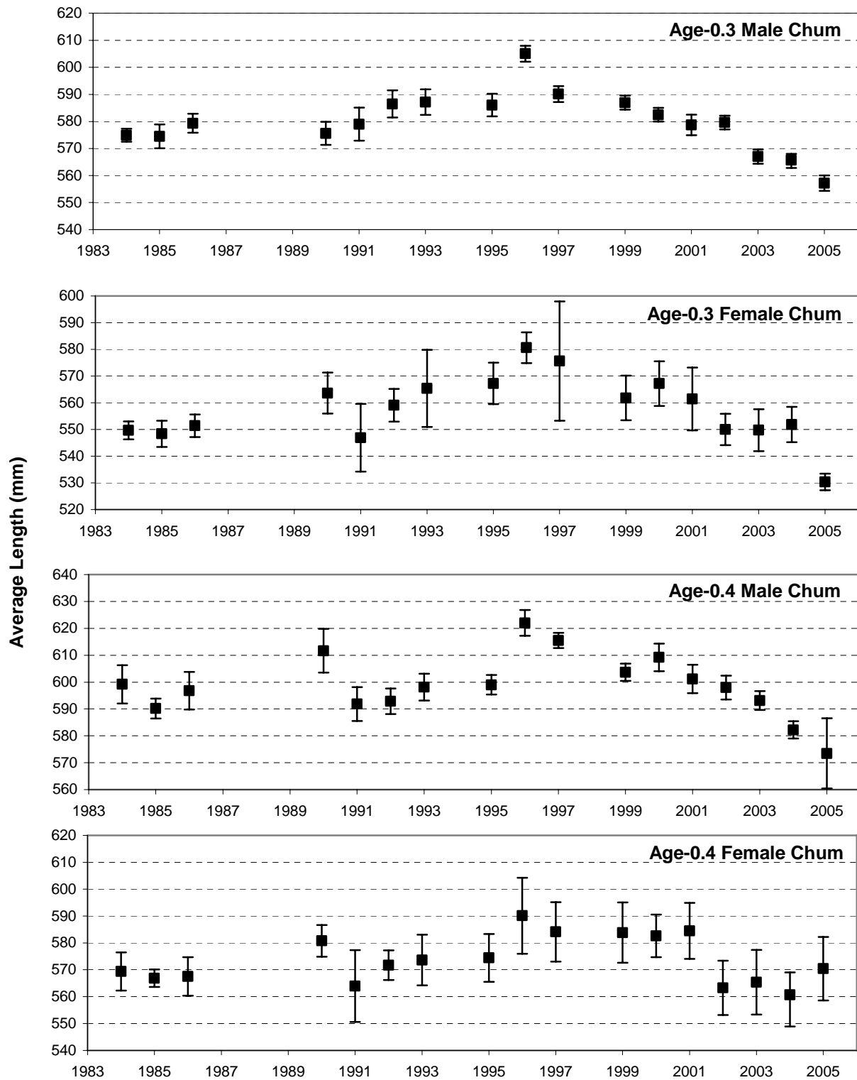
Figure 29.- Historical average annual length with 95% confidence intervals for chum salmon at Kogruklu River weir (Jasper and Molyneux In prep ).
