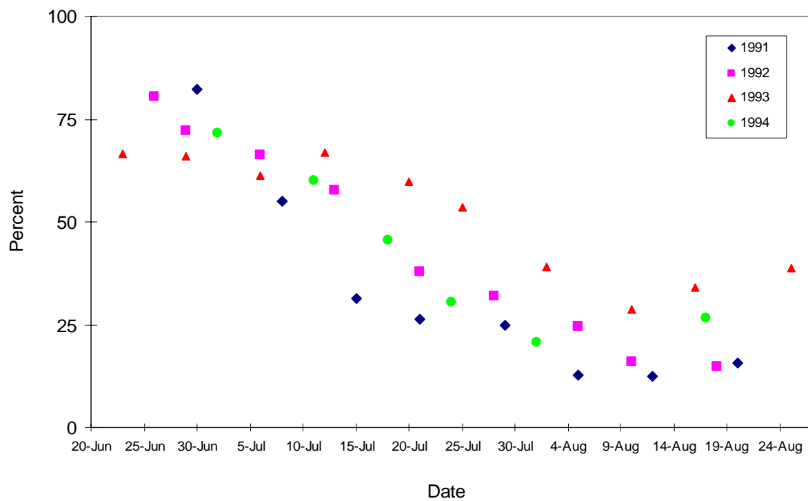
Figure 22.- Percent of the chum salmon migration composed of age-0.2 fish in 2002 at Kuskokwim Area tributary escapement projects.
