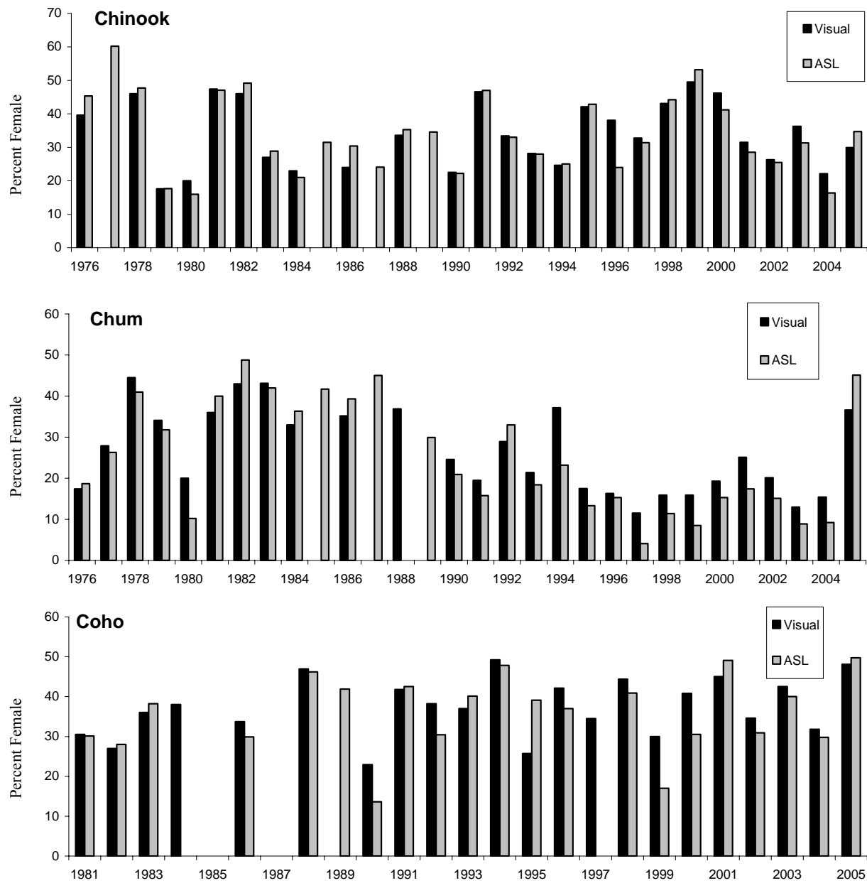
Figure 9.- Historical annual percentage of female salmon as determined by weighted ASL sampling and visual identification at the Kogruklu River weir.
