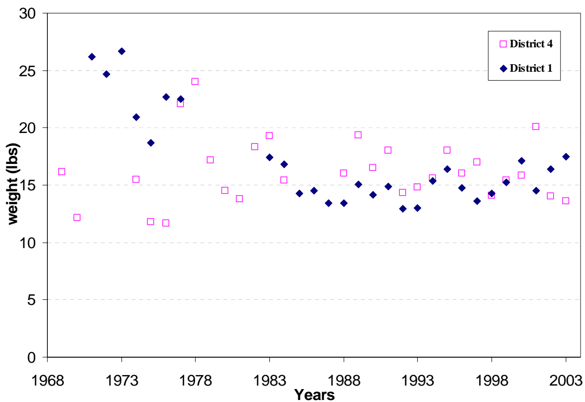
Figure 16.- Average weight by year of commercially caught Chinook salmon in Kuskokwim area fishing Districts 1 and 4.
