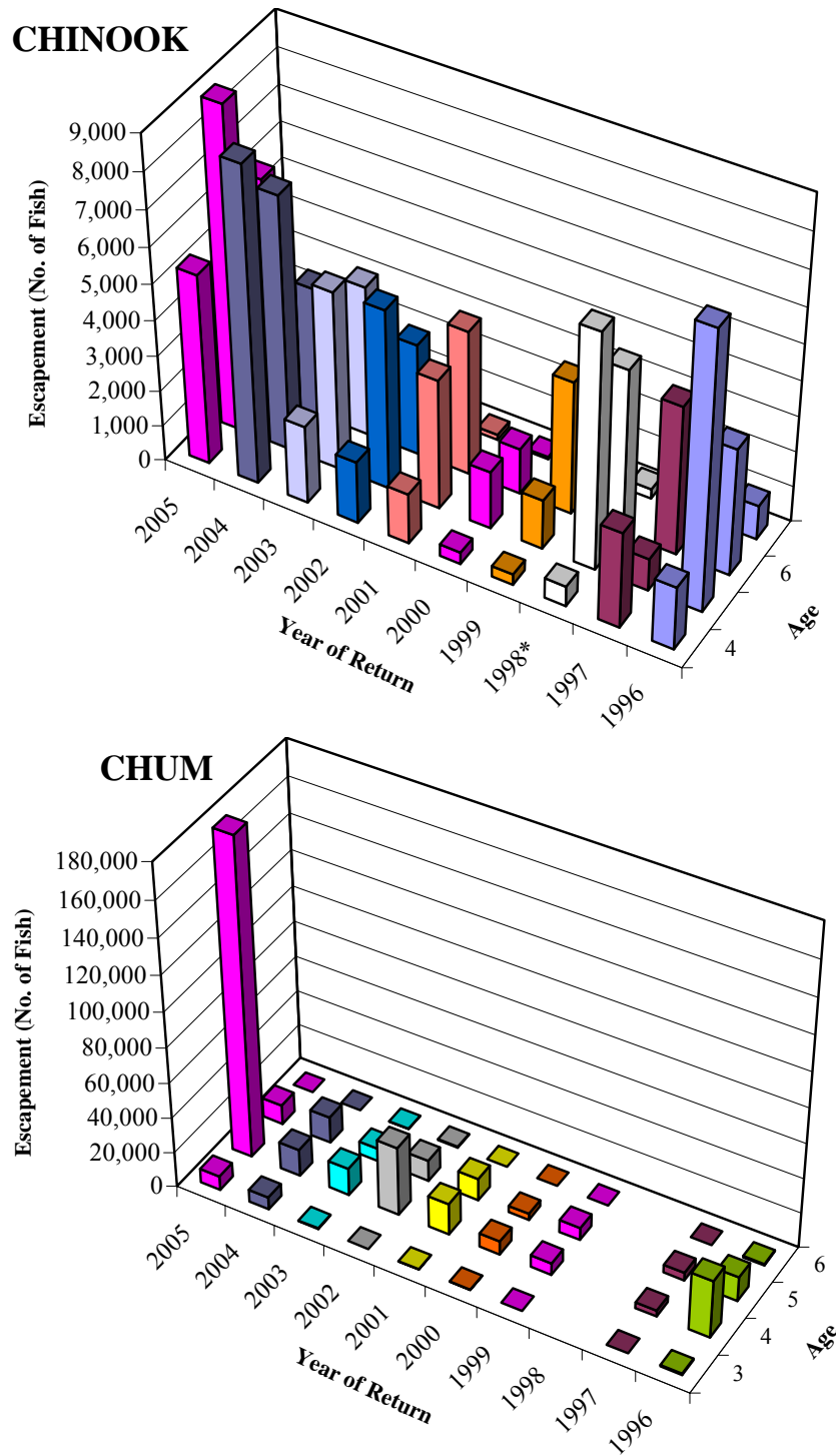
Figure 6.- Chinook and chum salmon age distribution over time at the Kogruklu River weir (Jasper and Molyneaux In prep ).
