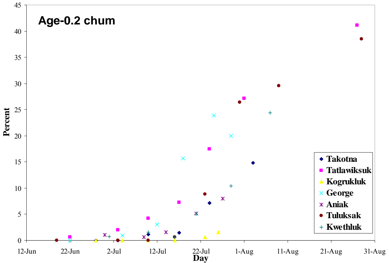
Figure 21.- Percent of the chum salmon migration composed of age-0.2 fish in 2002 at Kuskokwim Area tributary escapement projects.
