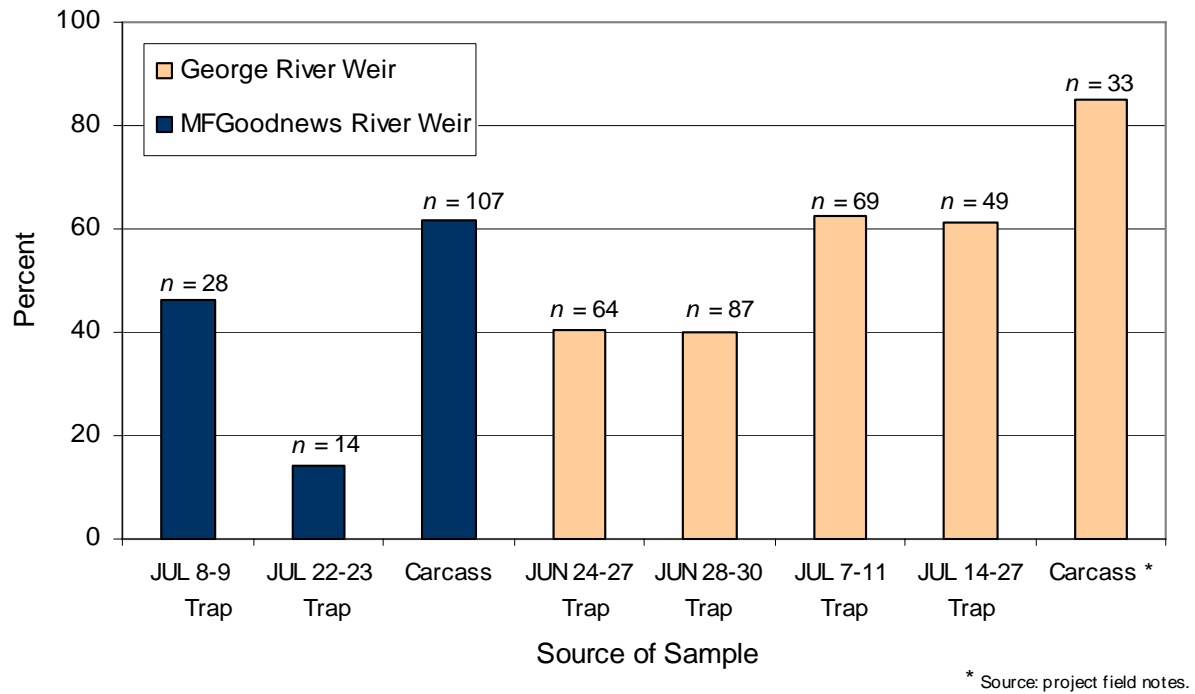
Figure 2.- Percentage of male Chinook salmon in trap and carcass samples from the Middle Fork Goodnews River weir in 1996 and the George River weir in 1997.
