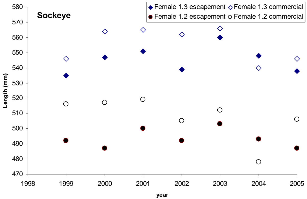
Figure 20.- Comparison of average length by year of female sockeye salmon sampled from the W5 commercial fishery and at the Middle Fork Goodnews River weir.
