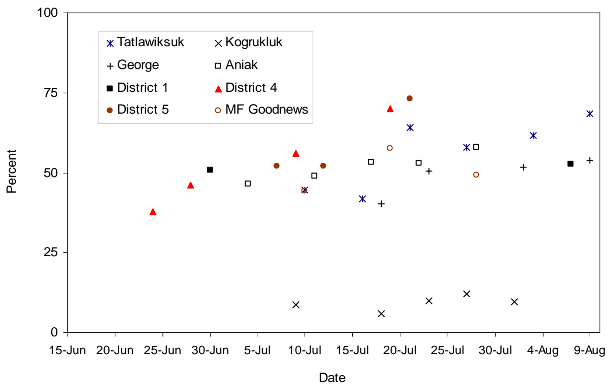
Figure 24.- Percentage of female chum salmon by sample date from Kuskokwim Area tributary escapements and commercial catches, 1999.
