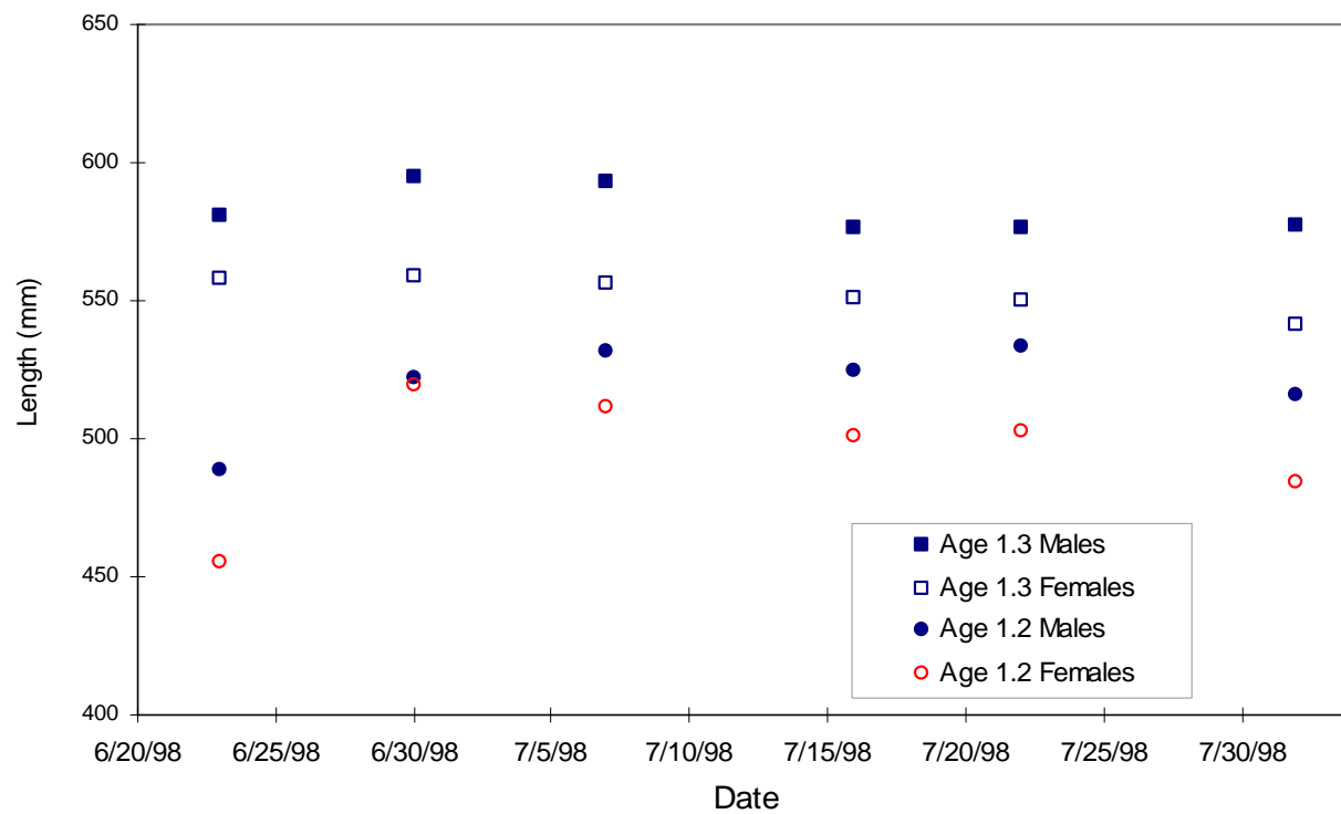
Figure 19.- Average length by sample date for Kanektok River sockeye salmon in 1997.
