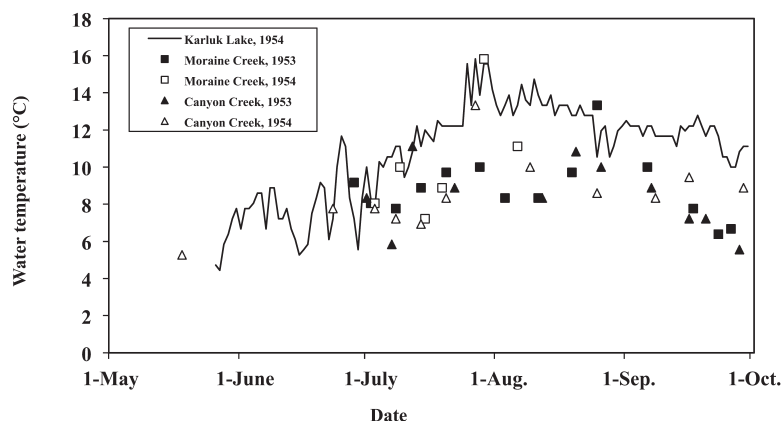
Figure 7-1. Surface water temperatures of Karluk Lake (1954), a lateral tributary (Moraine Creek, 1953–1954), and a terminal tributary (Canyon Creek 1953–1954). From Bevan and Walker (1954, 1955).
