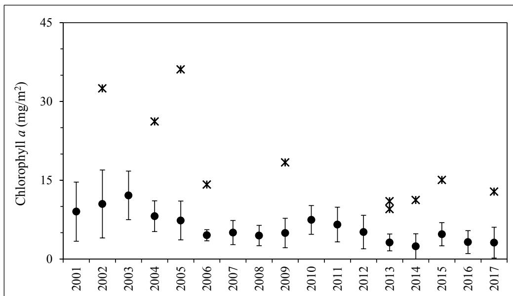
Figure 17.—Tributary Creek Site 9 chlorophyll a densities.
