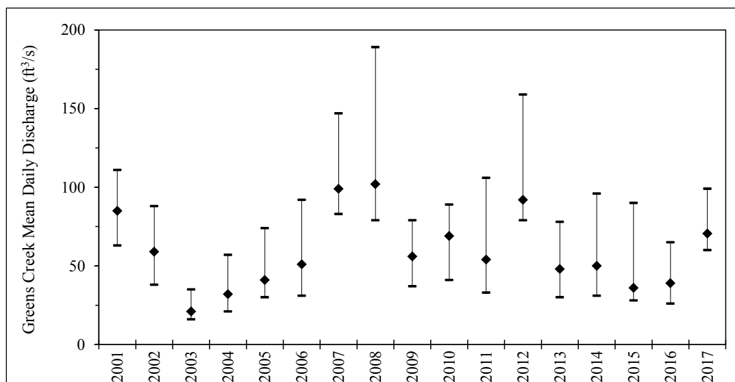
Figure 6.—Greens Creek mean daily discharges three weeks prior to sampling, 2011–2017.
