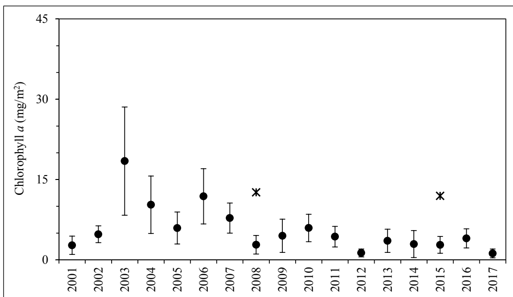
Figure 7.—Greens Creek Site 48 chlorophyll a densities.
