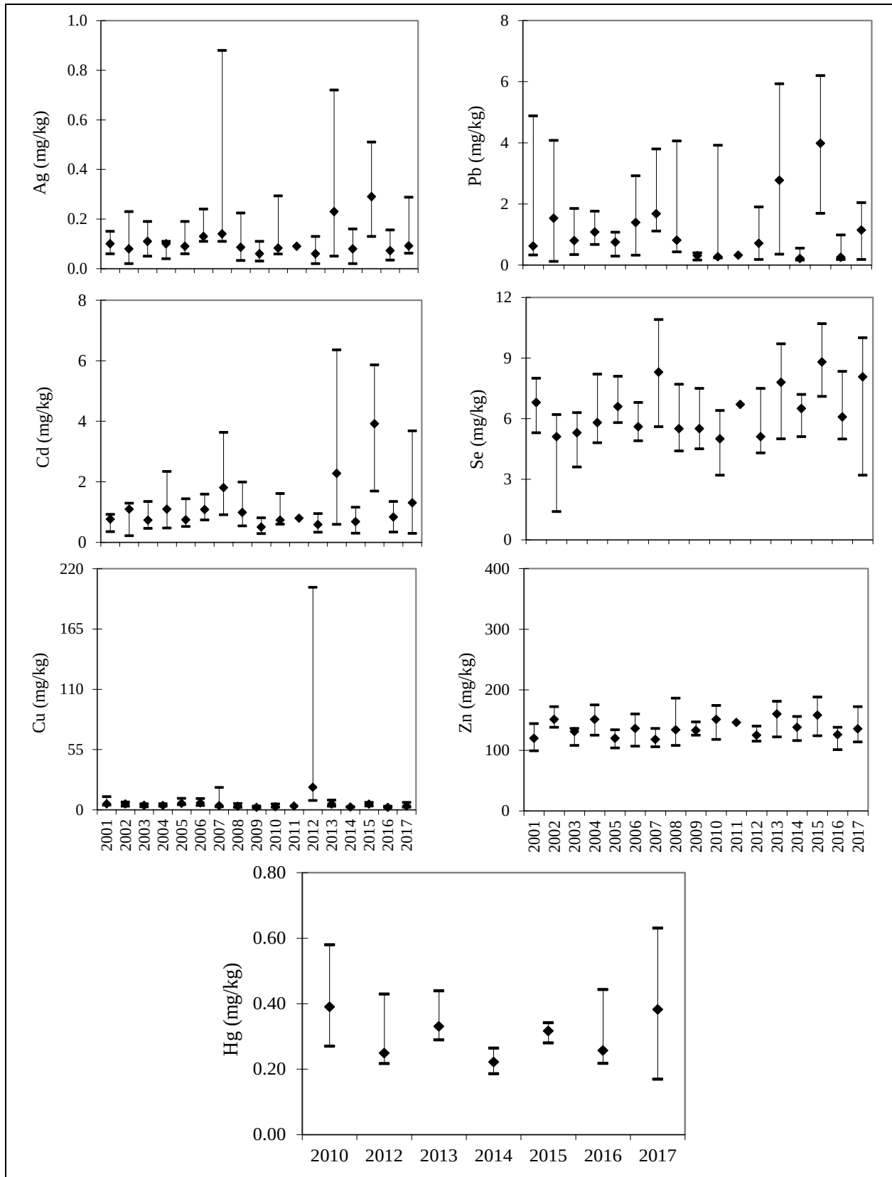
Figure 21.–Tributary Creek Site 9 Dolly Varden char element concentrations. Note: Minimum, median, and maximum whole body concentrations presented.
