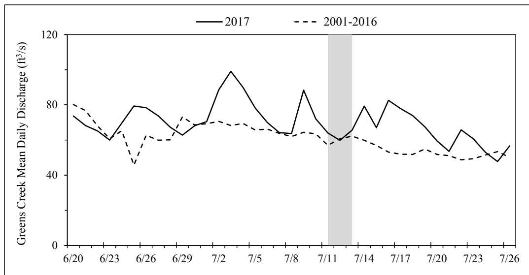
Figure 5.—Greens Creek mean daily discharge three weeks prior to sampling in 2017.
