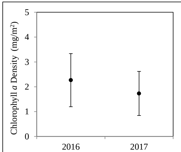
Figure 5.–Lower Glacier Creek mean chlorophyll a densities \pm 1 SD.
