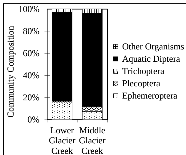
Figure 18.–2017 Glacier Creek mean benthic macroinvertebrate community compositions.
