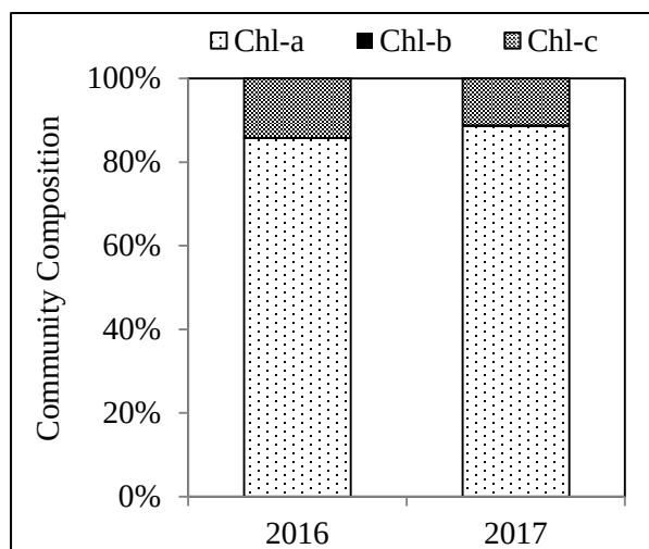
Figure 11.–Middle Glacier Creek mean proportions of chlorophylls a , b , and c .
