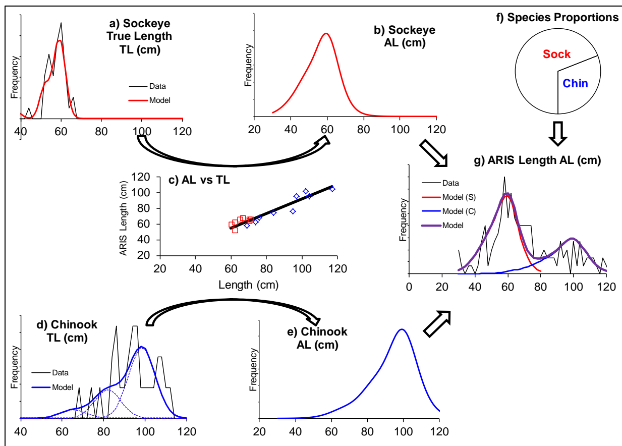
Appendix C2.—Flow chart of a mixture model.
