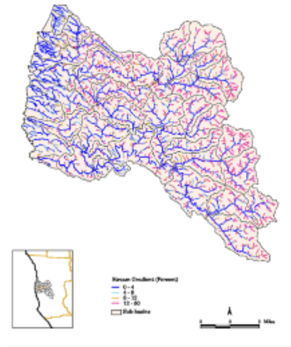
Figure 3: Noyo and Big River Stream Gradient
