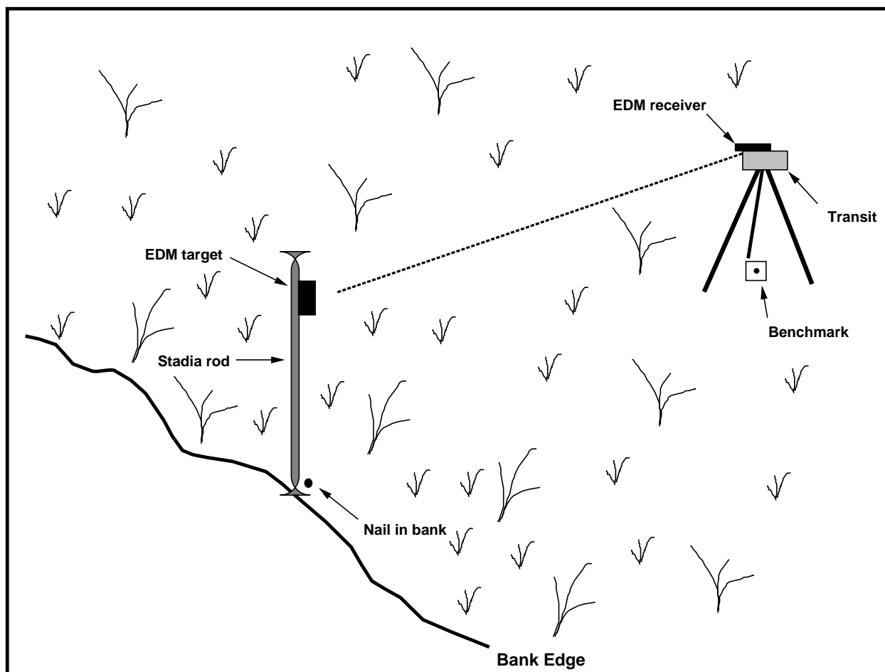
Figure 3.—Schematic of instrument layout for taking bank position measurements, 2000.
