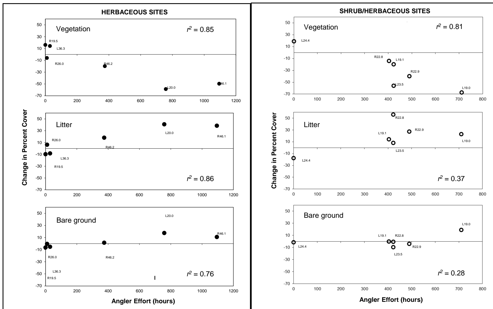
Figure 7.—Angler effort (2000) versus mean change (prefishery to postfishery) in percent cover of vegetation (top), litter (middle), and bare ground (bottom) for permanent vegetation plots at herbaceous (left) and shrubland/herbaceous (right) habitat sites ( n = 6 each), Kenai River.
