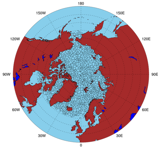
Figure 1. Voronoi tessellation of points randomly seeded in the polar region to use as initial set of polygons for sea ice representation.
