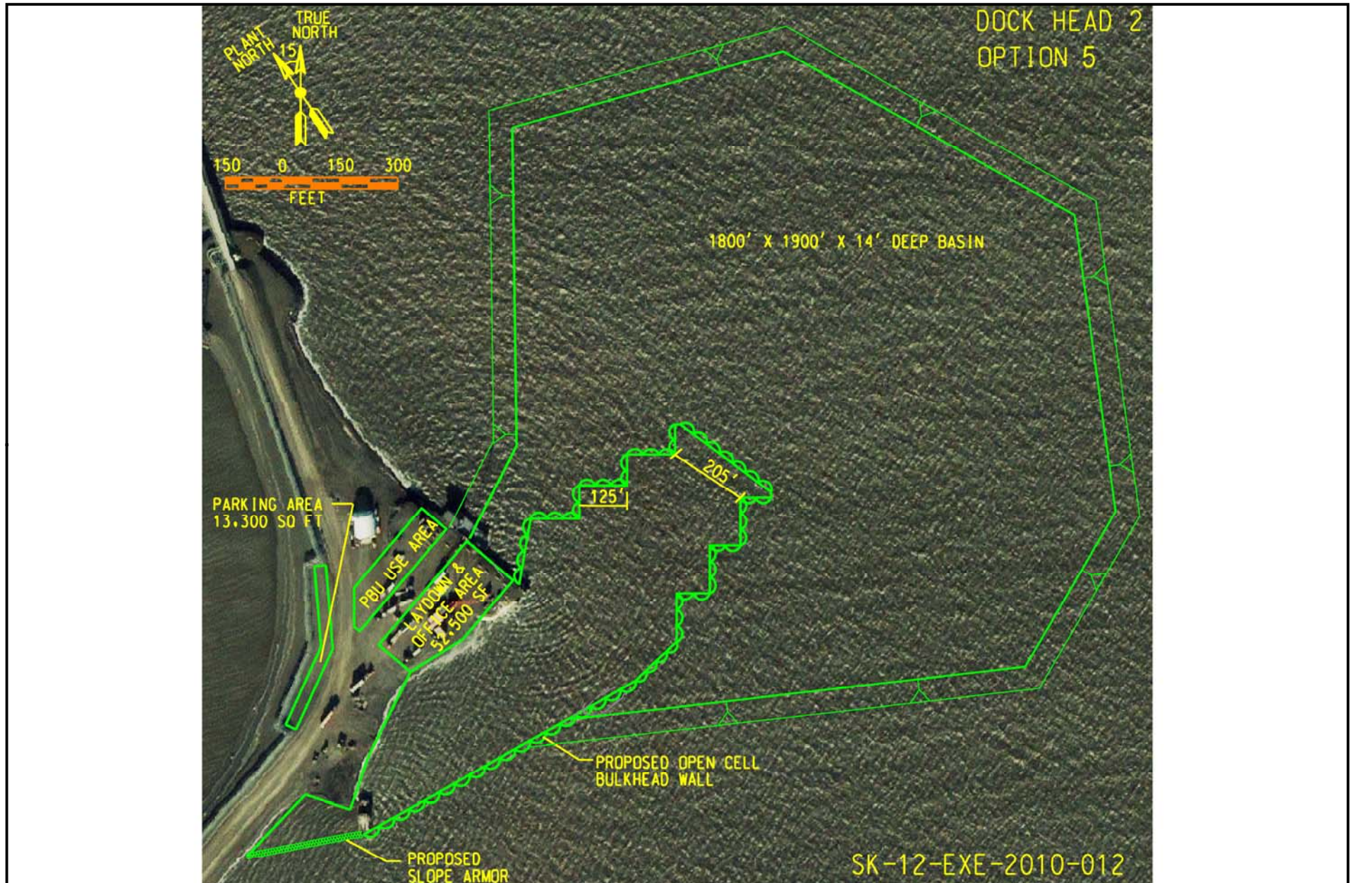
Appendix 10B Alaska Pipeline Project Dock Configuration 5
