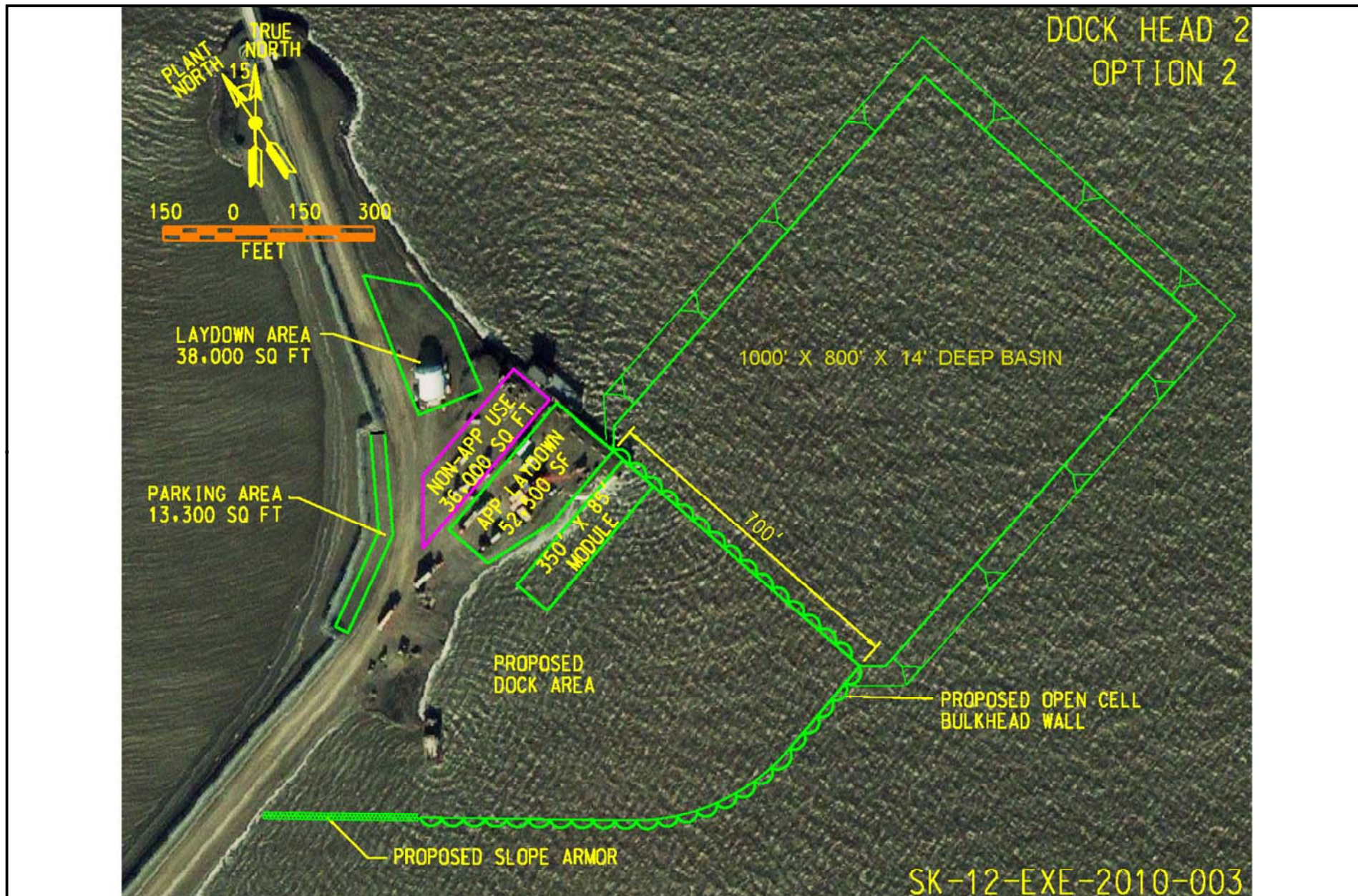
Appendix 10B Alaska Pipeline Project Dock Configuration 2
