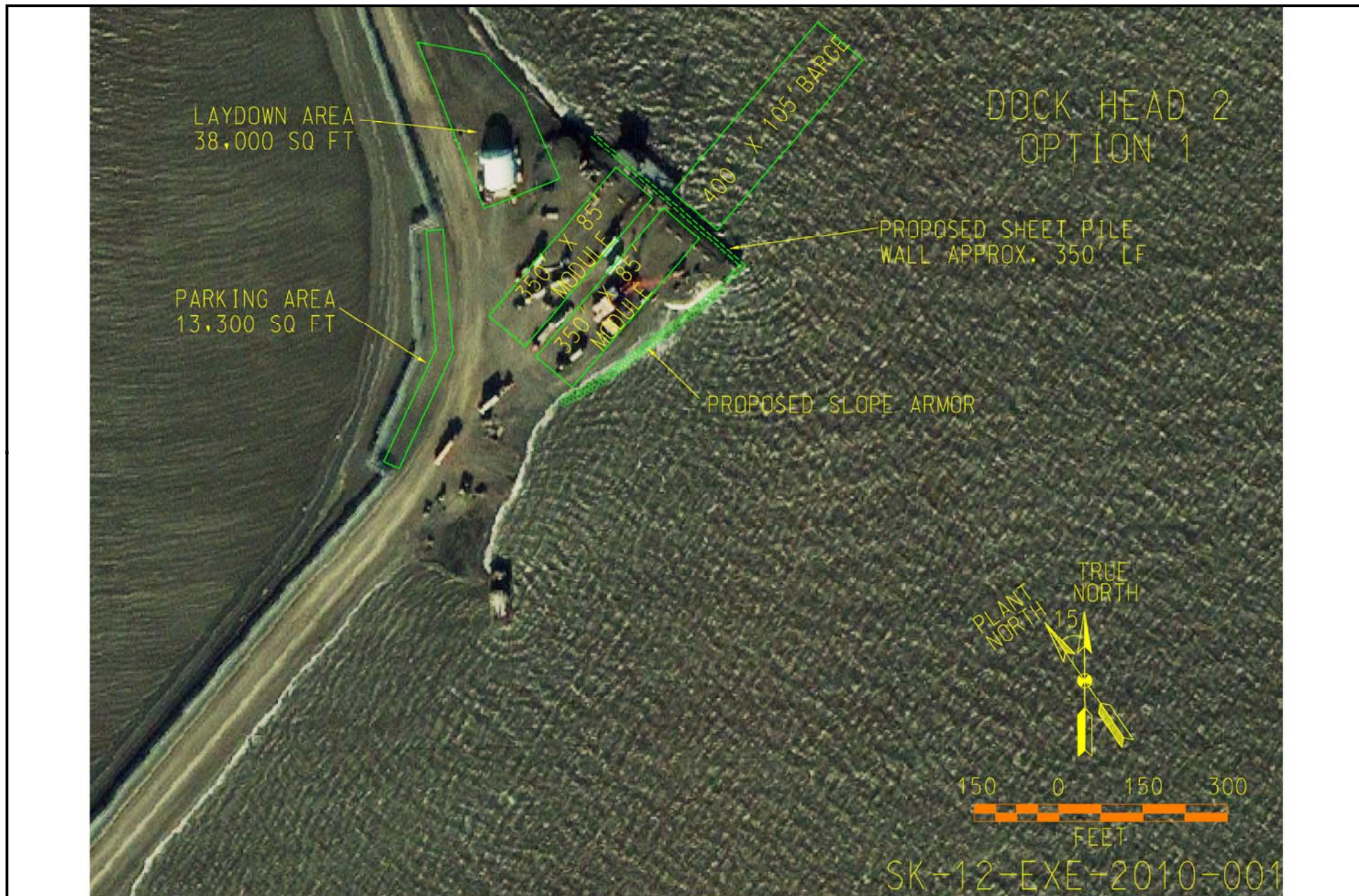
Appendix 10B Alaska Pipeline Project Dock Configuration 1
