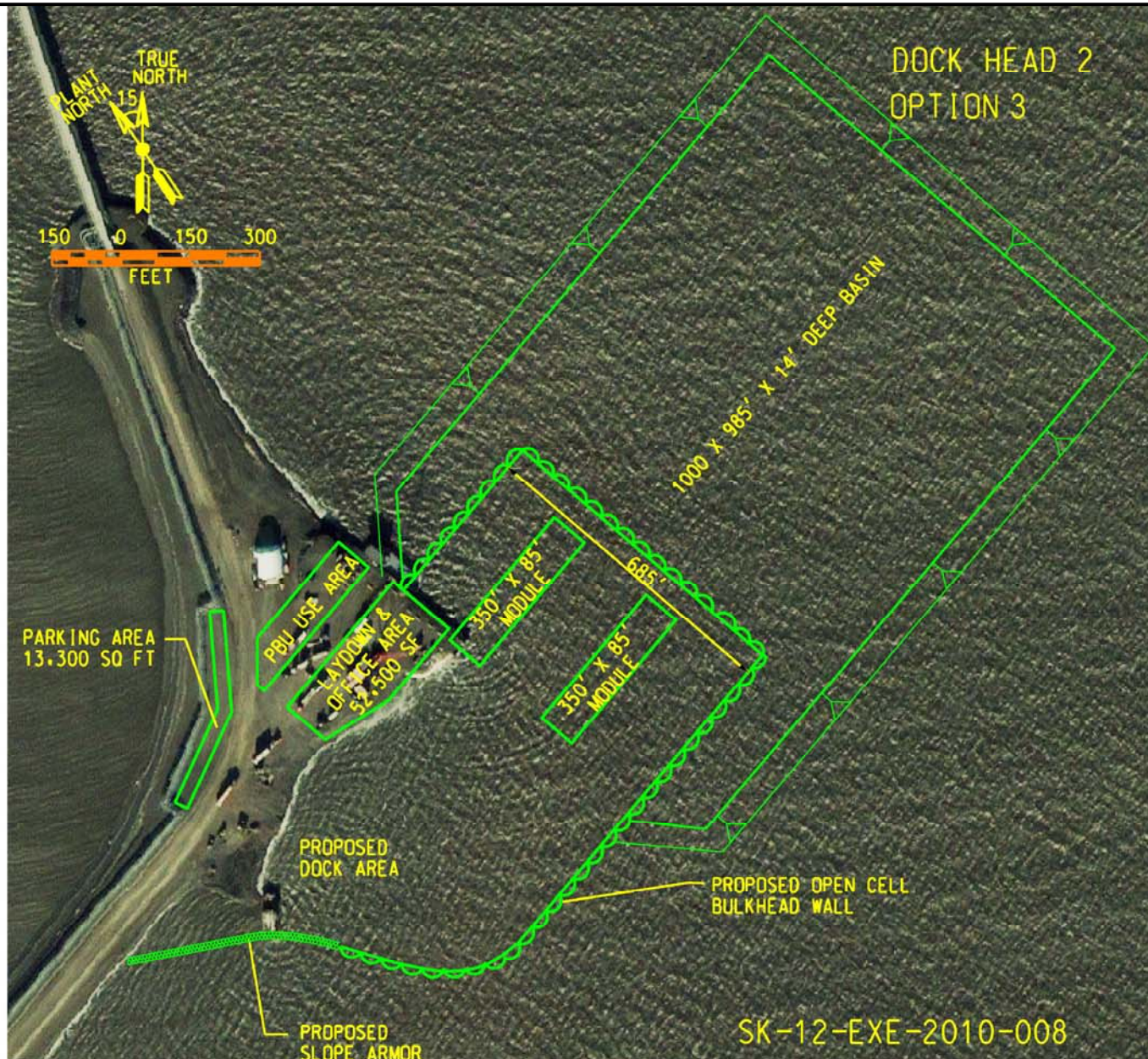
Appendix 10B Alaska Pipeline Project Dock Configuration 3
