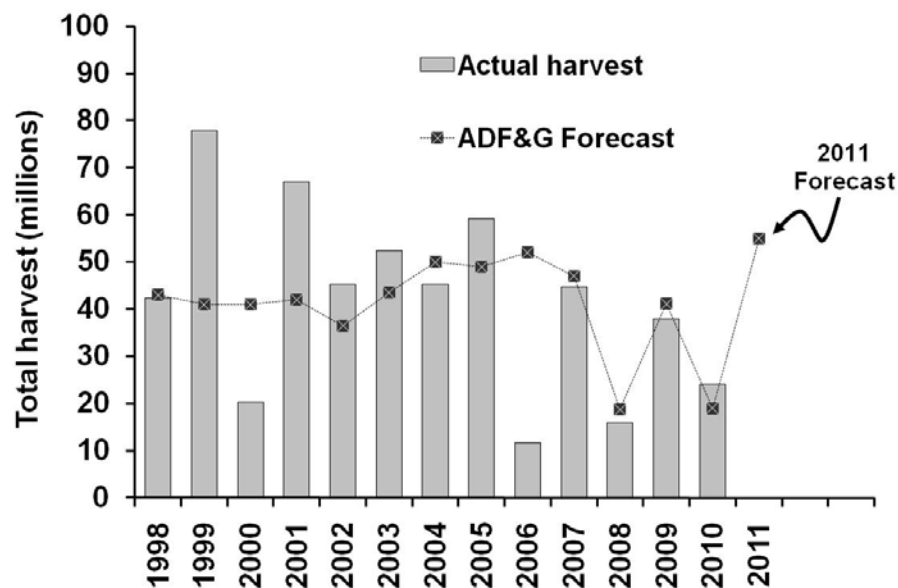
Figure A4.—Annual harvest of pink salmon in Southeast Alaska compared to the ADF&G preseason harvest forecast, 1998–2010. The 2007–2010 ADF&G harvest forecasts were adjusted using NOAA's juvenile pink salmon data.
