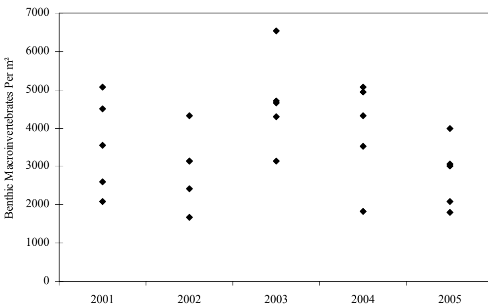
Figure 13. Density of benthic macroinvertebrates (n = 5 samples each year) at Greens Creek Below Pond D Site 54 in 2001 through 2005.
