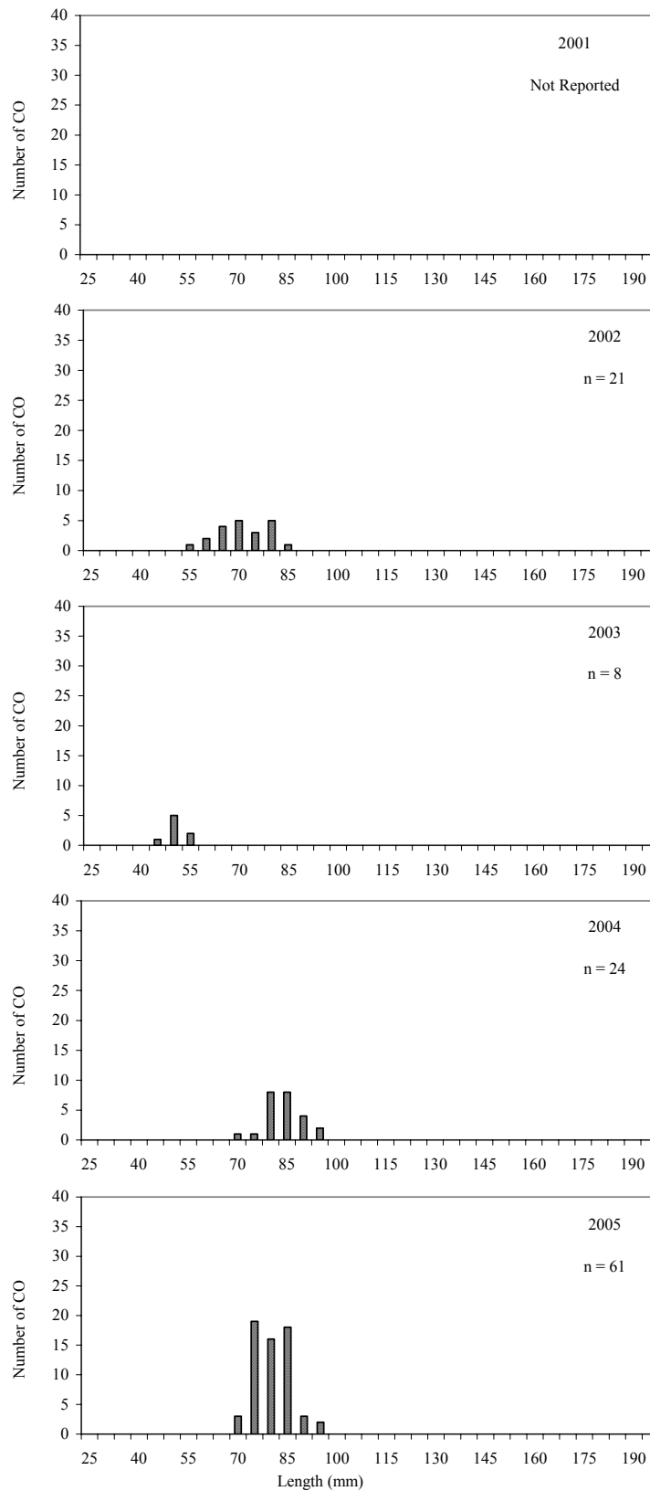
Figure 17. Length frequencies of juvenile coho salmon captured at Greens Creek Below Pond D Site 54 in 2001 through 2005.
