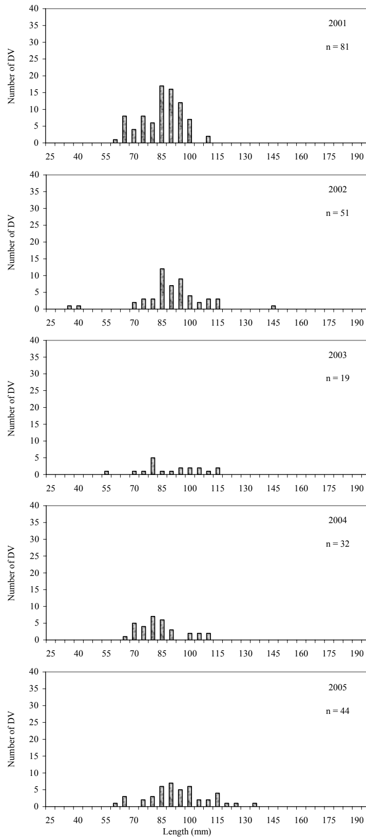
Figure 25. Length frequencies of Dolly Varden captured at Tributary Creek Site 9 in 2001 through 2005.
