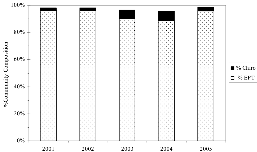
Figure 14. Proportions of EPT taxa and Chironomidae in Greens Creek Below Pond D Site 54 samples in 2001 through 2005.
