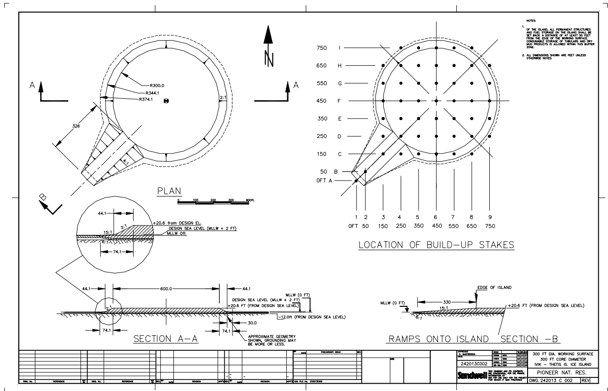
Figure 3-2b Geometry of Ivik Ice Island
