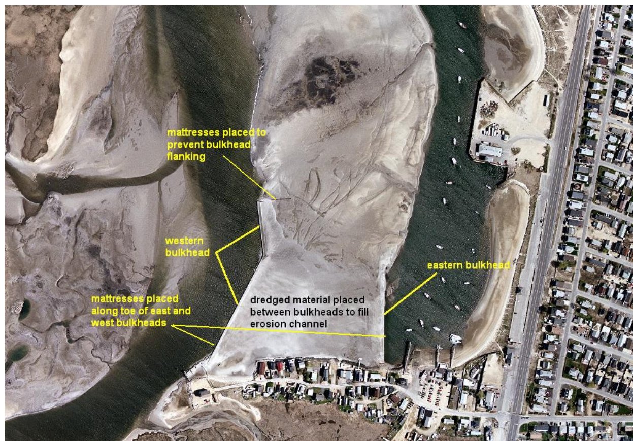
Figure 11. Aerial view of mattress placement at Seabrook, NH, Section 227 project (image provided by Kevin Knuuti, CHL)
