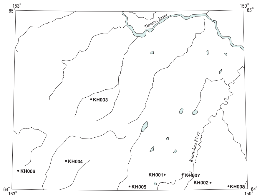
Distribution of mineral occurrences in the Kantishna River 1:250,000-scale quadrangle, Alaska
