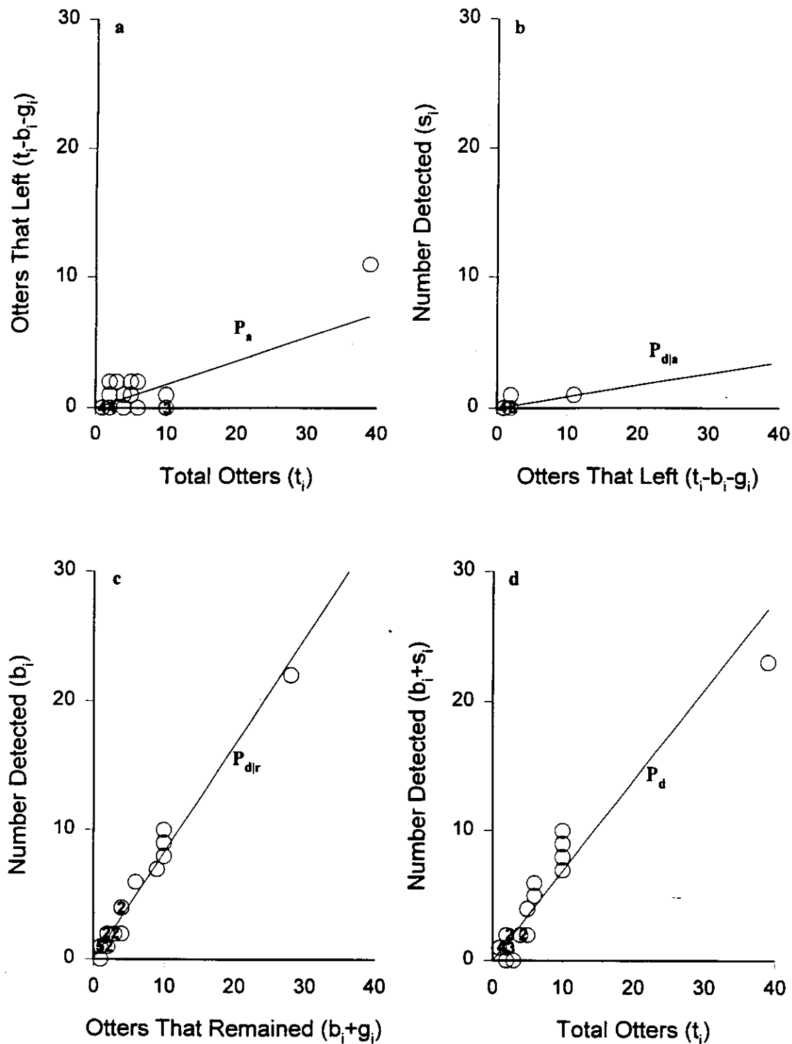
Figure 1. Scatter plots of the numbers of sea otters observed by ground crews, boat crews, or both on boat survey transect segments in Prince William Sound, Alaska. Numbers in circles indicate the number of segments represented by the circle. Circles without numbers represent one segment. Lines represent the overall ratio estimates of the probabilities.
